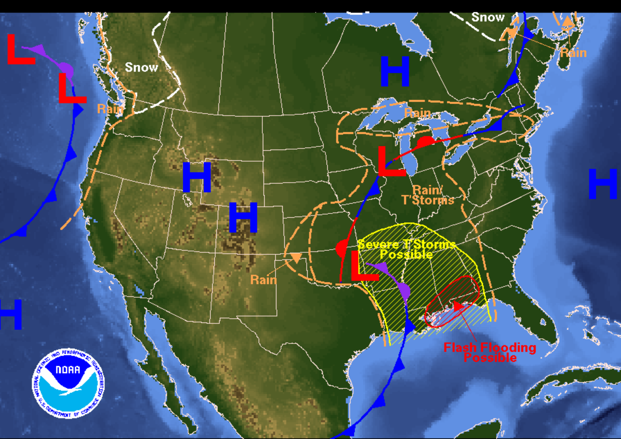
Weather Forecast for Wednesday, April 06, 2005 DOC/NOAA/NWS/NCEP/Hydrometeorological Prediction Center Prepared by Fries/Terry based on HPC, SPC, and TPC forecasts.
