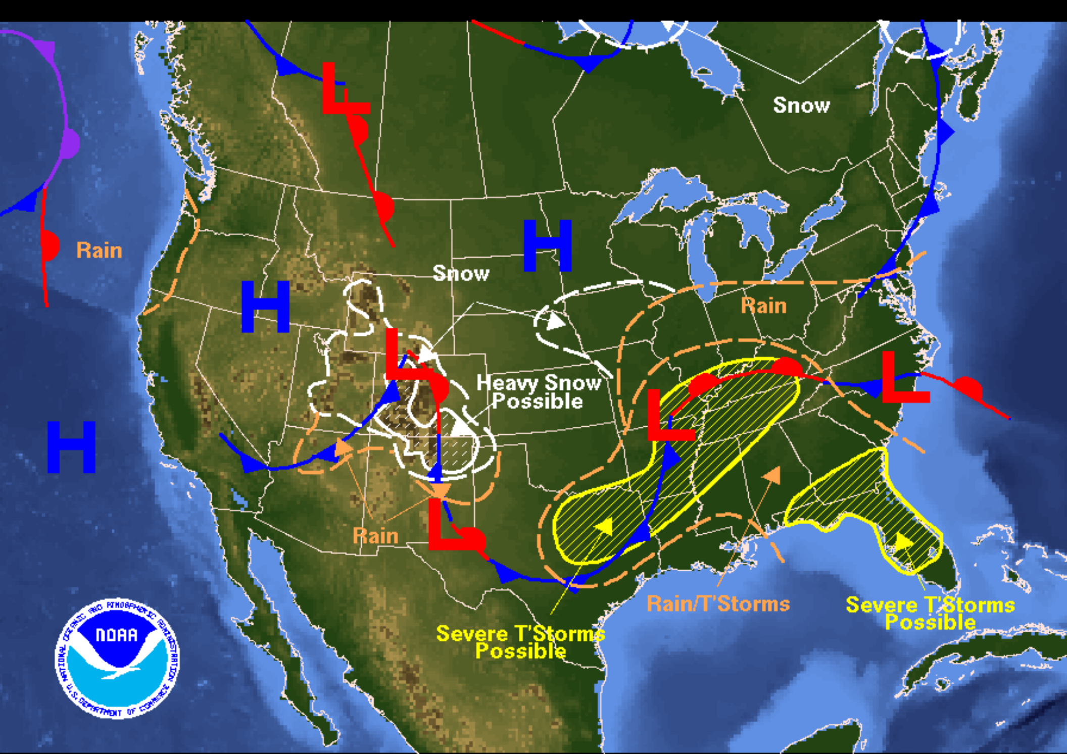
Weather Forecast for Friday, March 25, 2005 DOC/NOAA/NWS/NCEP/Hydrometeorological Prediction Center Prepared by Szataneck/Eckert based on HPC, SPC, and TPC forecasts.
