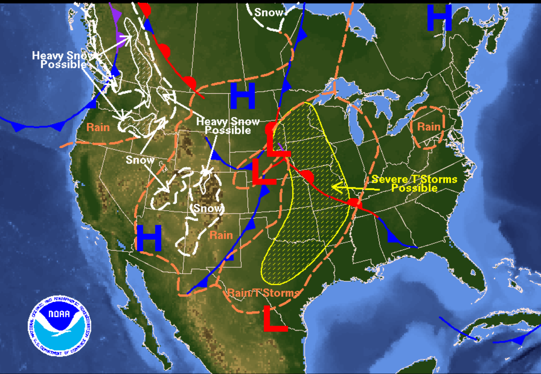
Weather Forecast for Friday, October 22, 2004 DOC/NOAA/NWS/NCEP/Hydrometeorological Prediction Center Prepared by Halbach/Oravec based on HPC, SPC, and TPC forecasts.
