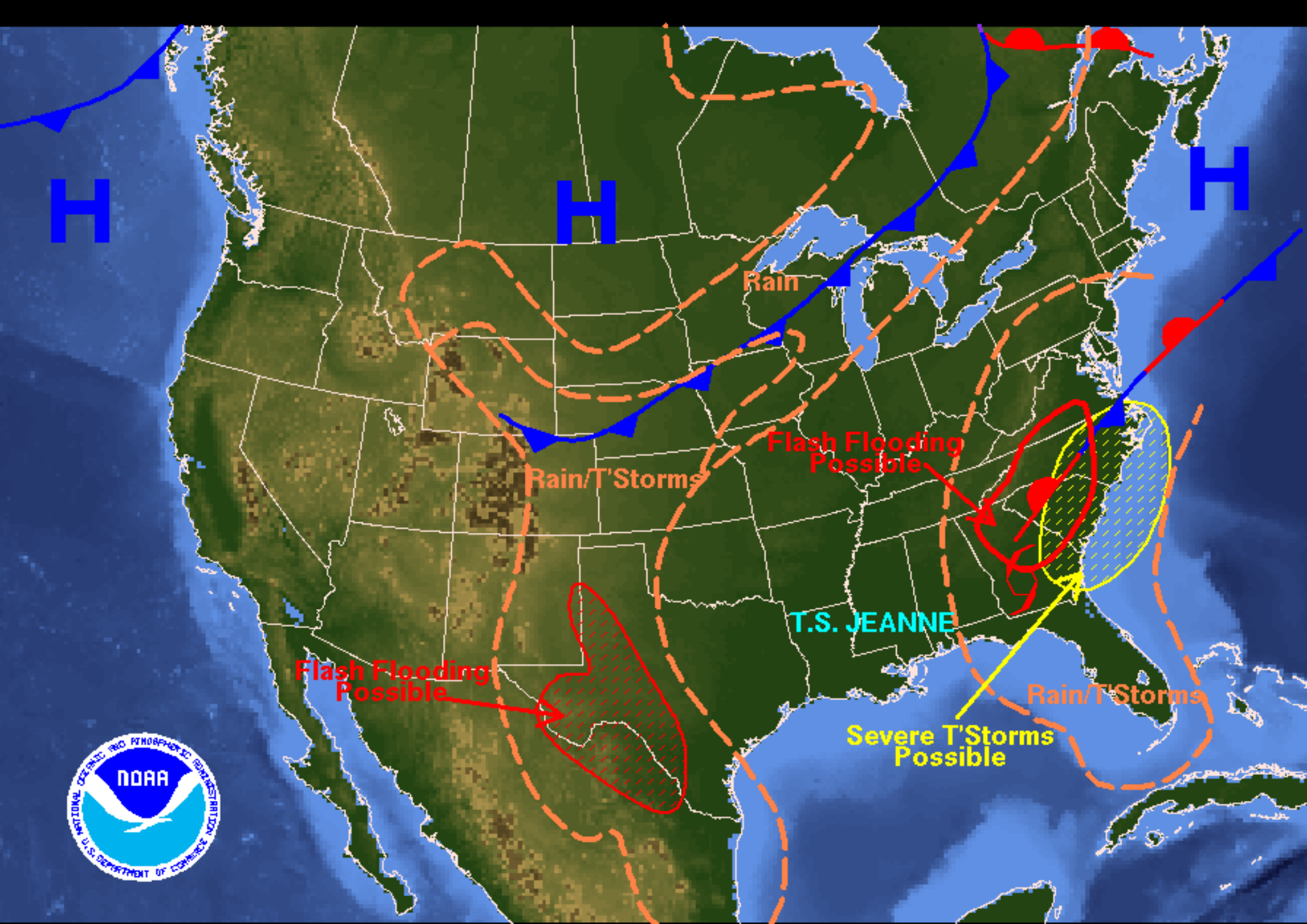
Weather Forecast for Monday, September 27, 2004 DOC/NOAA/NWS/NCEP/Hydrometeorological Prediction Center Prepared by Halbach/Oravec based on HPC, SPC, and TPC forecasts.
