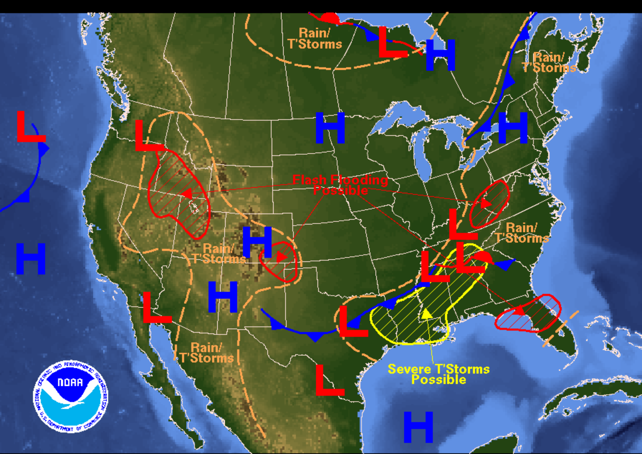
Weather Forecast for Saturday, July 17, 2004 DOC/NOAA/NWS/NCEP/Hydrometeorological Prediction Center Prepared by SzataneK/Oravec based on HPC, SPC, and TPC forecasts.
