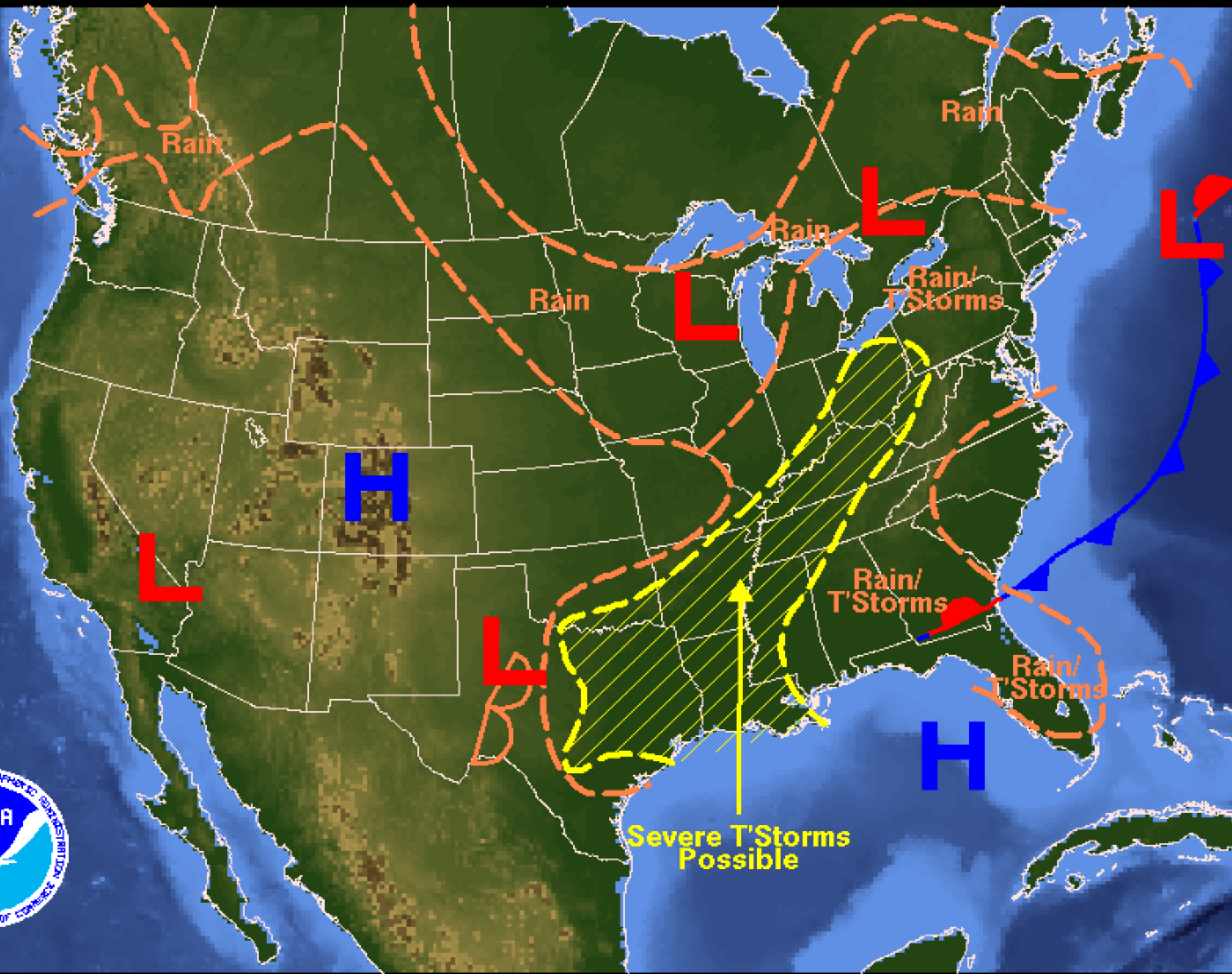
Weather Forecast for Tuesday, June 01, 2004 DOC/NOAA/NWS/NCEP/Hydrometeorological Prediction Center Prepared by Kosier/Korty based on HPC, SPC, and TPC forecasts.
