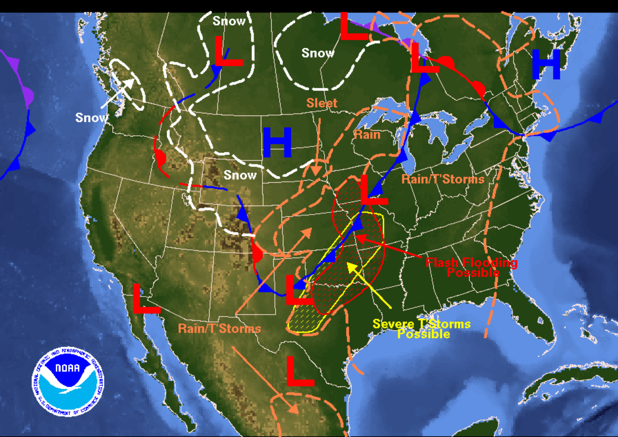
Weather Forecast for Thursday, May 13, 2004 DOC/NOAA/NWS/NCEP/Hydrometeorological Prediction Center Prepared by Bell/Eckert based on HPC, SPC, and TPC forecasts.
