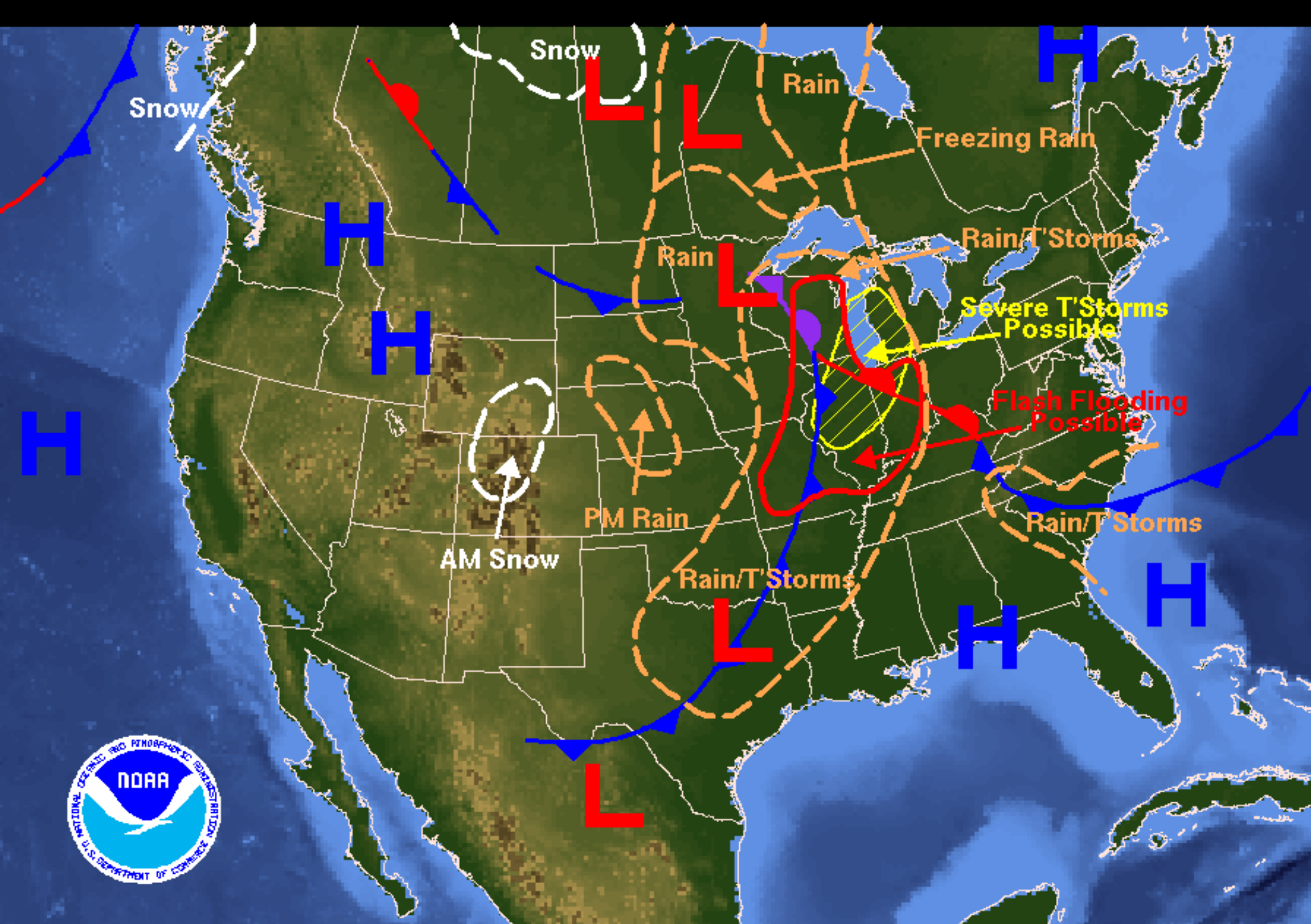
Weather Forecast for Sunday, March 28, 2004 DOC/NOAA/NWS/NCEP/Hydrometeorological Prediction Center Prepared by Hatchett/Clark based on HPC, SPC, and TPC forecasts.
