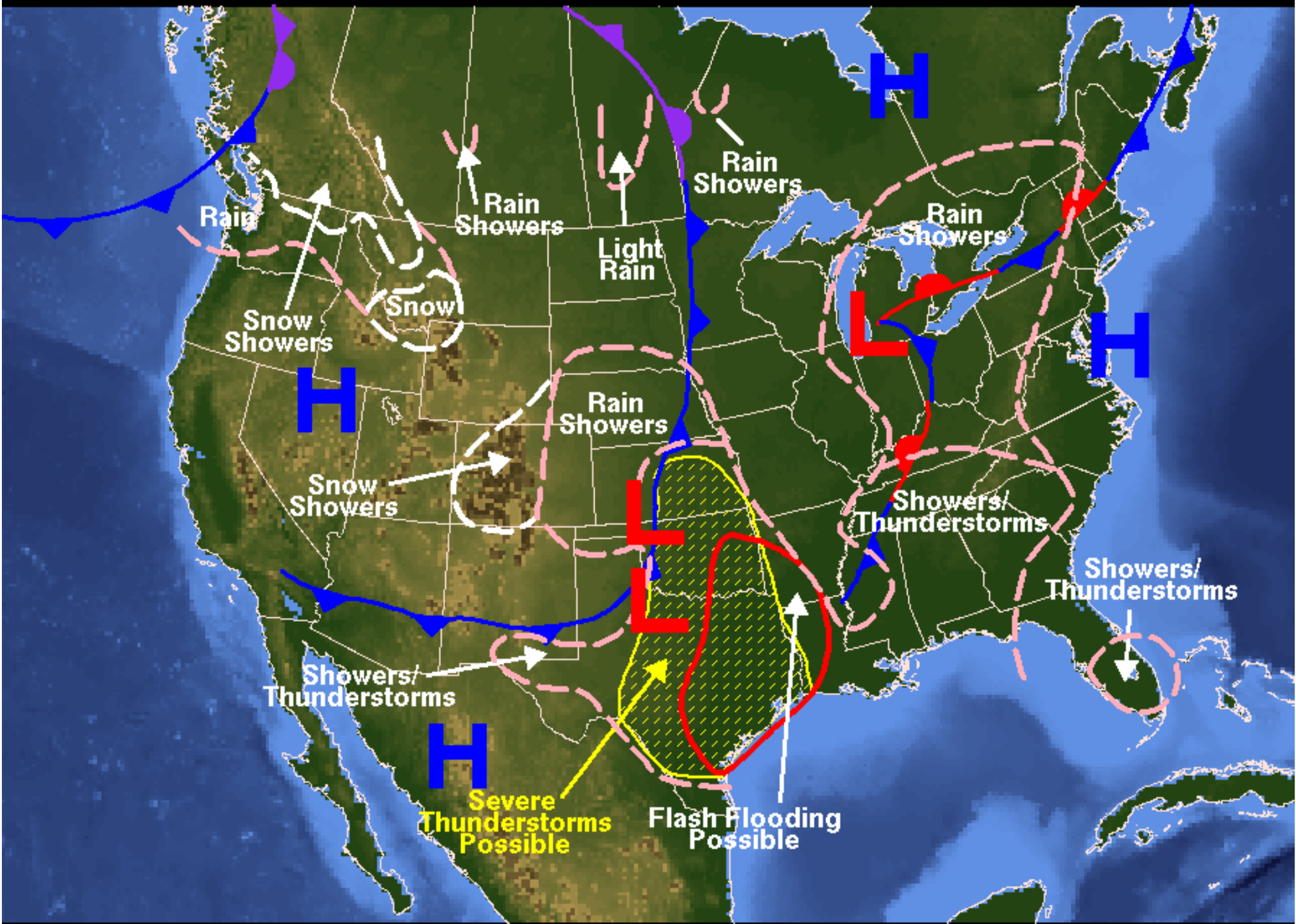
Weather Forecast for Friday, October 12, 2001 Prepared by HATCHETT/ECKERT
