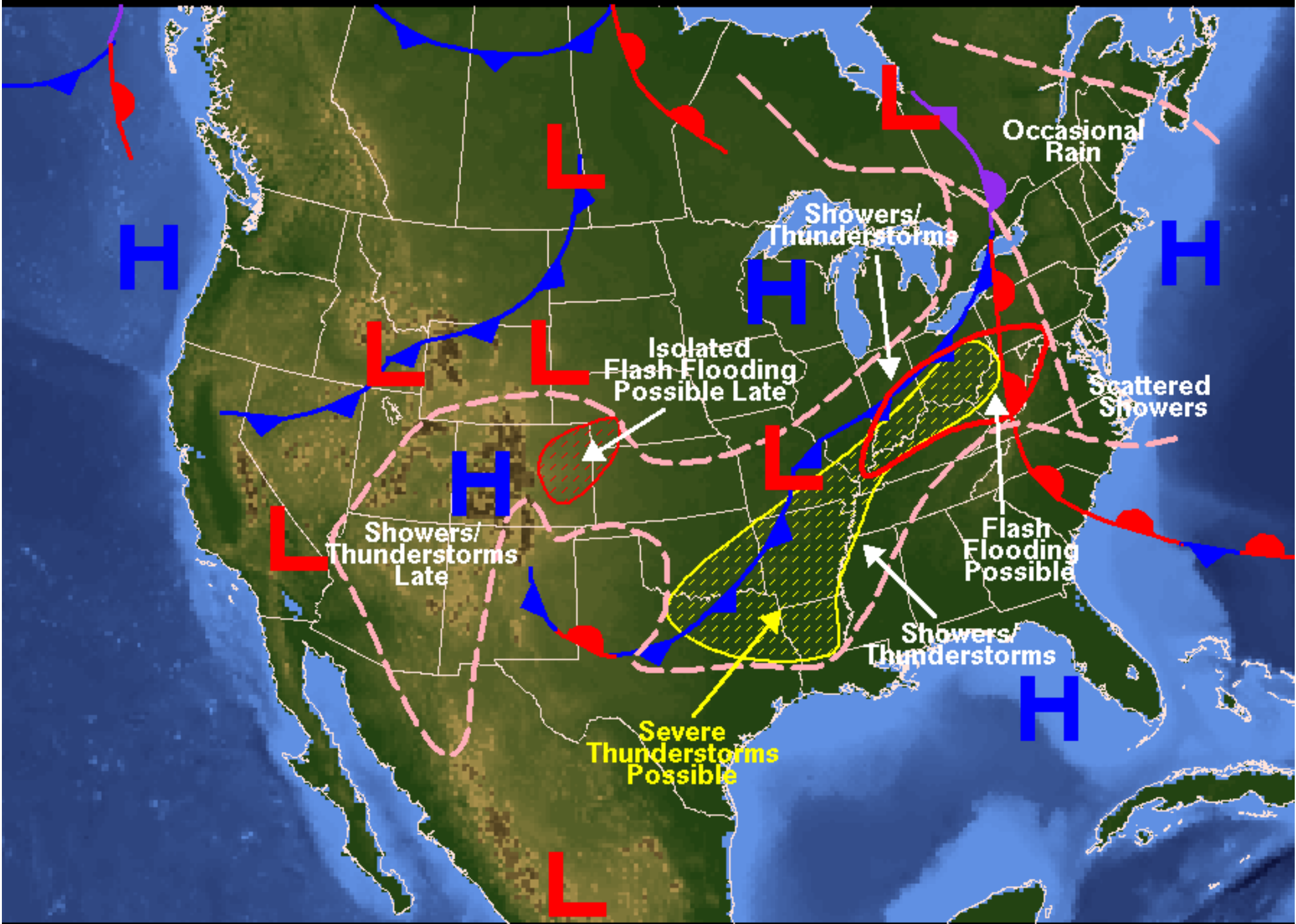
Weather Forecast for Friday, May 18, 2001 Prepared by RAUSCH/ECKERT DOC/NOAA/NWS/NCEP/Hydrometeorological Prediction Center
