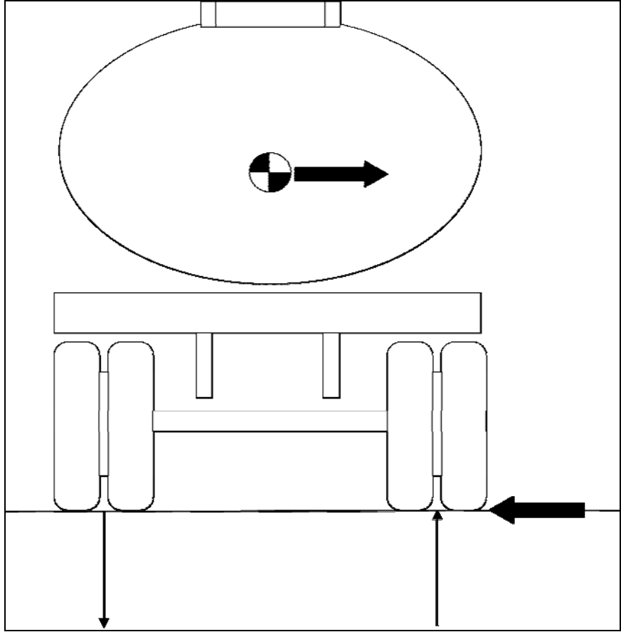
Figure 1 - 1 Roll Plane Forces Acting on a Tank Trailer
