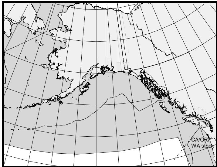
Figure 35. Approximate distribution of minke whales in the eastern North Pacific (shaded area).
