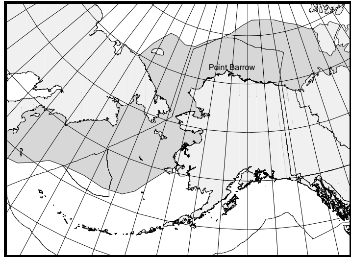
Figure 37. Approximate distribution of the Western Arctic stock of bowhead whales. The shaded area includes regions used during both the winter and summer by whales from this stock.
