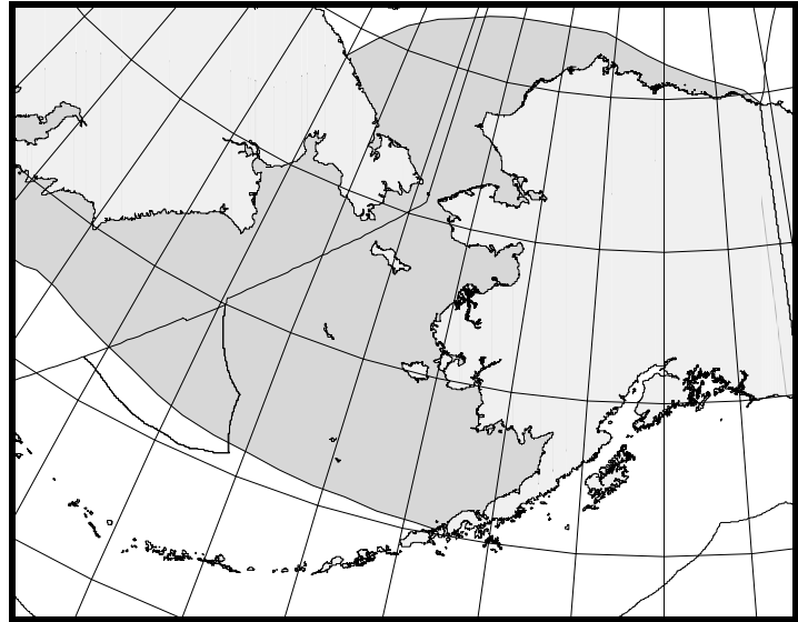
Figure 11. Approximate distribution of spotted seals in Alaska waters (shaded area).
