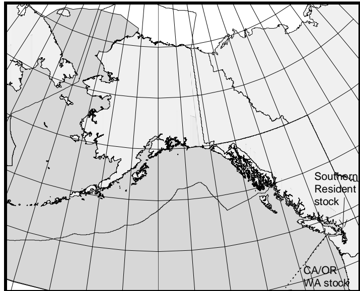
Figure 21. Approximate distribution of killer whales in the eastern North Pacific (shaded area). The distribution of the Eastern North Pacific Northern Resident and Transient stocks are largely overlapping (see text).
