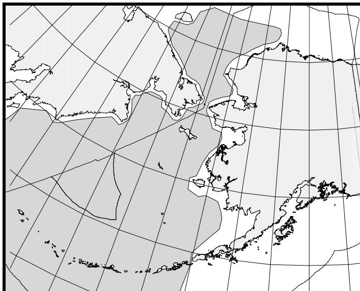
Figure 14. Approximate distribution of ribbon seals in Alaska waters (shaded area). The combined summer and winter distribution is depicted.
