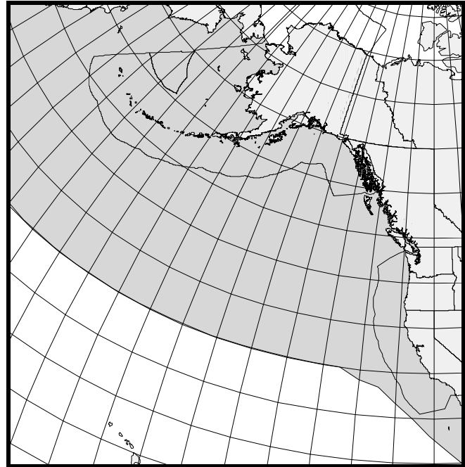
Figure 36. Approximate historical distribution of right whales in the eastern North Pacific (shaded area).
