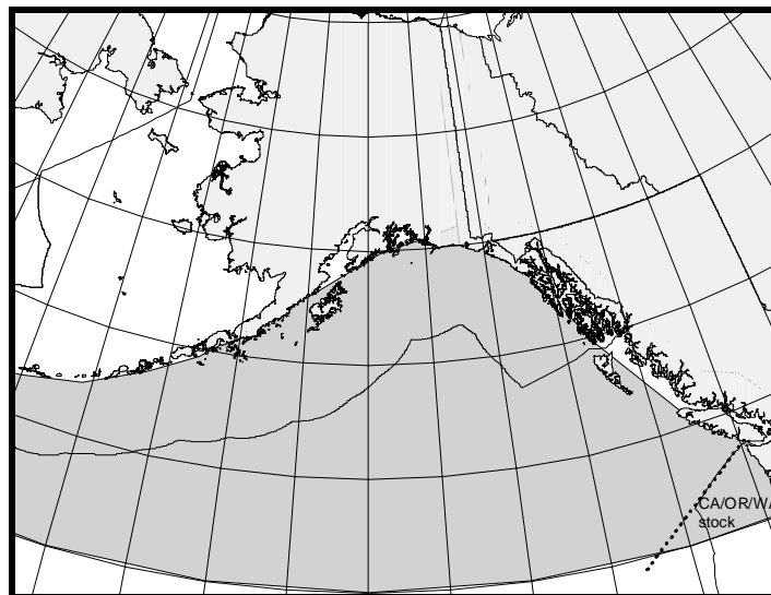
Figure 29. Approximate distribution of Cuvier's beaked whales in the eastern North Pacific (shaded area).
