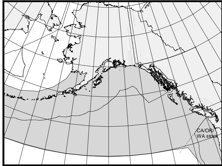
Figure 22. Approximate distribution of Pacific white-sided dolphins in the eastern North Pacific (shaded area).
