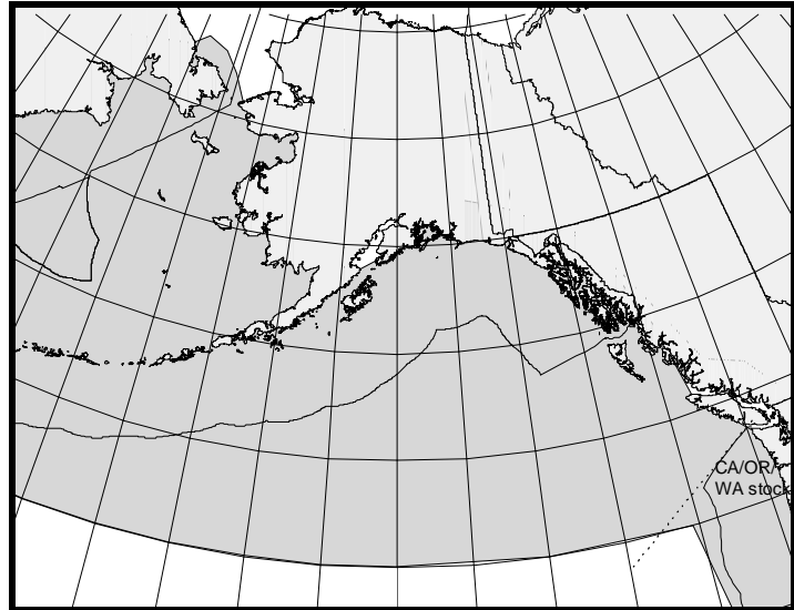
Figure 34. Approximate distribution of fin whales in the eastern North Pacific (shaded area).
