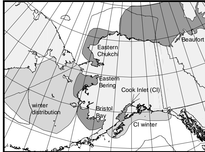
Figure 19. Approximate distribution of beluga whales in Alaska waters. The dark shading displays the summer distributions of the five stocks. Winter distributions are depicted with lighter shading.
