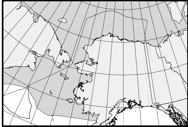
Figure 13. Approximate distribution of ringed seals in Alaska waters (shaded area). The combined summer and winter distribution is depicted.
