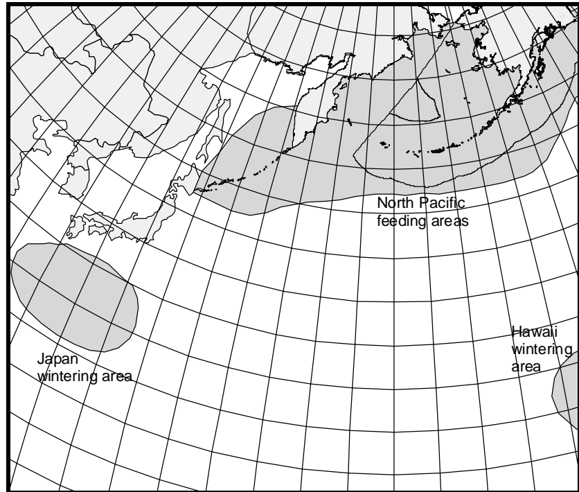
Figure 32. Approximate distribution of humpback whales in the western North Pacific (shaded area). Feeding and wintering areas are presented above (see text). See Figure 32 for humpback whale distribution in the eastern North Pacific.
