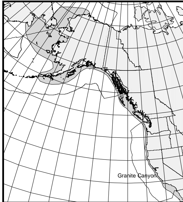
Figure 31. Approximate distribution of the Eastern North Pacific stock of gray whales (shaded area). Excluding some Mexican waters, the entire range of this stock is depicted in the figure.
