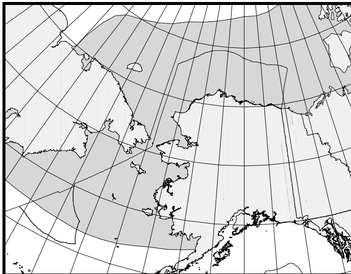
Figure 12. Approximate distribution of bearded seals in Alaska waters (shaded area). The combined summer and winter distributions are depicted.
