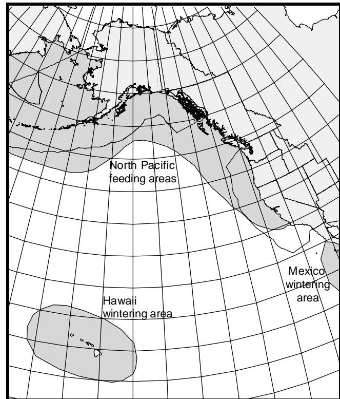
Figure 33. Approximate distribution of humpback whales in the eastern North Pacific (shaded area). Feeding and wintering areas are presented above (see text). See Figure 31 for distribution of humpback whales in the western North Pacific.
