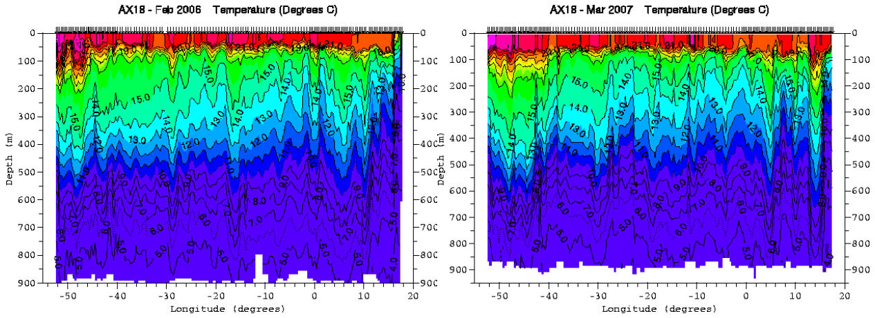
Figure 3. Temperature sections obtained from the February 2006 and March 2007 transects.
