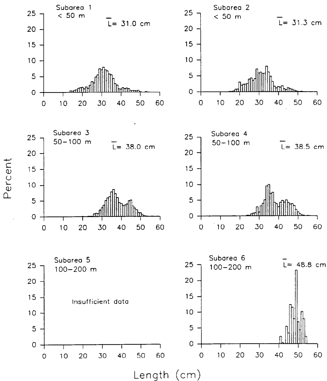
Figure 33. --Estimated relative size composition of Alaska plaice (sexes combined) by subarea, 1990 eastern Bering Sea bottom trawl survey.
