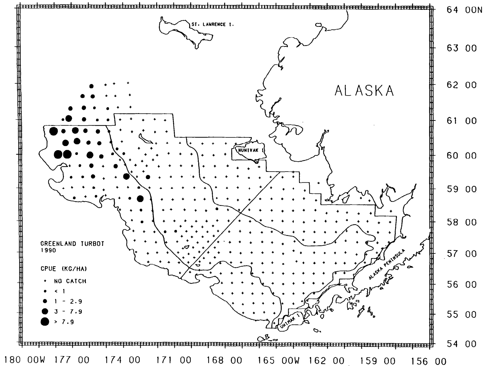
Figure 35. --Distribution and relative abundance in kg/ha of Greenland turbot, 1990 eastern Bering Sea bottom trawl survey.
