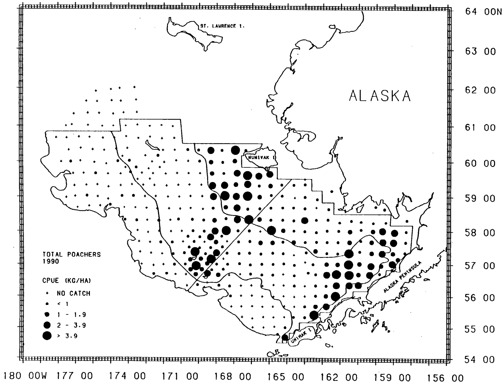
Figure 47.--Distribution and relative abundance in kg/ha of poachers, 1990 eastern Bering Sea bottom trawl survey.
