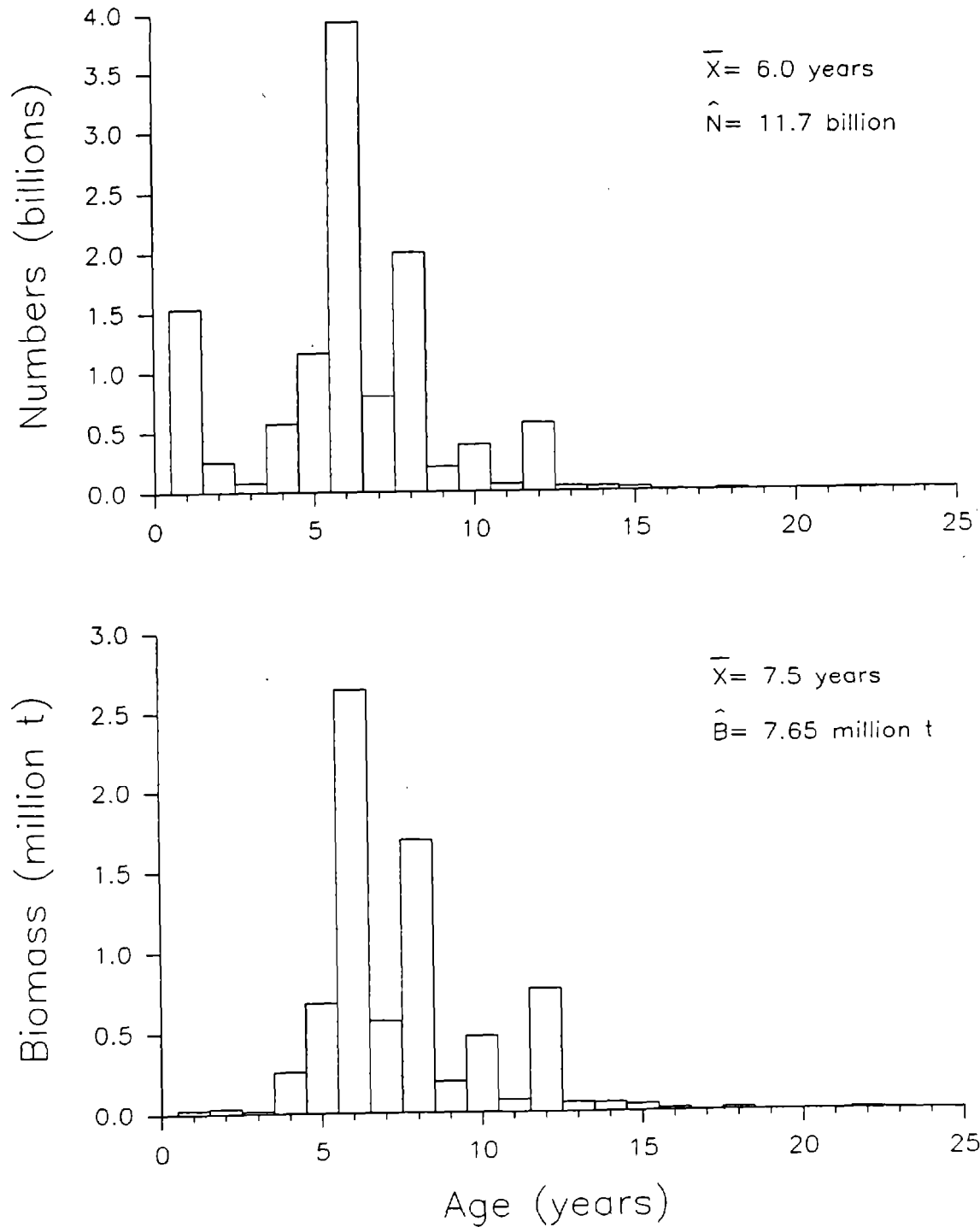
Figure 12. --Population number and biomass (metric tons) estimates by age for walleye pollock, 1990 eastern Bering Sea bottom trawl survey.
