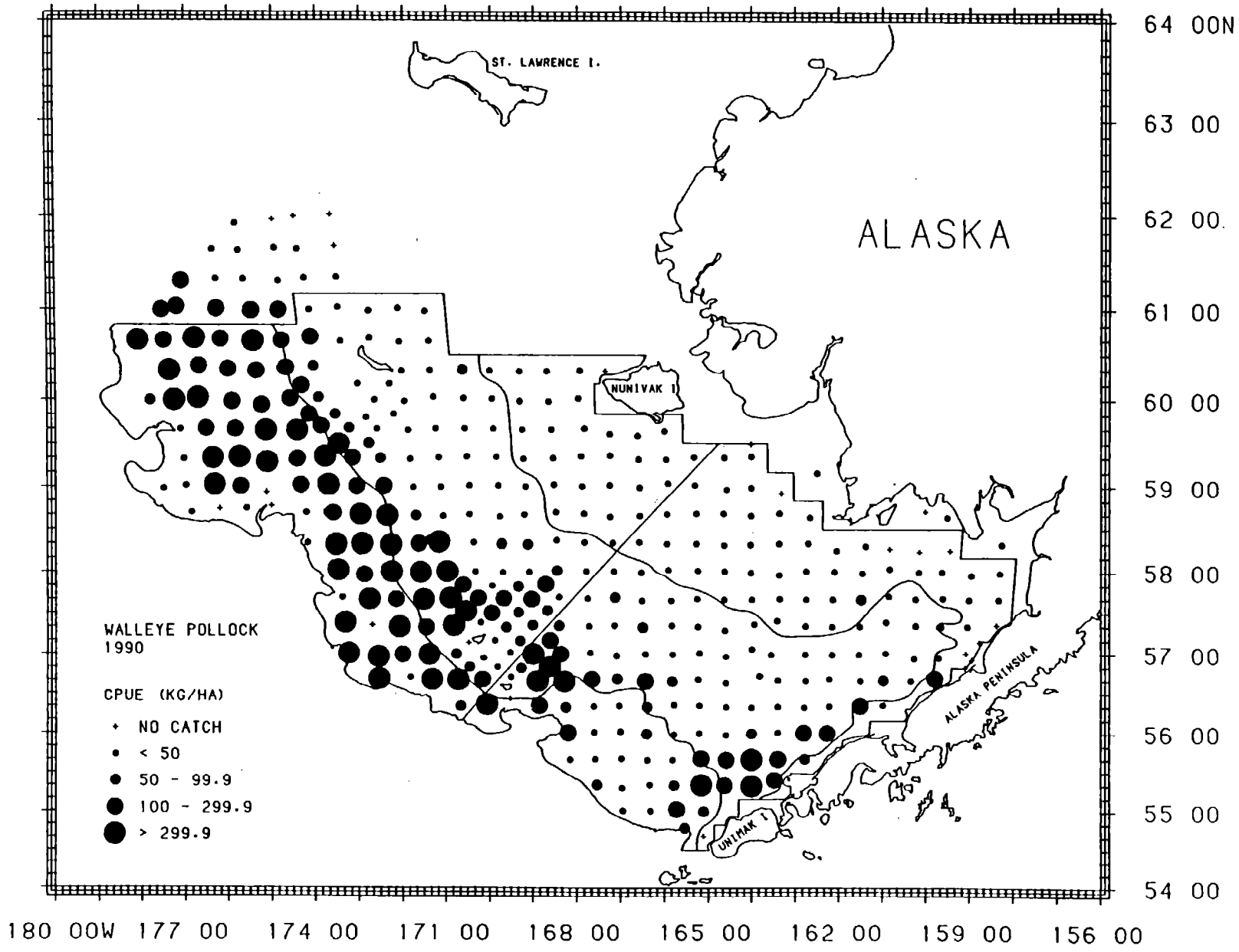
Figure 9. --Distribution and relative abundance in kg/ha of walleye pollock, 1990 eastern Bering Sea bottom trawl survey.
