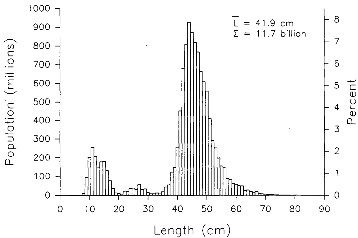
Figure 11. --Estimated size composition of walleye pollock (sexes combined), all subareas combined, 1990 eastern Bering Sea bottom trawl survey.
