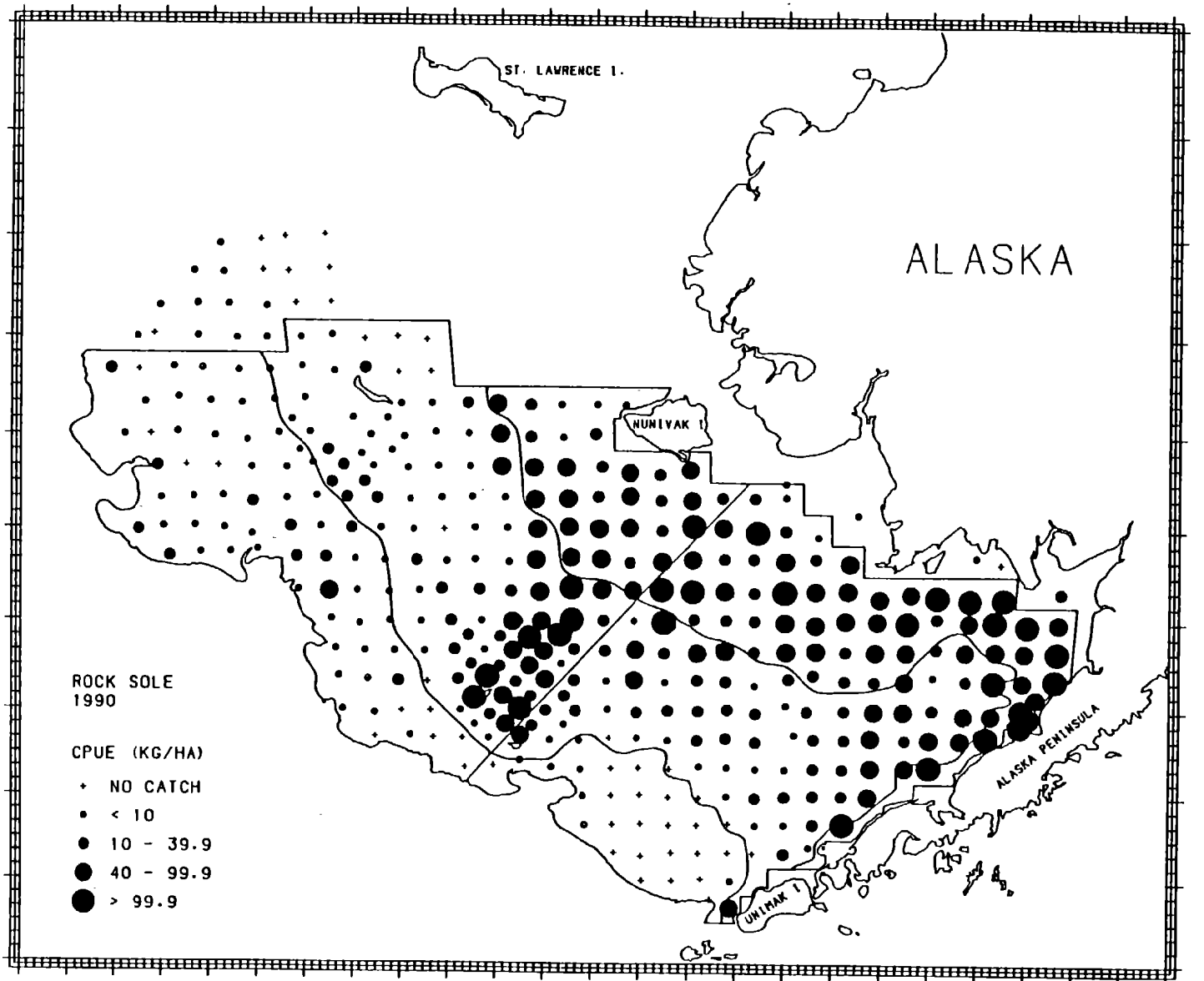
Figure 24.--Distribution and relative abundance in kg/ha of rock sole, 1990 eastern Bering Sea bottom trawl survey.
