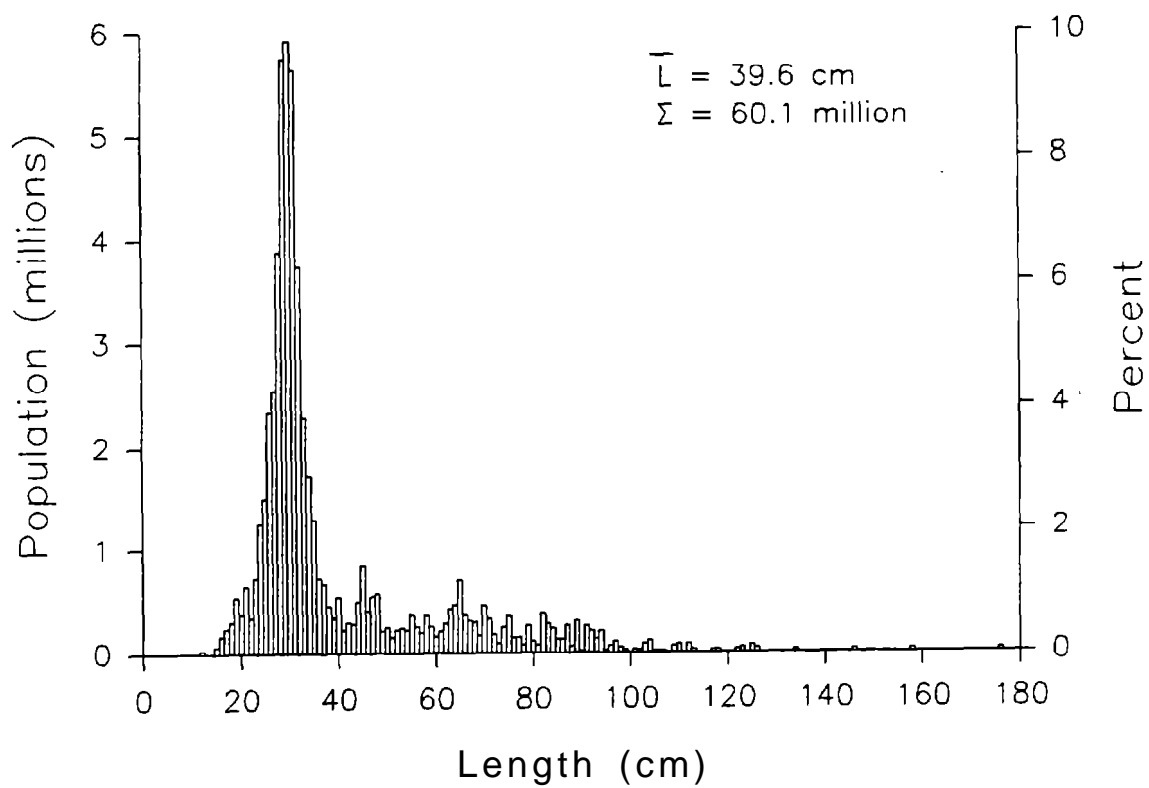
Figure 43. --Estimated size composition of Pacific halibut (sexes combined), all subareas combined, 1990 eastern Bering Sea bottom trawl survey.
