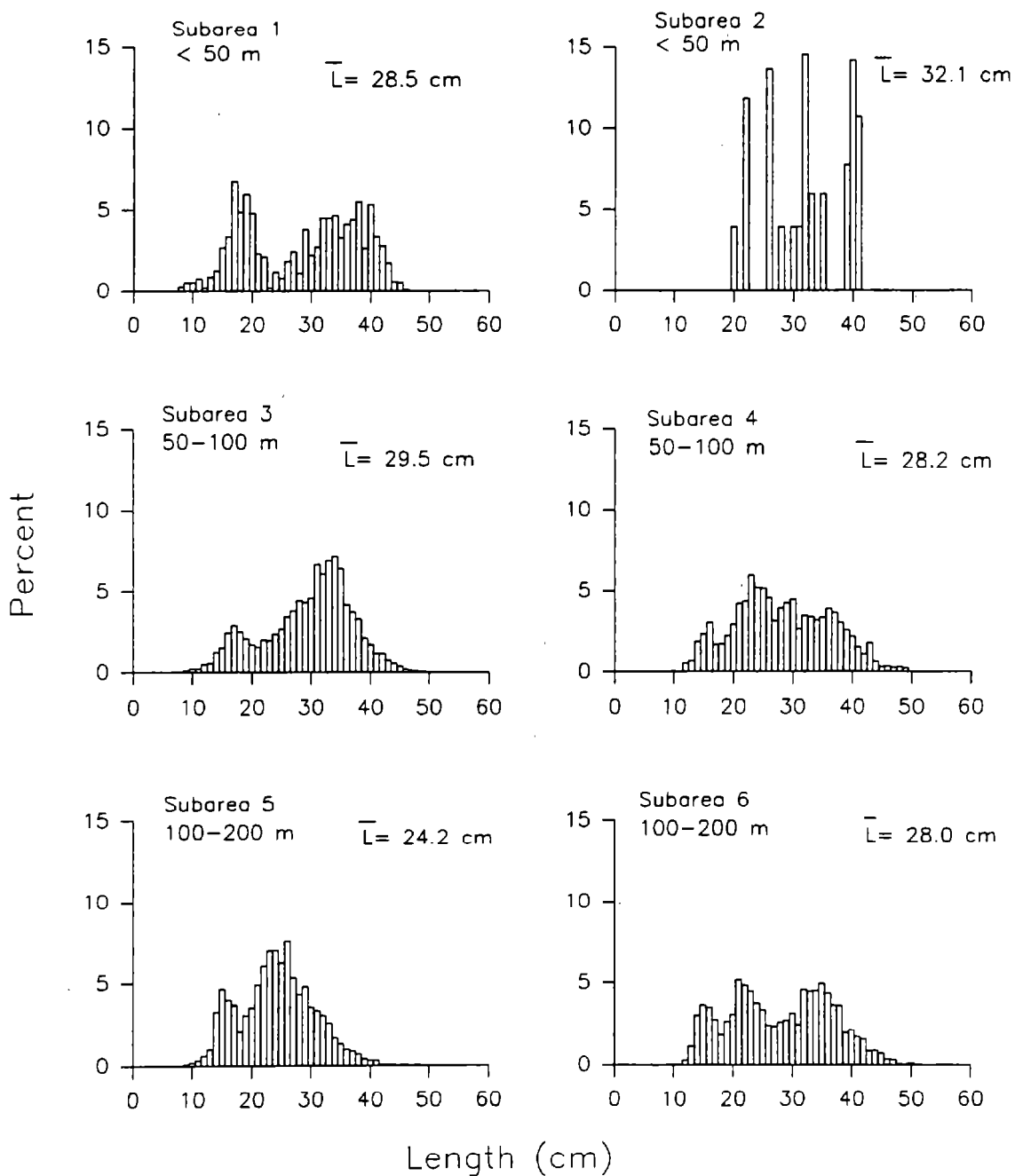
Figure 30. --Estimated relative size composition of Hippoglossoides Spp. (sexes combined) by subarea, 1990 eastern Bering Sea bottom trawl survey.
