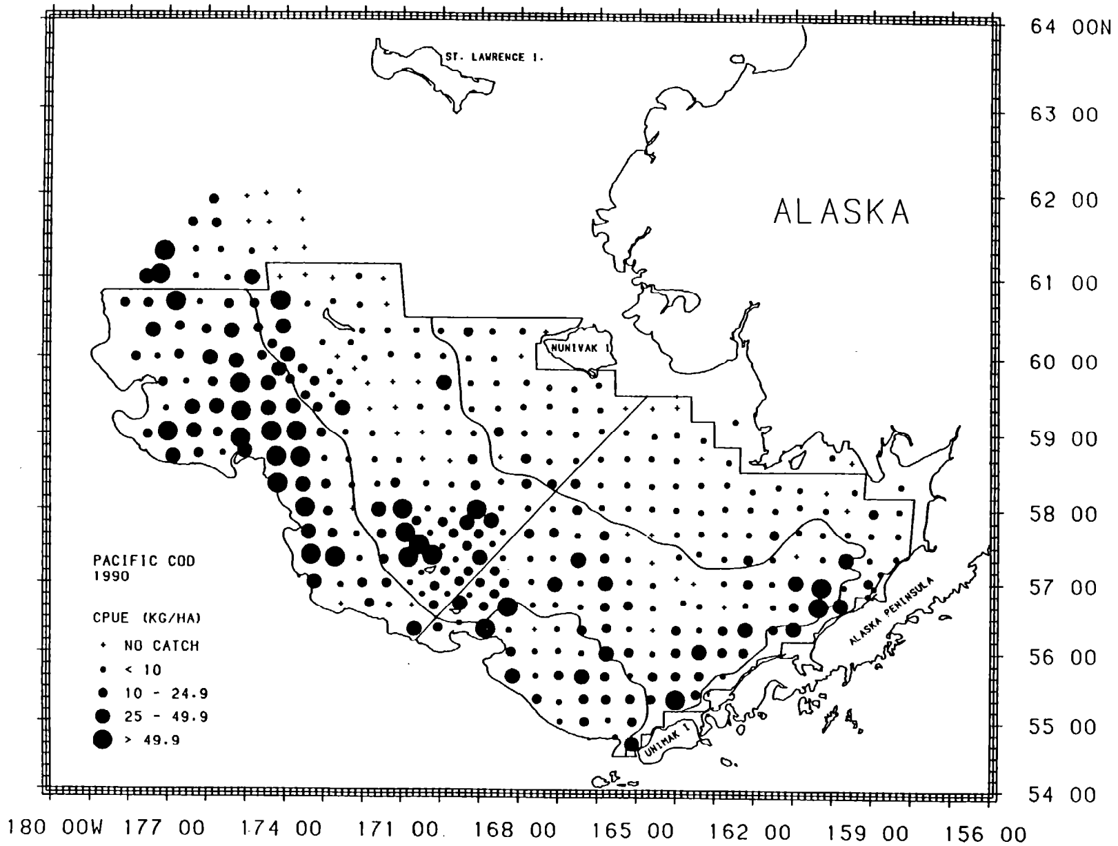
Figure 14. --Distribution and relative abundance in kg/ha of Pacific cod, 1990 eastern Bering Sea bottom trawl survey.
