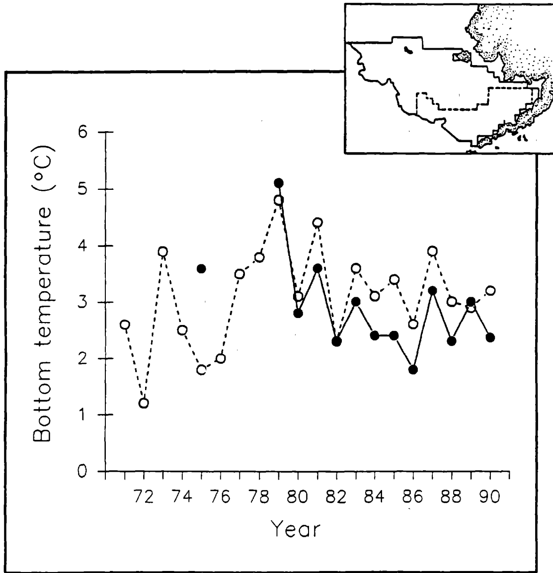
Figure 6. --Mean summer bottom water temperatures based on bathythermograph casts made during Alaska Fisheries Science Center bottom trawl surveys. The 1971-90 means (dashed line) are from the southeast Bering Sea (see inset) and the 1975 and 1979-90 means are from the larger survey area outlined on the inset. The 1975 data point for the overall survey area is based on data collected from August through September, while those in all other years and areas were collected from June through early August.
