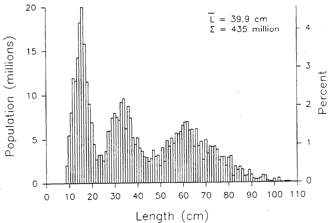
Figure 16. --Estimated size composition of Pacific cod (sexes combined), all subareas combined, 1990 eastern Bering Sea bottom trawl survey.
