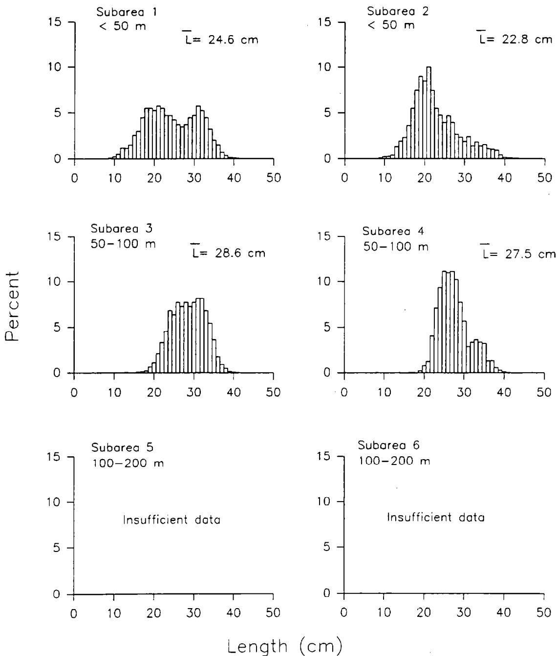
Figure 20. --Estimated relative size composition of yellowfin sole (sexes combined) by subarea, 1990 eastern Bering Sea bottom trawl survey.
