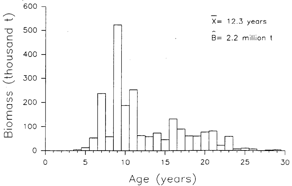
Figure 22. --Population number and biomass (metric tons) estimates by age for yellowfin sole, 1990 eastern Bering Sea bottom trawl survey.
