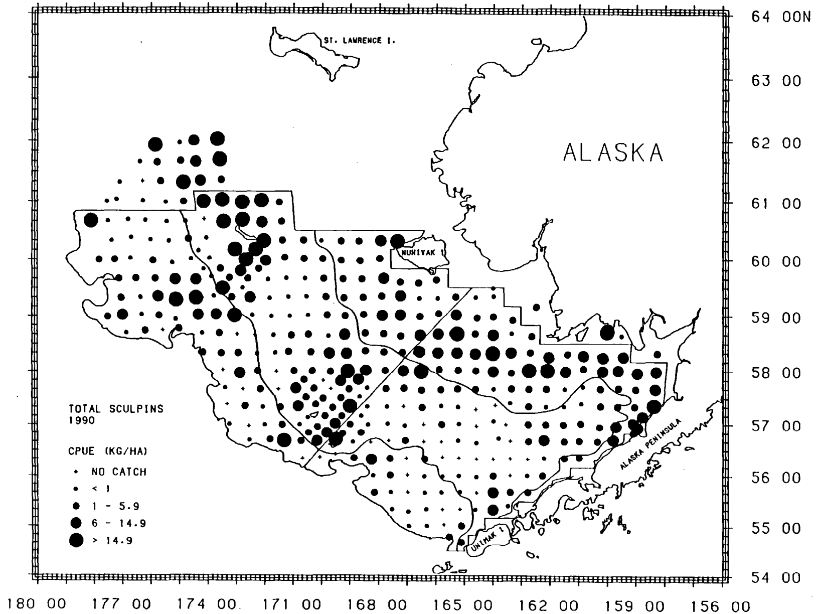
Figure 45.--Distribution and relative abundance in kg/ha of sculpins, 1990 eastern Bering Sea bottom trawl survey.
