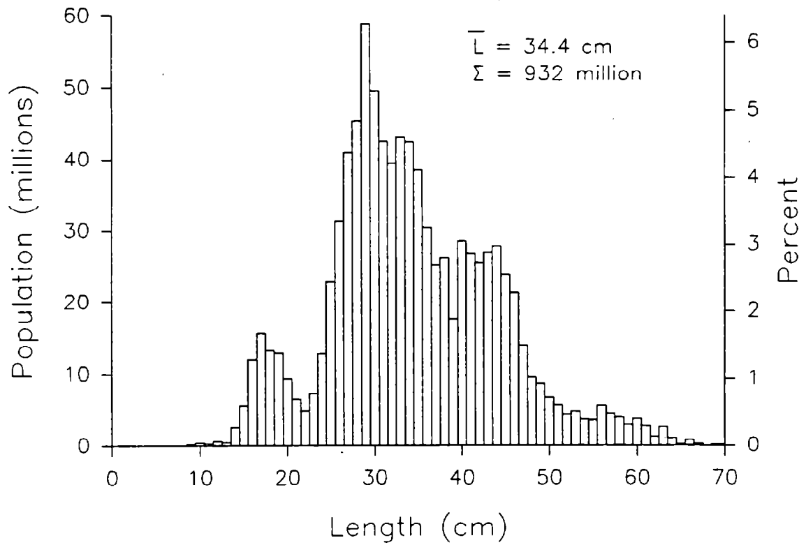
Figure 40. --Estimated size composition of Atheresthes spp. (sexes combined), all subareas combined, 1990 eastern Bering Sea bottom trawl survey.
