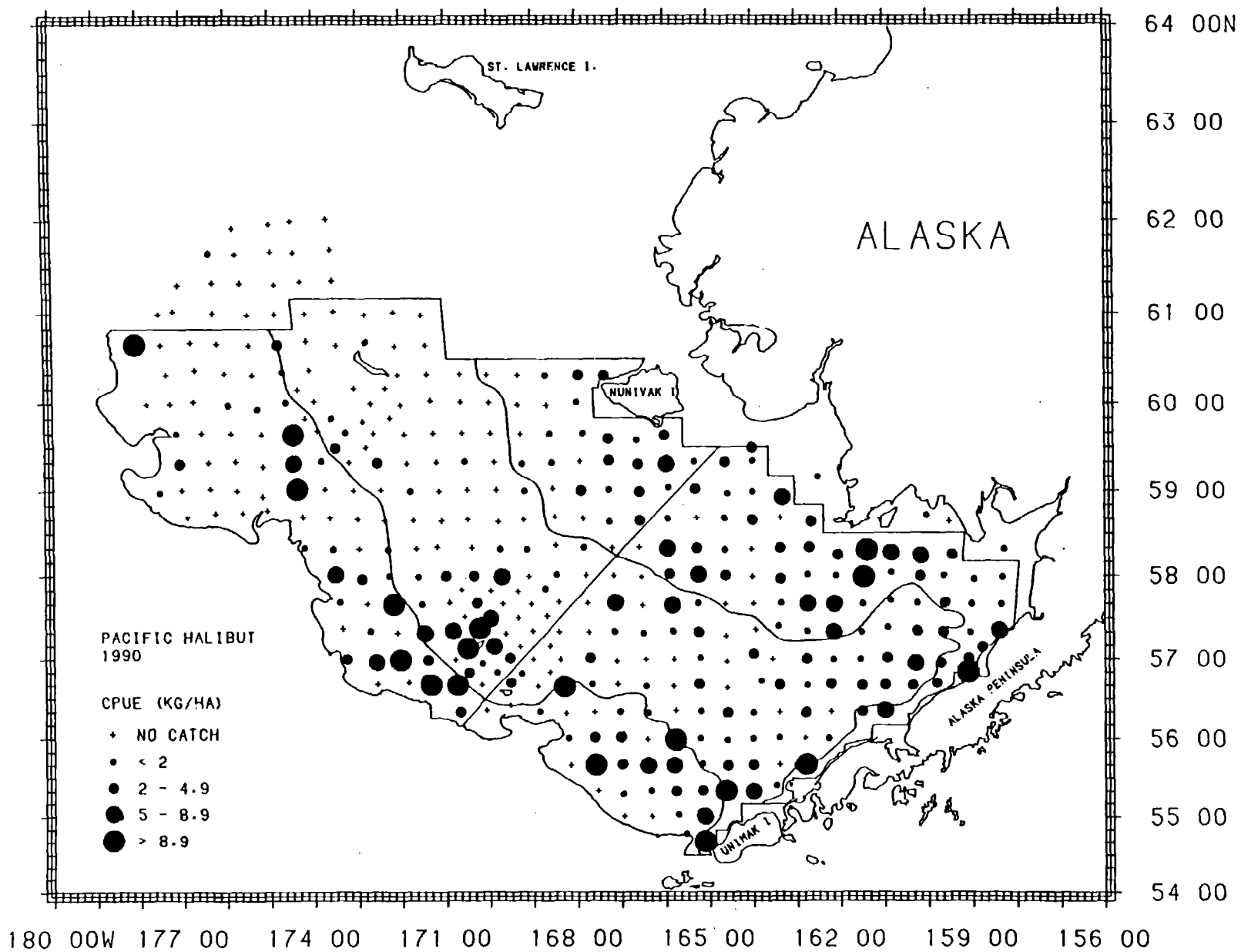
Figure 41.--Distribution and relative abundance in kg/ha of Pacific halibut, 1990 eastern Bering Sea bottom trawl survey.
