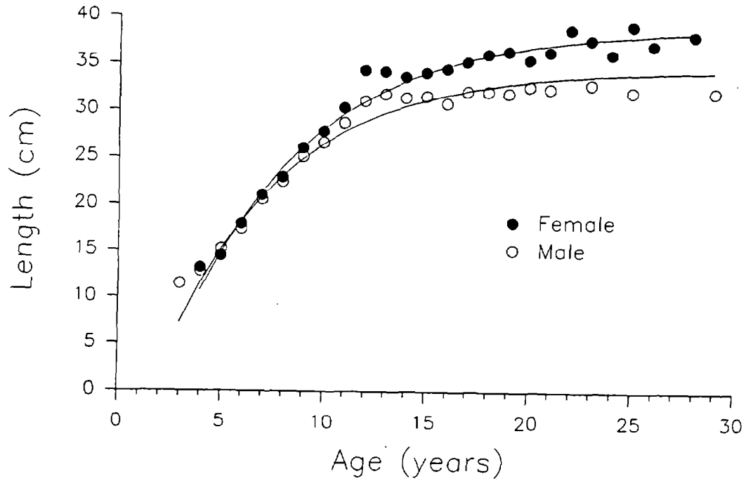
Figure 23.--Von Bertalanffy growth curves and mean lengths at age (symbols) for male and female yellowfin sole, 1990 age eastern Bering Sea bottom trawl survey.
