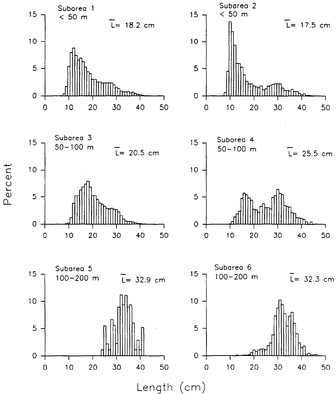
Figure 25. --Estimated relative size composition of rock sole (sexes combined) by subarea, 1990 eastern Bering Sea bottom trawl survey.
