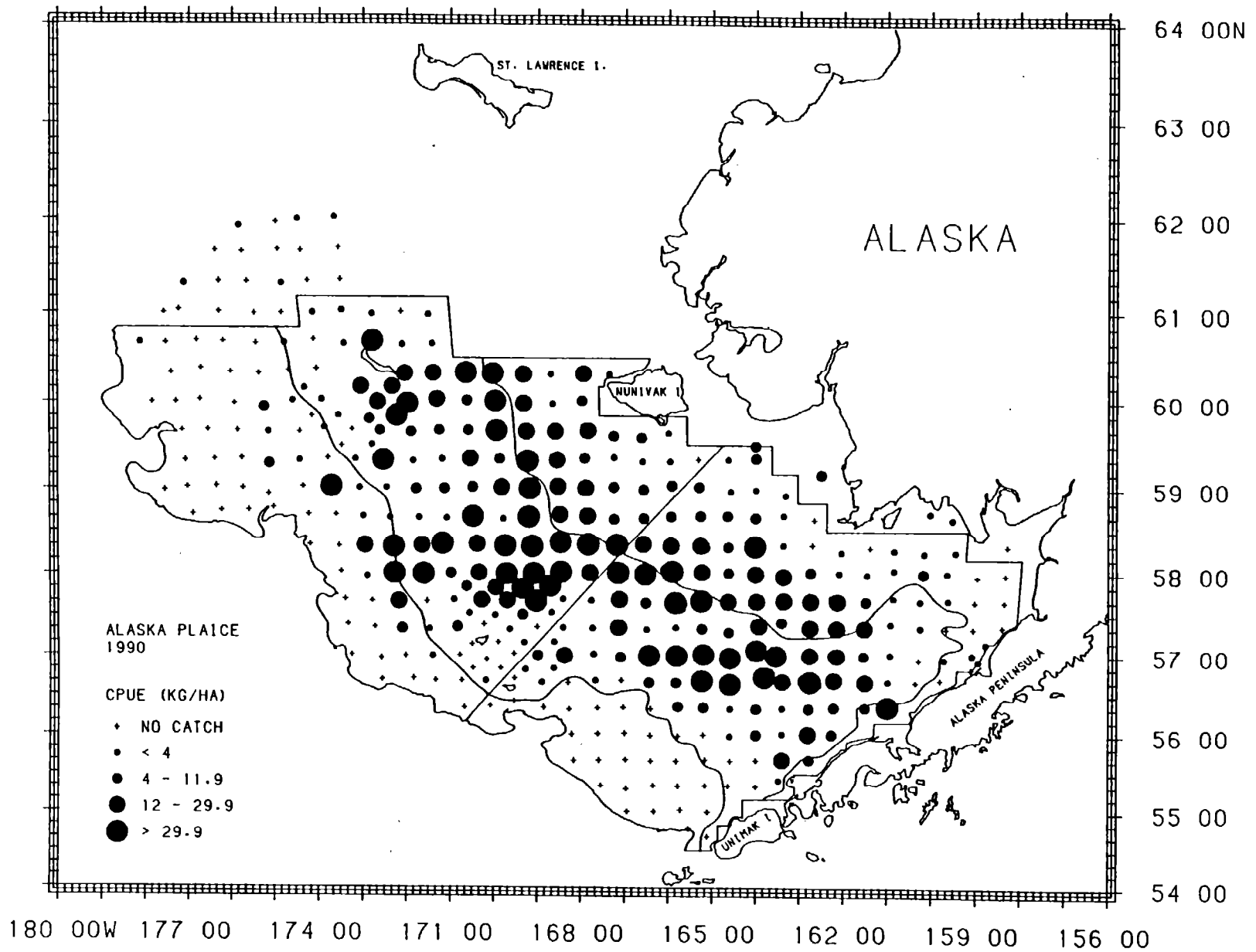
Figure 32.--Distribution and relative abundance in kg/ha of Alaska plaice, 1990 eastern Bering Sea bottom trawl survey.
