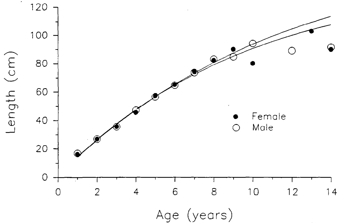
Figure 18.--Von Bertalanffy growth curves and mean lengths at age (symbols) for male and female Pacific cod, 1990 eastern Bering Sea bottom trawl survey.
