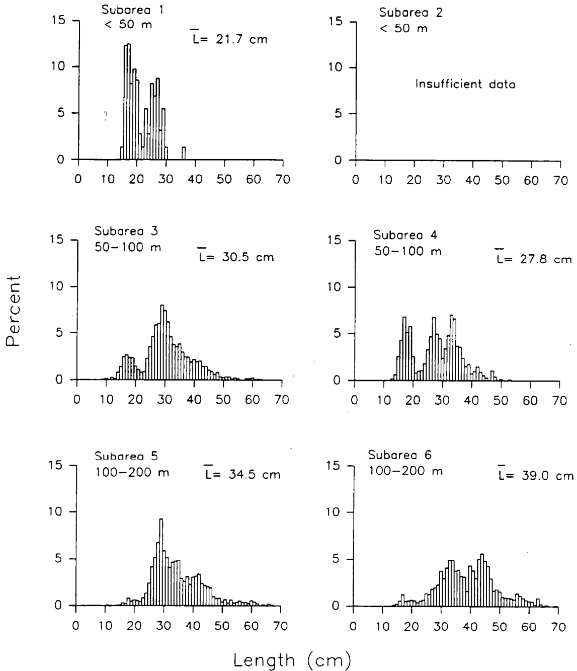
Figure 39. --Estimated relative size composition of Atheresthes spp. (sexes combined) by subarea, 1990 eastern Bering Sea bottom trawl survey.
