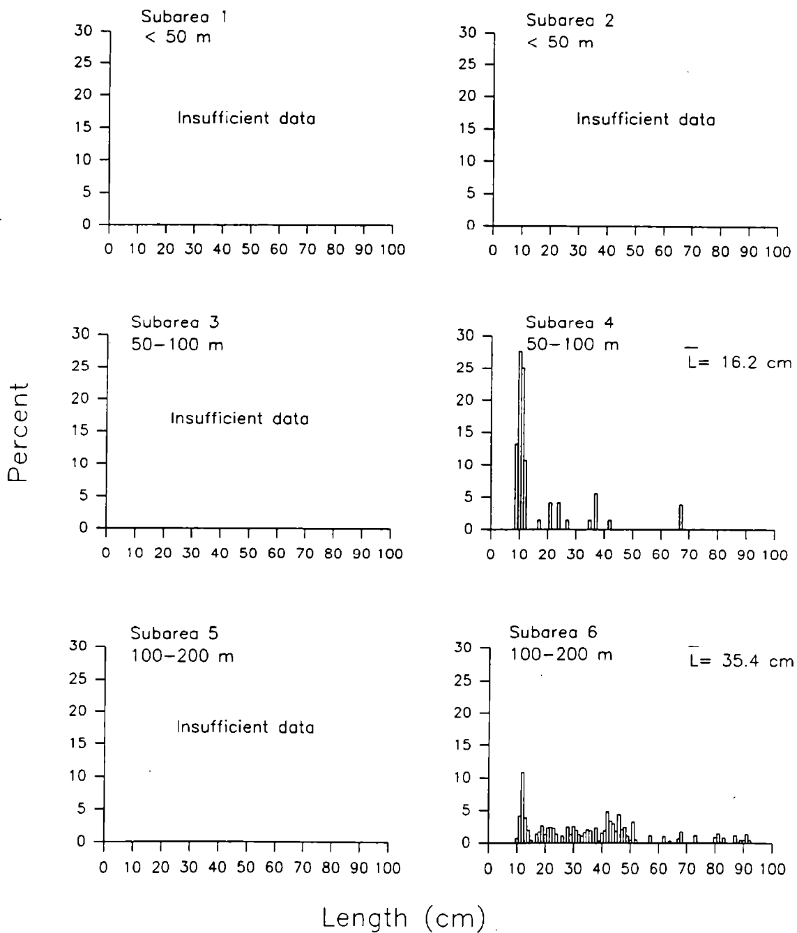
Figure 36. --Estimated relative size composition of Greenland turbot (sexes combined) by subarea, 1990 eastern Bering Sea bottom trawl survey.
