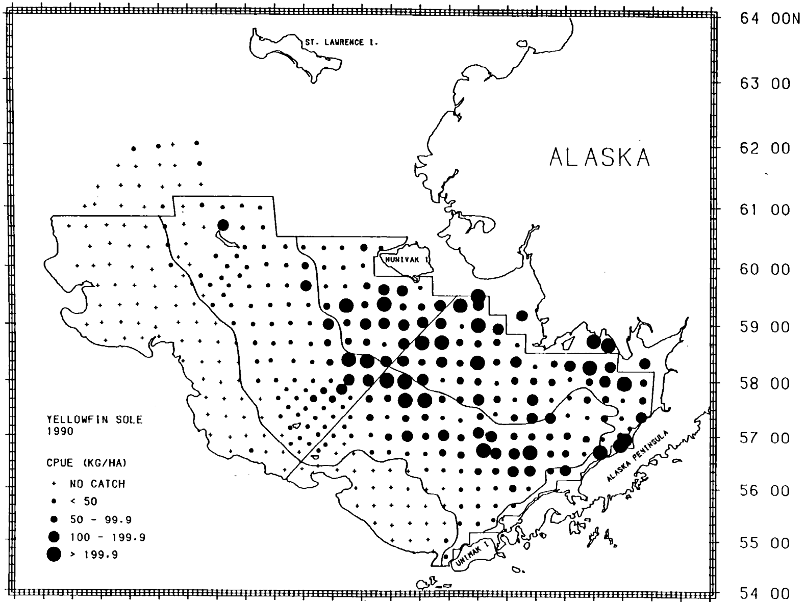
180 00W 177 00 174 00 171 00 168 00 165 00 162 00 159 00 156 00
