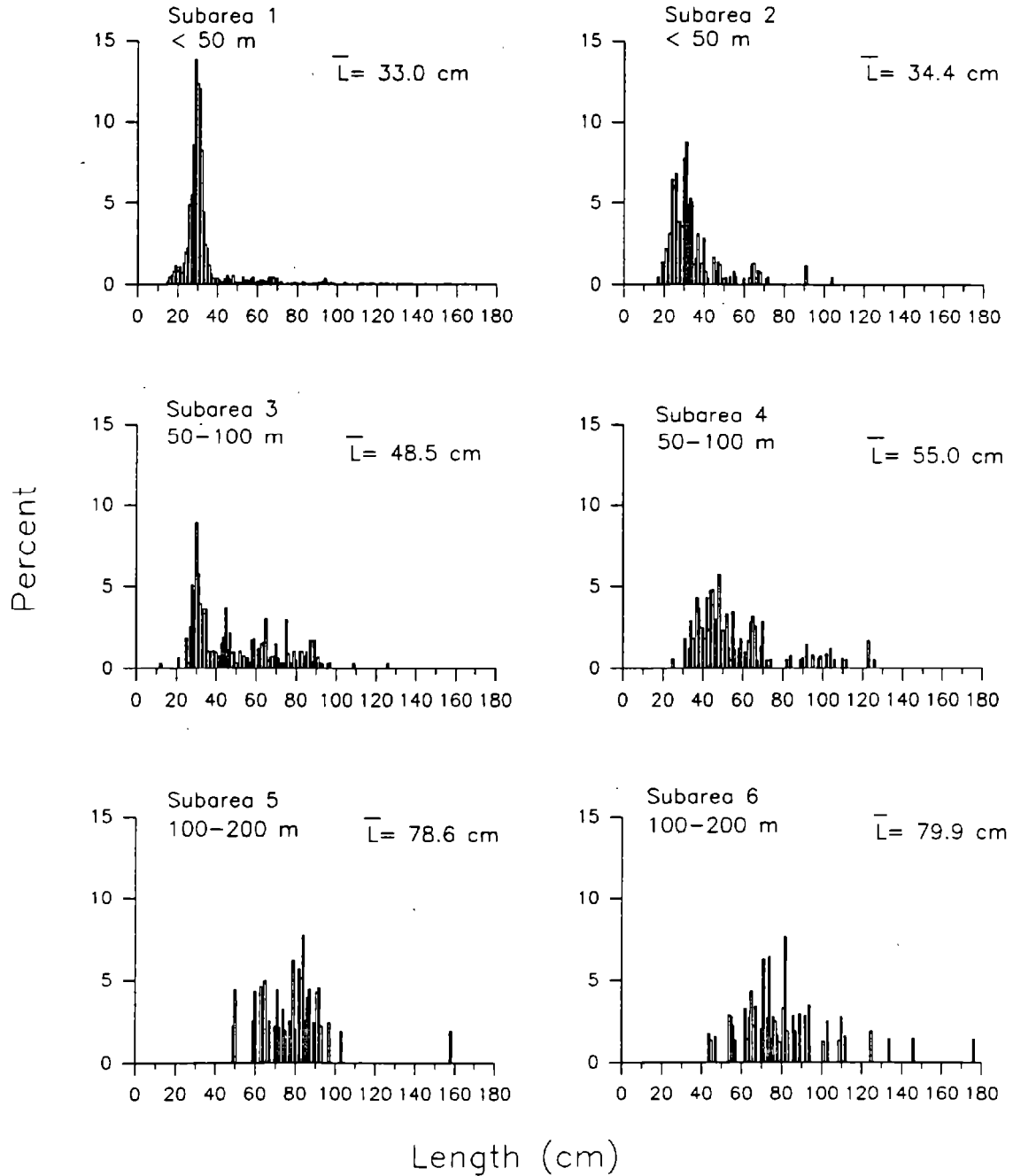
Figure 42. --Estimated relative size composition of Pacific halibut (sexes combined), by subarea, 1990 eastern Bering Sea bottom trawl survey.
