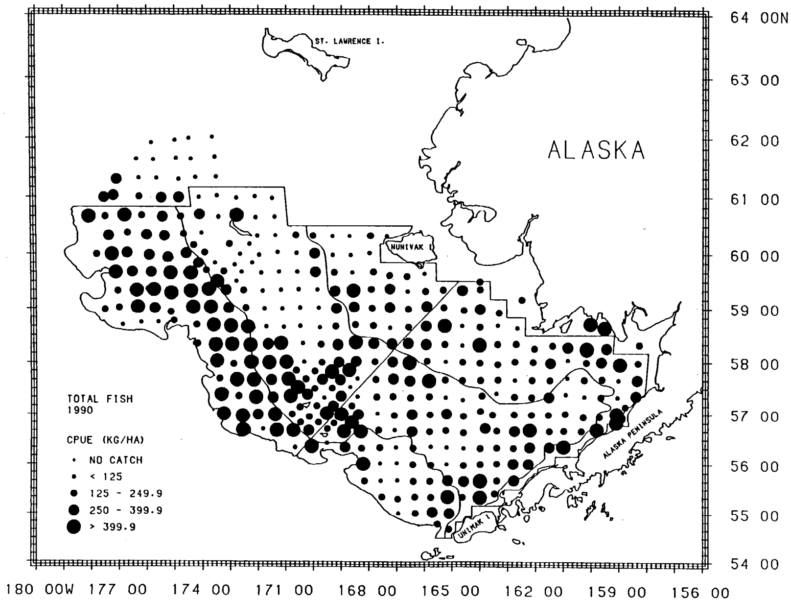
Figure 7.--Distribution and relative abundance in kg/ha of total fish, 1990 eastern Bering Sea bottom trawl survey.
