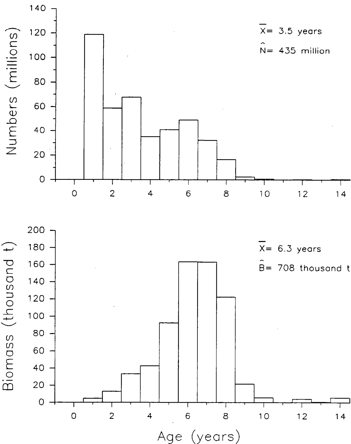
Figure 17. --Population number and biomass (metric tons) estimates by age for Pacific cod, 1990 eastern Bering Sea bottom trawl survey.
