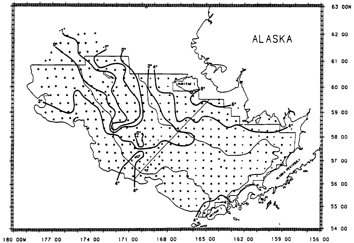
Figure 5. --Distribution of surface water (top panel) and bottom water (lower panel) temperatures (°C) observed during the 1990 eastern Bering Sea bottom trawl survey.
