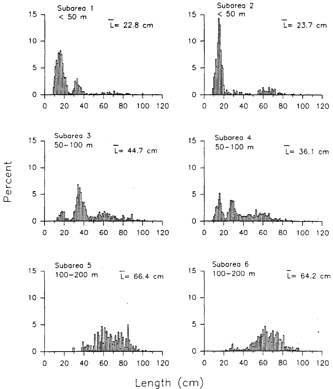
Figure 15. --Estimated relative size composition of Pacific cod (sexes combined) by subarea, 1990 eastern Bering Sea bottom trawl survey.
