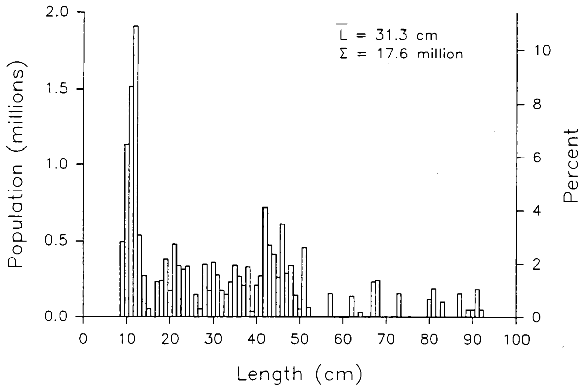
Figure 37. --Estimated size composition of Greenland turbot (sexes combined), all subareas combined, 1990 eastern Bering Sea bottom trawl survey.
