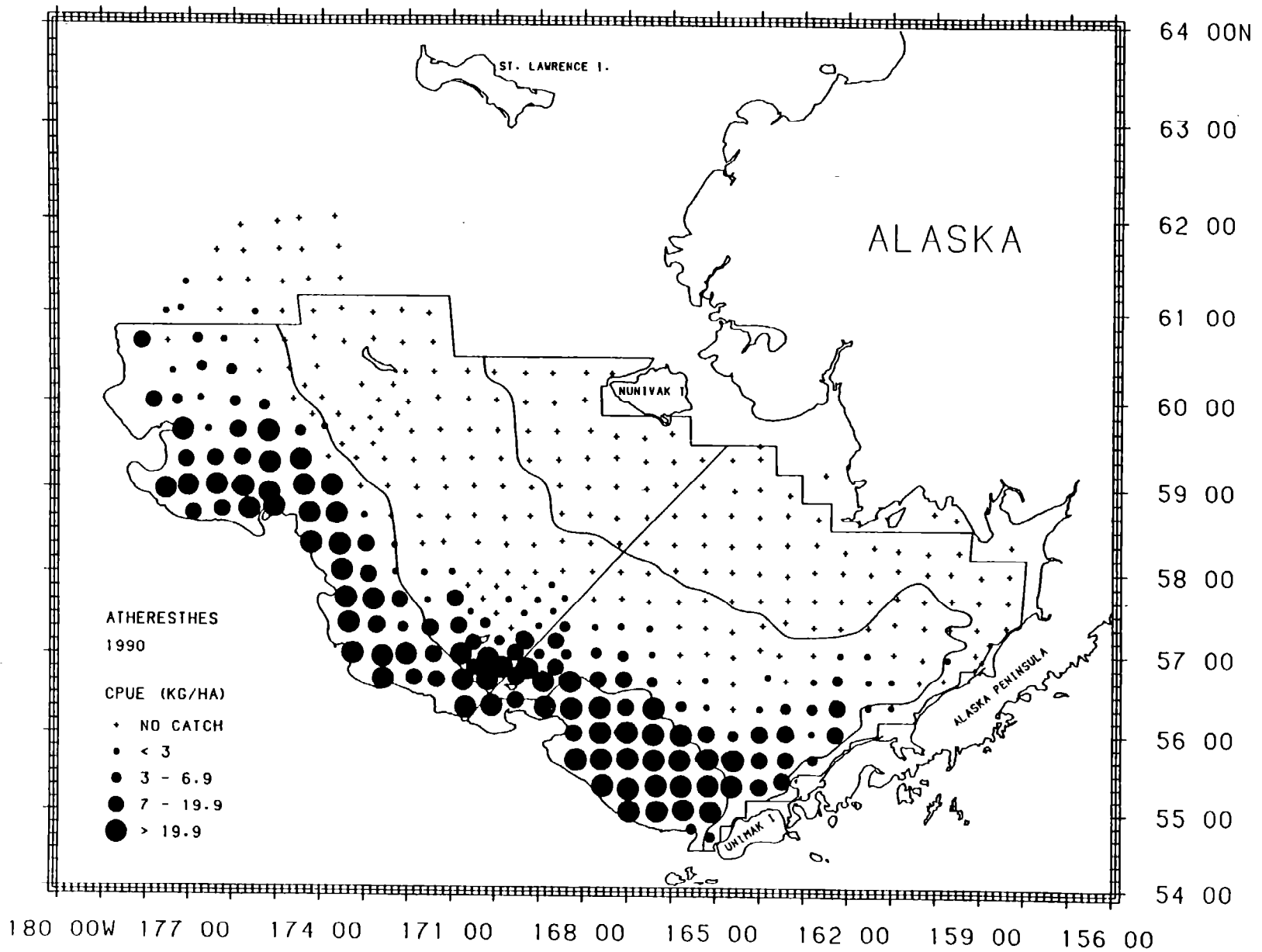
Figure 38.--Distribution and relative abundance in kg/ha of Atheresthes spp., 1990 eastern Bering Sea bottom trawl survey.
