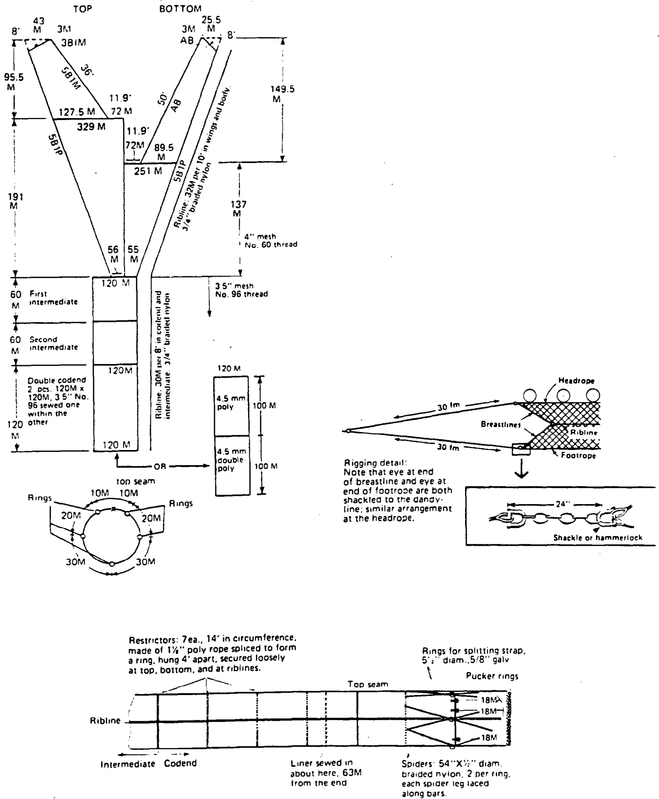
Figure B-1.--Schematic diagram of trawl used during the 1990 eastern Bering Sea bottom trawl survey.
