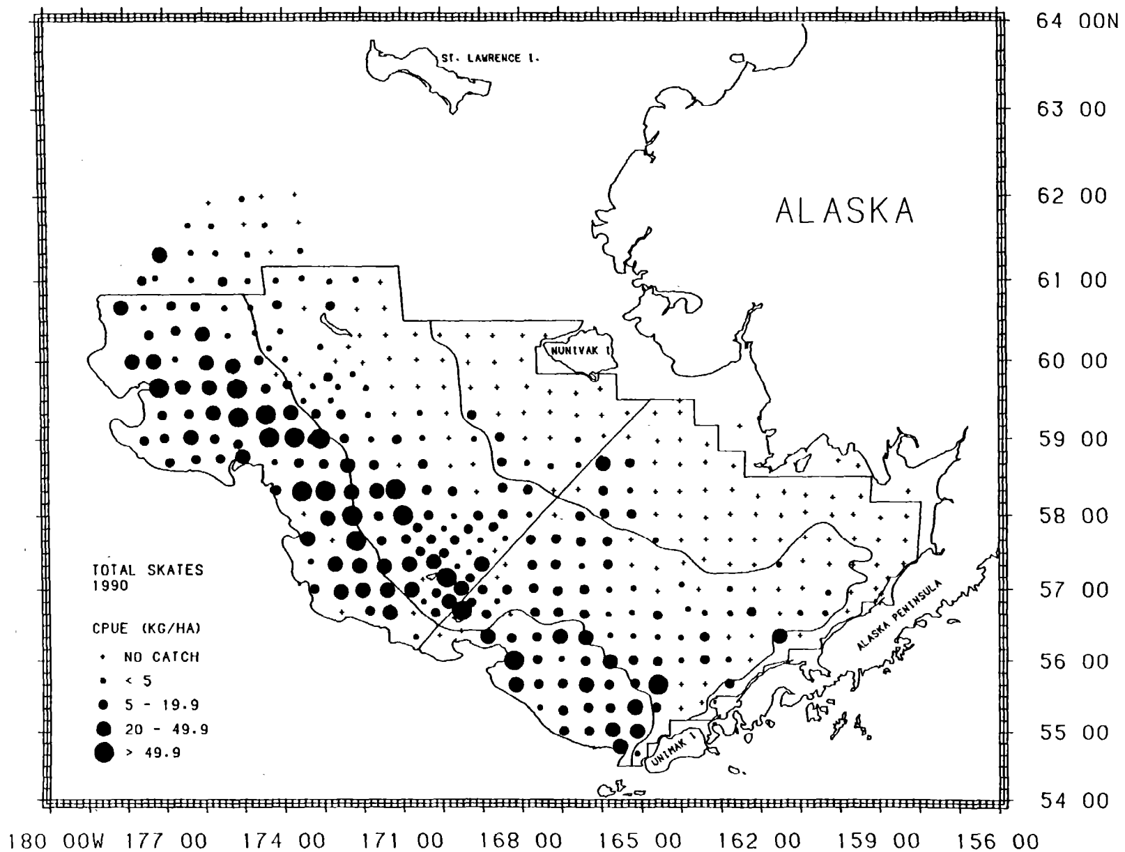
Figure 44. --Distribution and relative abundance in kg/ha of skates, 1990 eastern Bering Sea bottom trawl survey.
