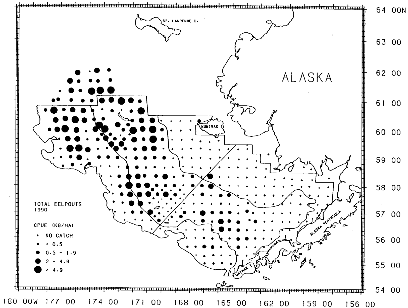
Figure 46.--Distribution and relative abundance in kg/ha of eelpouts, 1990 eastern Bering Sea bottom trawl survey.
