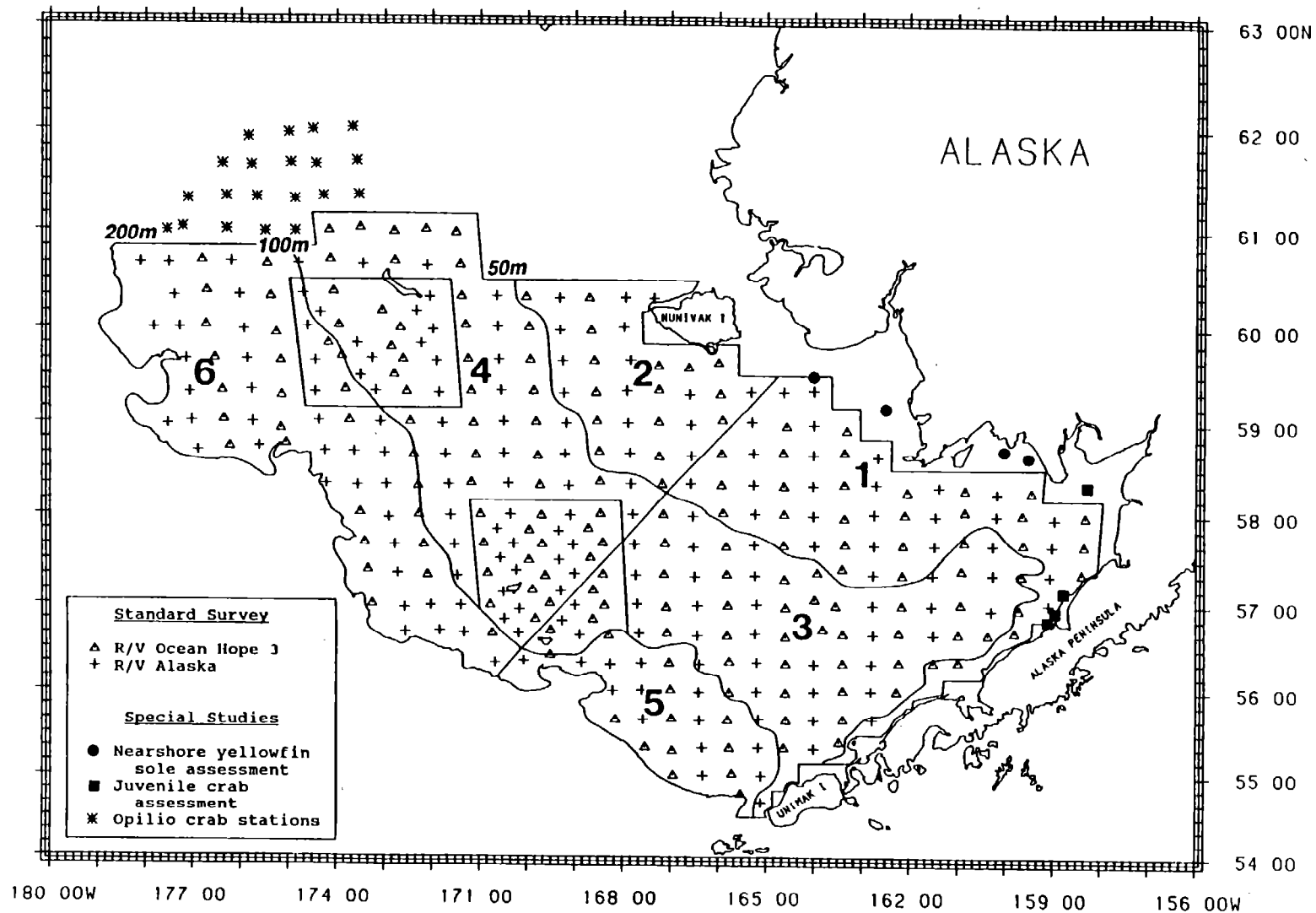
Figure 3.--Standard and special study stations sampled during the 1990 eastern Bering Sea bottom trawl survey, and stratification used for analyses of the data. Boxed areas surrounding the Pribilof Islands and St. Matthew Island indicate locations of high-density sampling.
