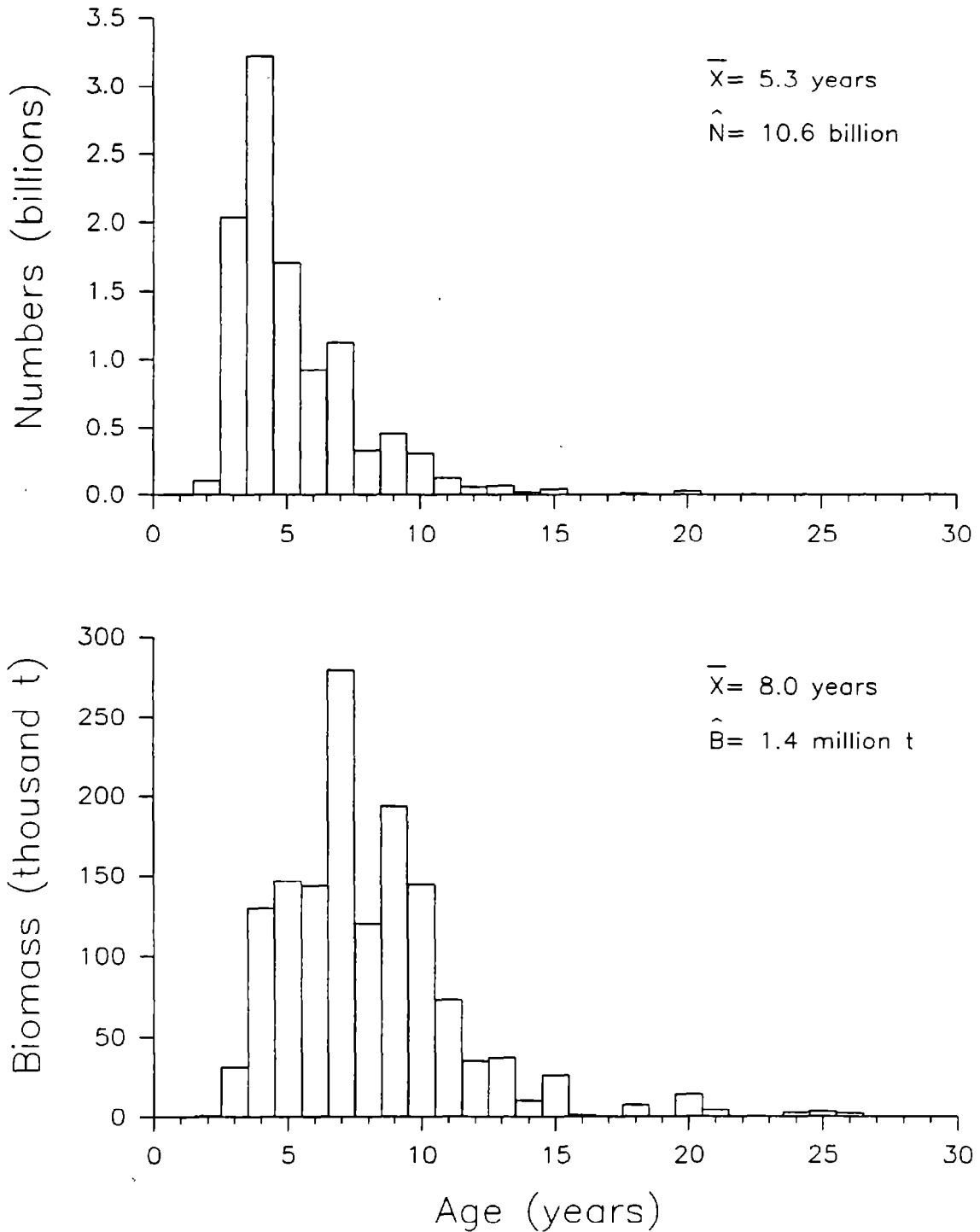
Figure 27. --Population number and biomass (metric tons) estimates by age for rock sole, 1990 eastern Bering Sea bottom trawl survey.
