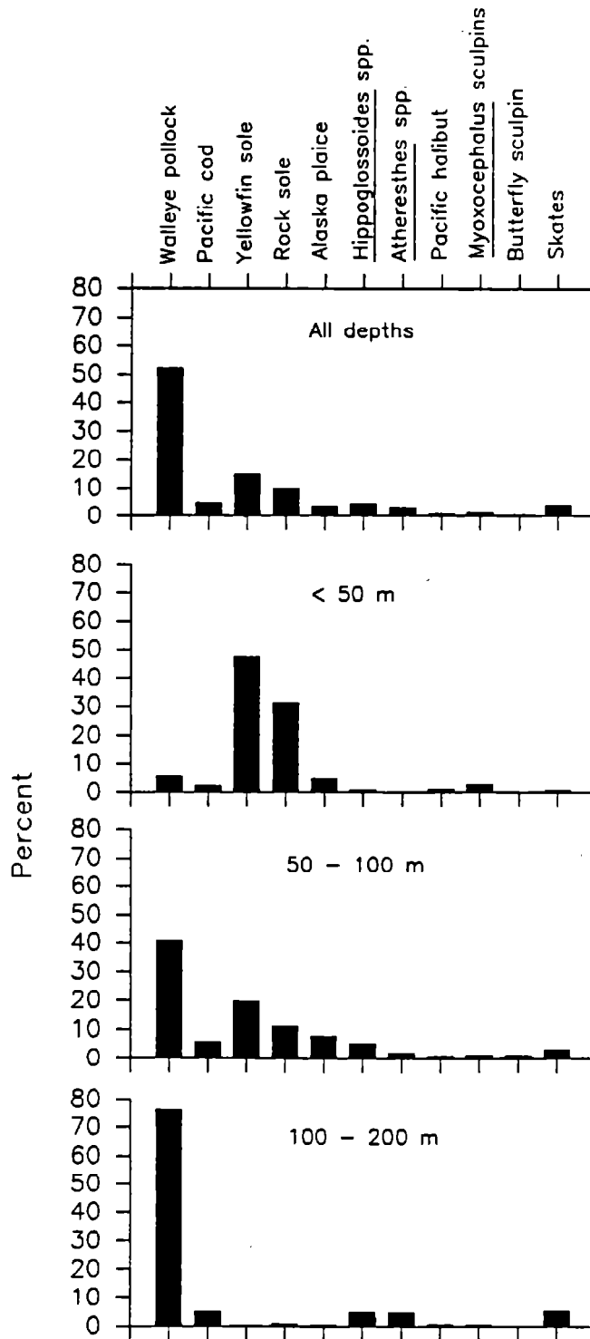
Figure 8. --Relative abundance (%CPUE in kg/ha) of principal groundfish species by depth zone and for all depths combined, 1990 eastern Bering Sea bottom trawl survey.
