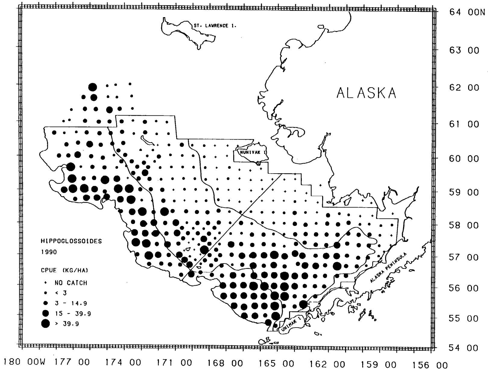
Figure 29.--Distribution and relative abundance in kg/ha of Hippoglossoides spp., 1990 eastern Bering Sea bottom trawl survey.
