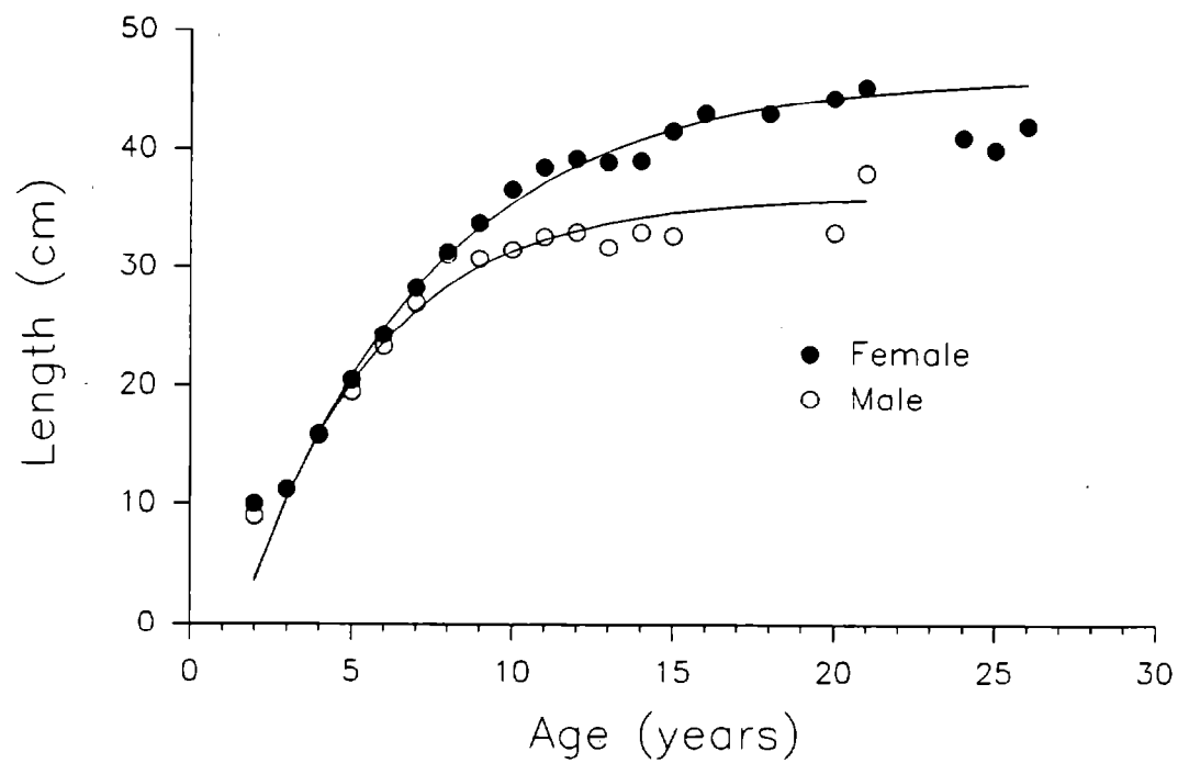
Figure 28.--Von Bertalanffy growth curves and mean lengths at age (symbols) for male and female rock sole, 1990 eastern Bering Sea bottom trawl survey.
