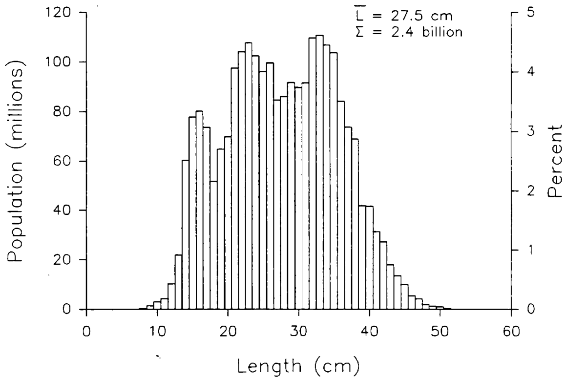
Figure 31.--Estimated size composition of Hippoglossoides spp. (sexes combined), all subareas combined, 1990 eastern Bering Sea bottom trawl survey.
