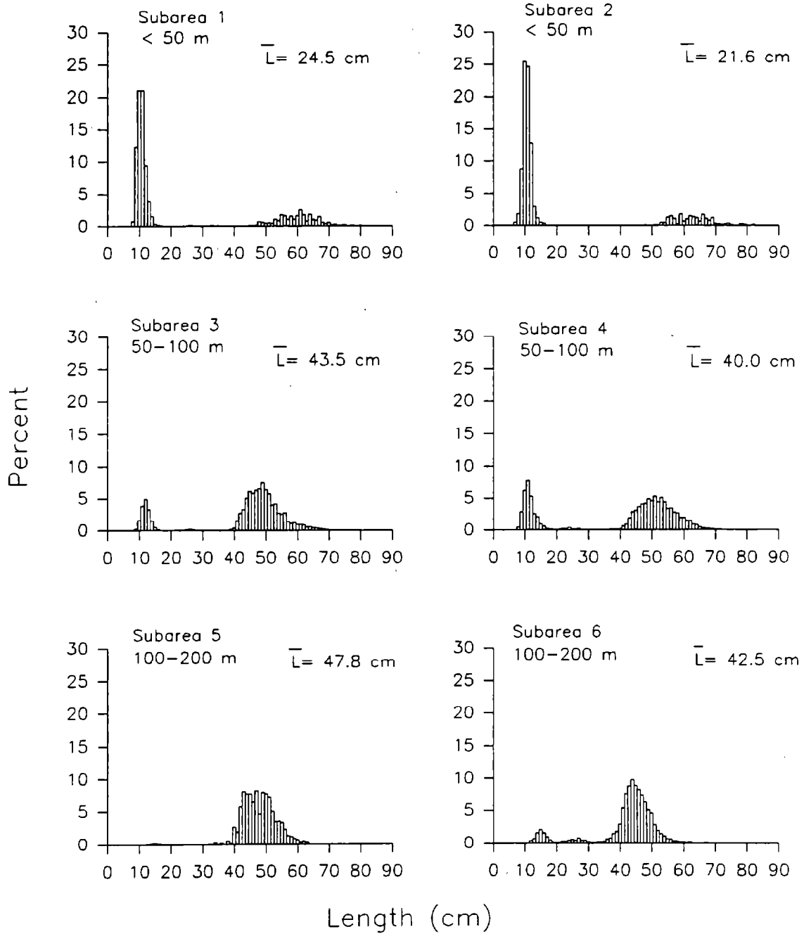
Figure 10. --Estimated relative size composition of walleye pollock (sexes combined) by subarea, 1990 eastern Bering Sea bottom trawl survey.
