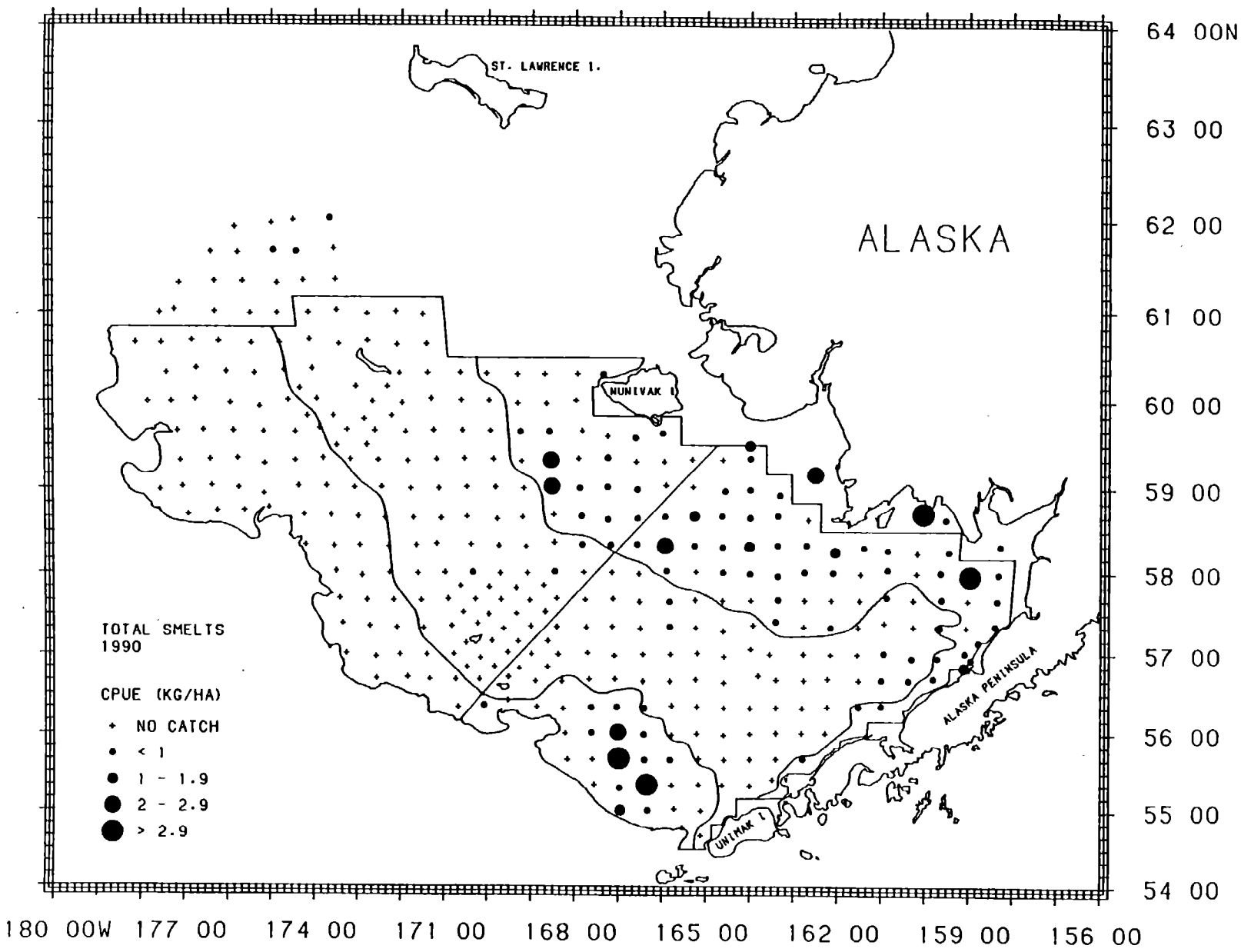
Figure 49. --Distribution and relative abundance in kg/ha of smelts, 1990 eastern Bering Sea bottom trawl survey.
