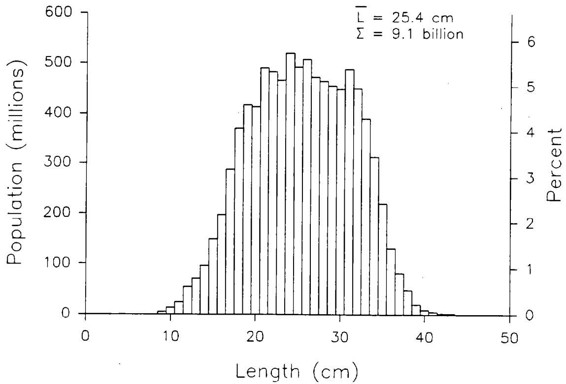
Figure 21. --Estimated size composition of yellowfin sole (sexes combined), all subareas combined, 1990 eastern Bering Sea bottom trawl survey.
