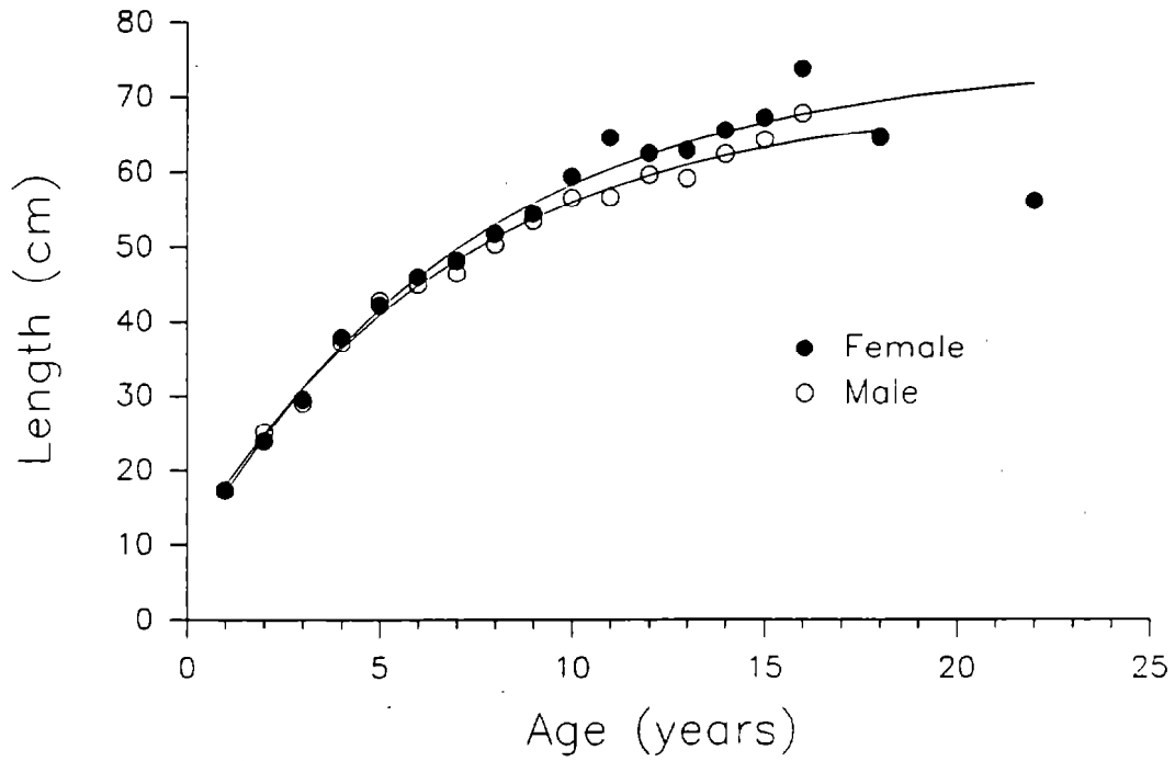
Figure 13. --Von Bertalanffy growth curves and mean lengths at age (symbols) for male and female walleye pollock, 1990 eastern Bering Sea bottom trawl survey.
