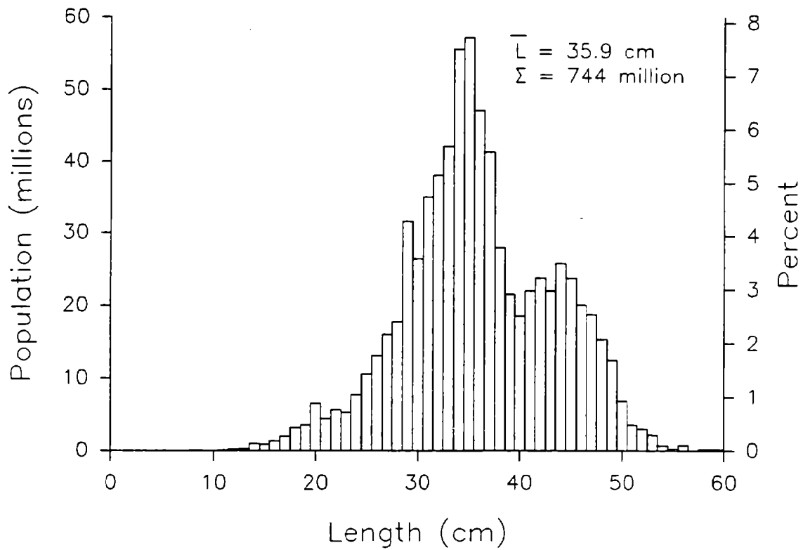
Figure 34.--Estimated size composition of Alaska plaice (sexes combined), all subareas combined, 1990 eastern Bering Sea bottom trawl survey.
