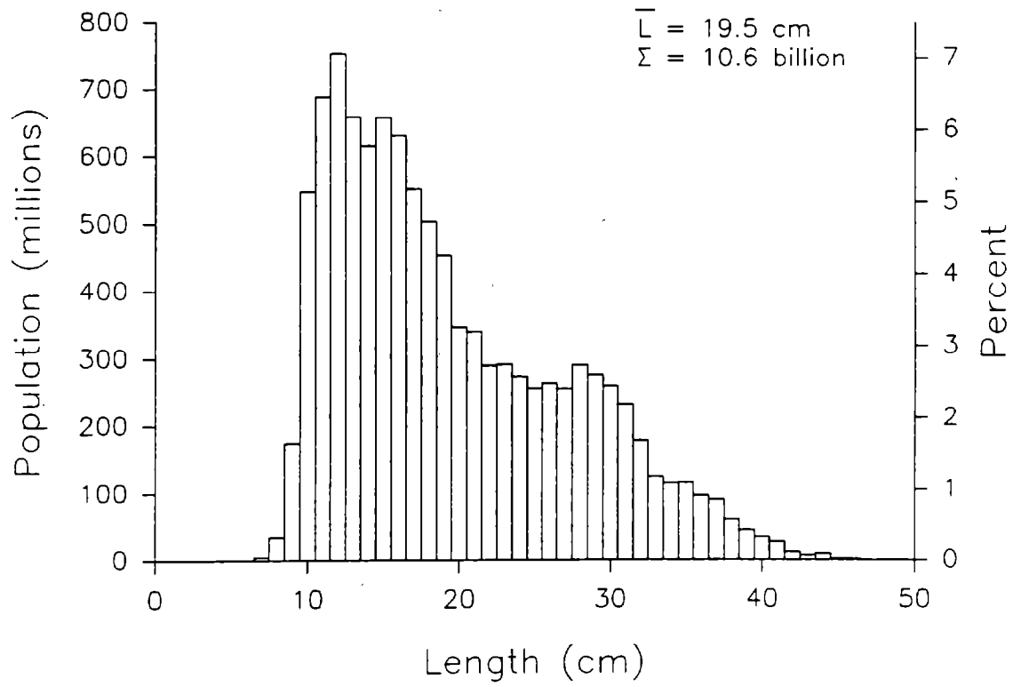
Figure 26. --Estimated size composition of rock sole (sexes combined), all subareas combined, 1990 eastern Bering Sea bottom trawl survey.
