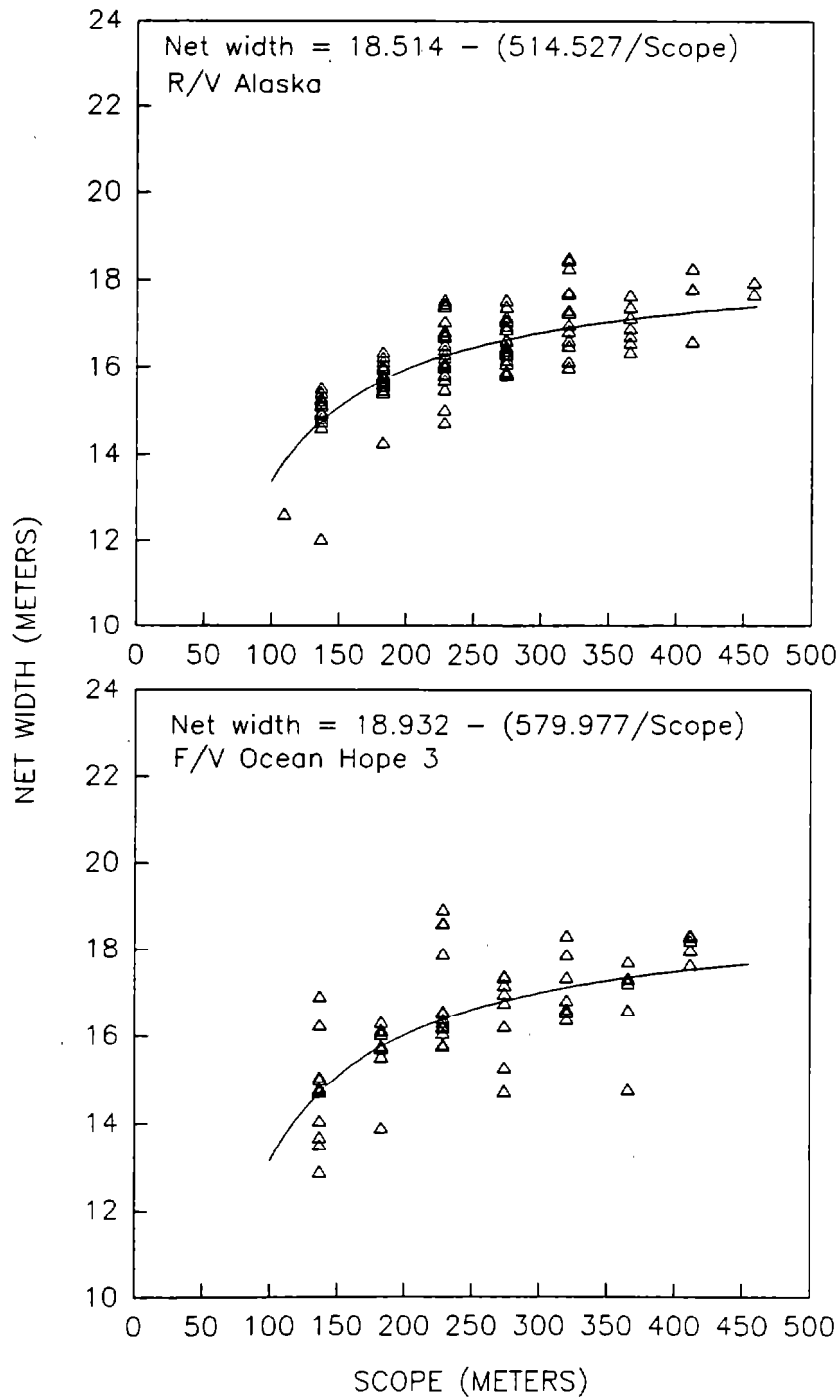
Figure 4. --Relationship between net-width and scope (wire-out) for the two vessels participating in the 1990 eastern Bering Sea bottom trawl survey.
