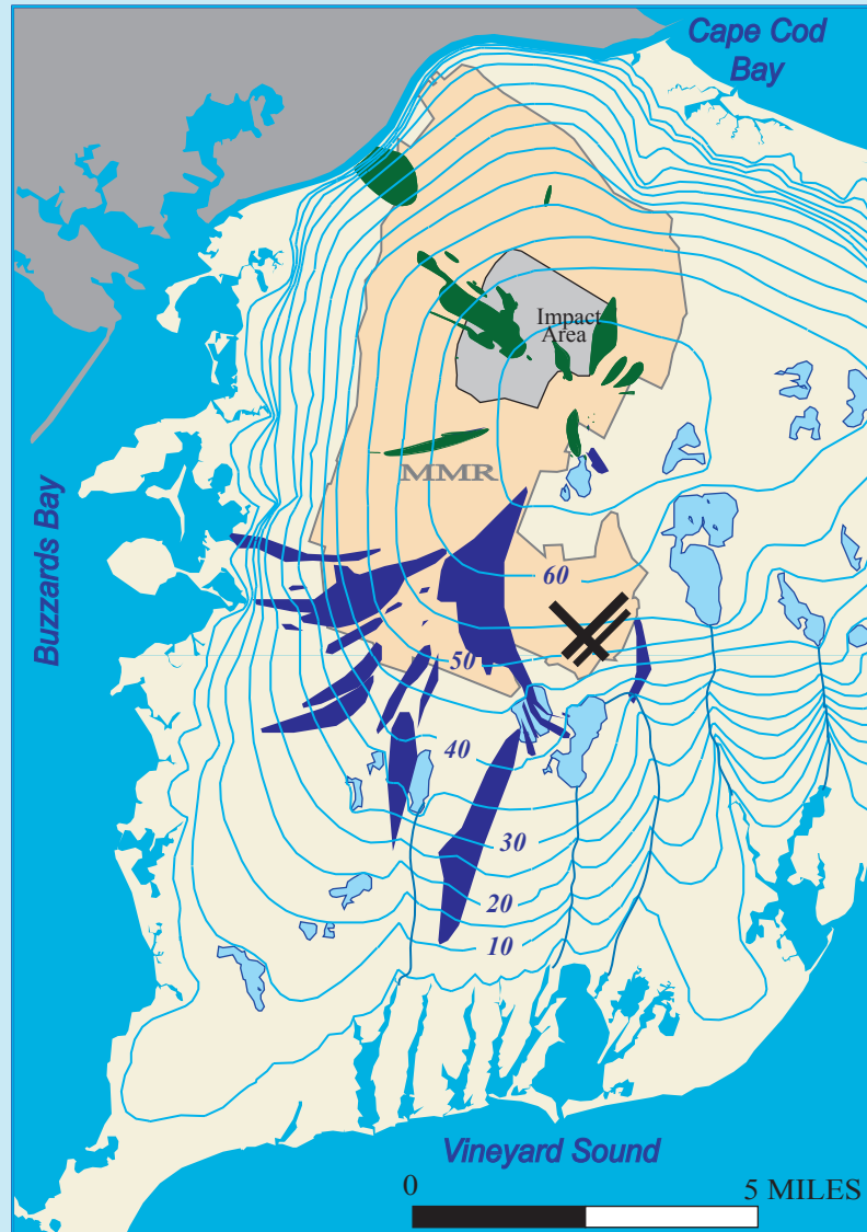
Ground-water contaminant plumes at and near the Massachusetts Military Reservation in February 2005. The green plumes are composed primarily of explosive compounds and perchlorate. The blue plumes are composed primarily of chlorinated solvents and ethylene dibromide. The water-table contours are shown in feet above sea level. Source of information: Air Force Center for Environmental Excellence Installation and Army
