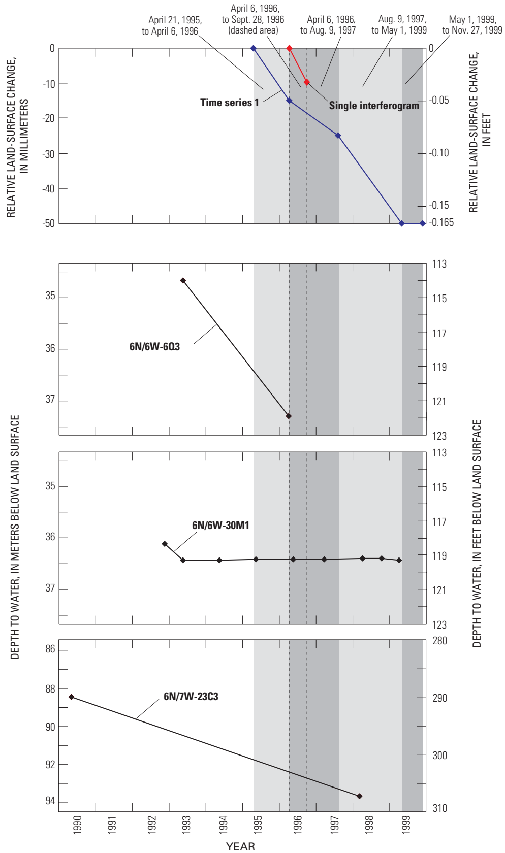
Figure 8. Depth to water for selected wells and relative land-surface change in the El Mirage area, San Bernardino County, California. (See figure 7A for locations of wells.)
