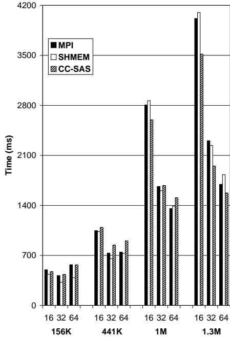
Figure 3: Runtimes (in milliseconds) for the Dynamic Remeshing problem on 16, 32, and 64 processors for different data sets.
