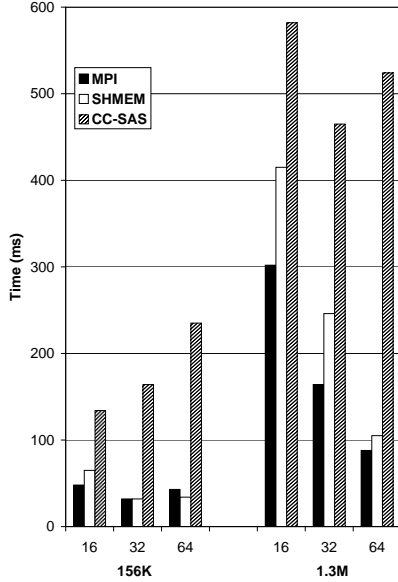
Figure 5: Runtimes (in milliseconds) for the Mesh Adaptor module on 16, 32, and 64 processors for the 156K and 1.3M data sets.
