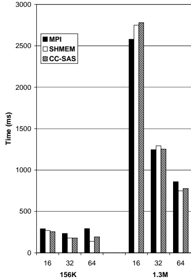
Figure 7: Runtimes (in milliseconds) for the Solver on 16, 32, and 64 processors for the 156K and 1.3M data sets.
