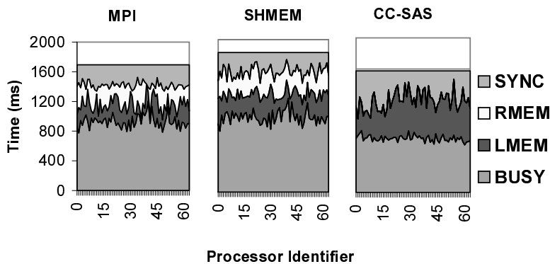
Figure 4: Time breakdown for the 1.3M data set size on 64 processors.
