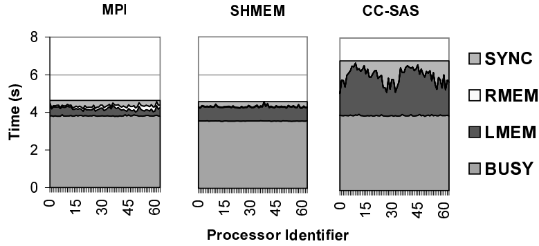
Figure 10: Time breakdown for the 1M data set on 64 processors.
