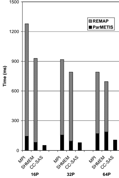
Figure 6: Runtimes (in milliseconds) for Load Balancing (ParMETIS Partitioning and Remapping), and partitioning quality on 16, 32, and 64 processors for the 1.3M data set.
