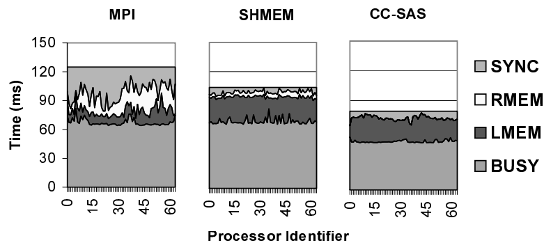
Figure 9: Time breakdown for the 16K data set on 64 processors.
