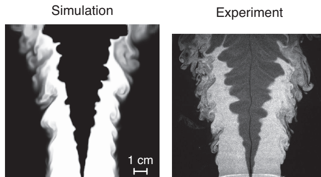
Figure 3: Computed \text{CH}_4 mole fraction and typical Mie scattering image used for PIV.
