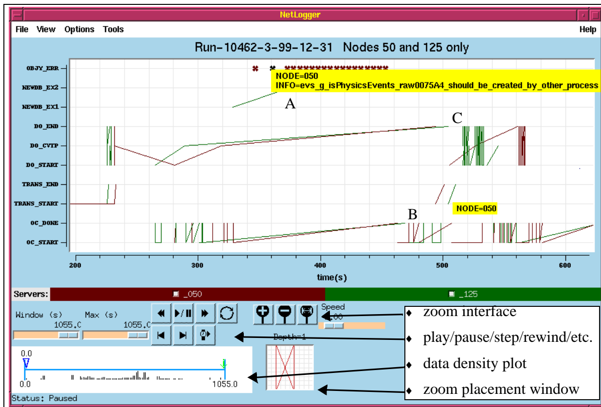
Figure 2: nlv screen dump showing Objectivity errors: nodes 50 and 125
