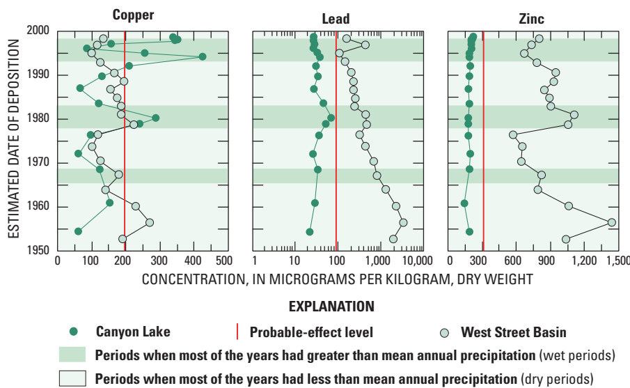
Figure 22. Trace-element concentrations in reservoir-sediment cores often exceeded guidelines established for protecting aquatic life at West Street Basin. Concentrations of lead and zinc in sediment core at Canyon Lake are lower than at West Street Basin.
