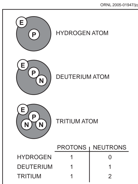
Fig. G.1. The hydrogen atom and its isotopes.
