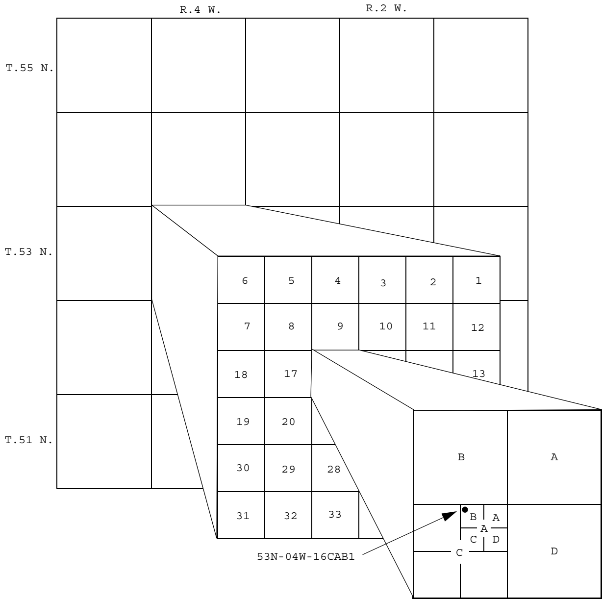
Figure 3. Diagram showing Idaho well-numbering system.
