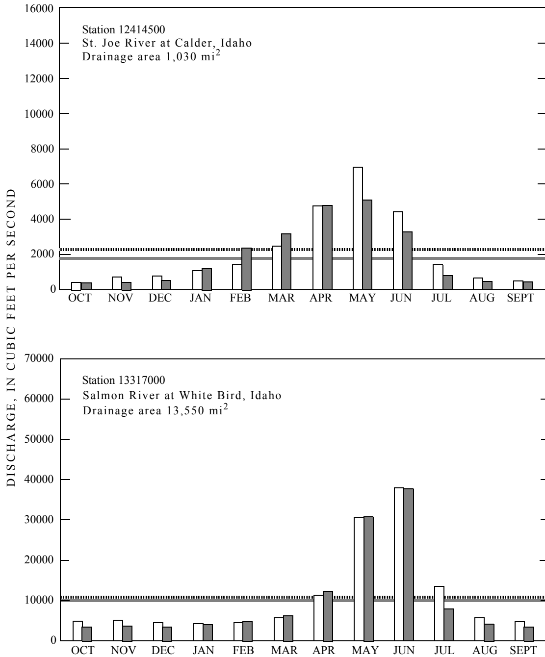
Figure 1. Discharge during 2003 water year compared with median discharge for period 1971-2000 for two representative gaging stations.
