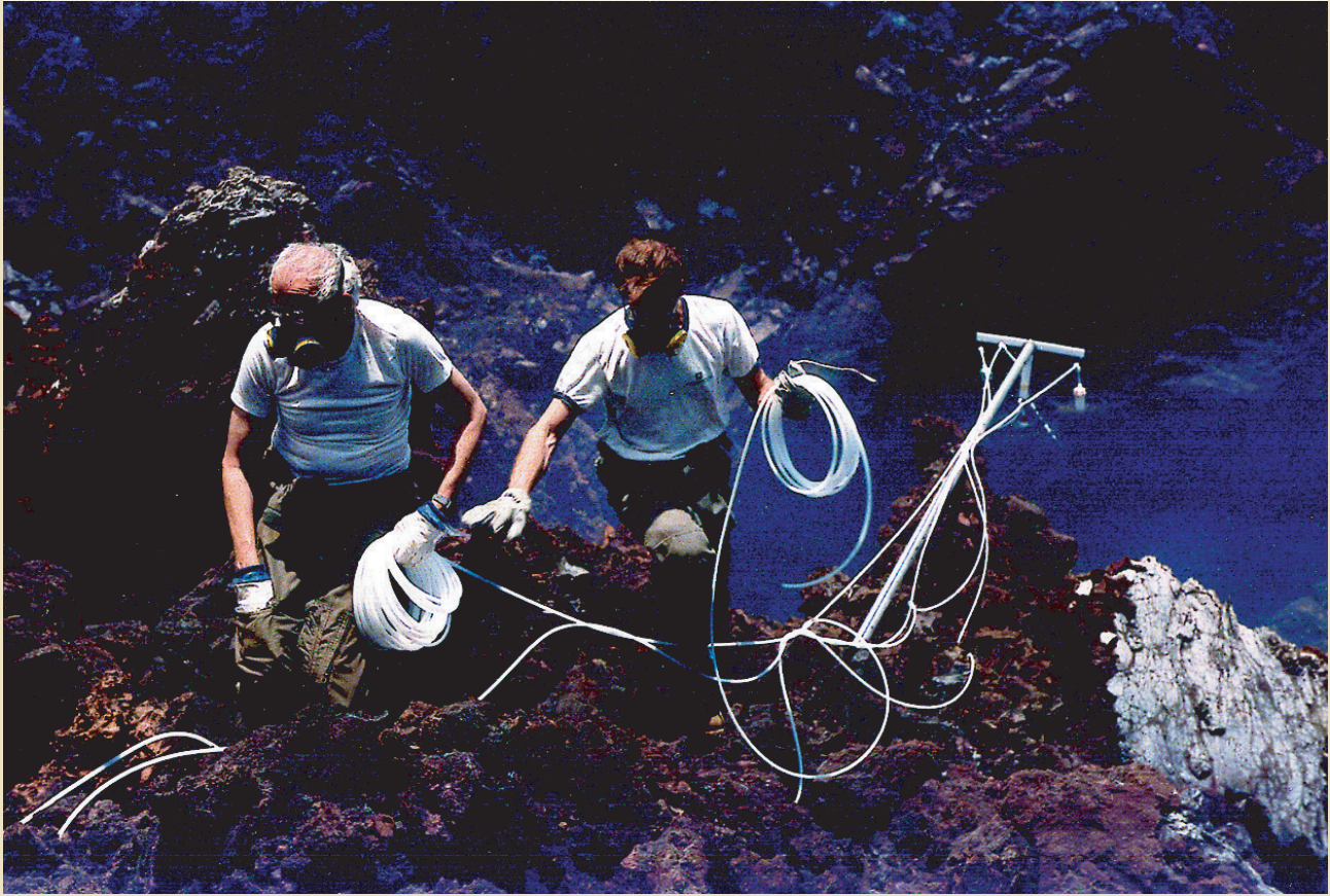
Figure 29. USGS and university scientists collecting volcanic gas samples for the measurement of mercury and other chemical constituents.
