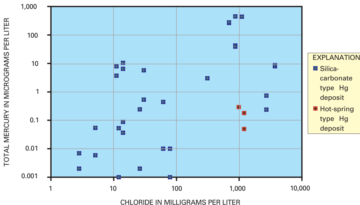
Figure 14. Total mercury concentration in acid-rock drainage from silica-carbonate and hot-spring-type mercury deposits in the California mercury mineral belt as a function of chloride concentration.
