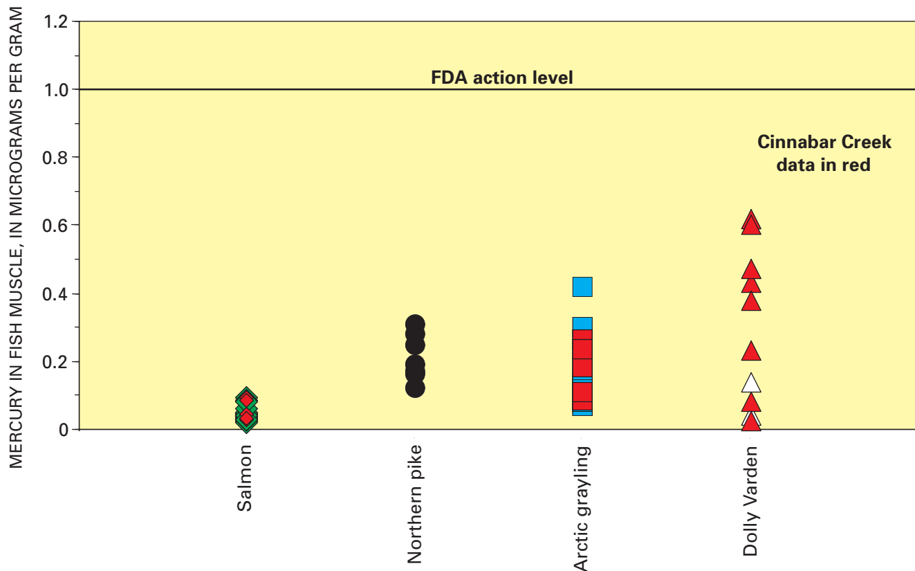
Figure 18. Mercury concentration in muscle for fish collected in southwestern Alaska. Fish collected nearest Cinnabar Creek mercury mine contain highest mercury concentrations. FDA action level is shown for reference.
