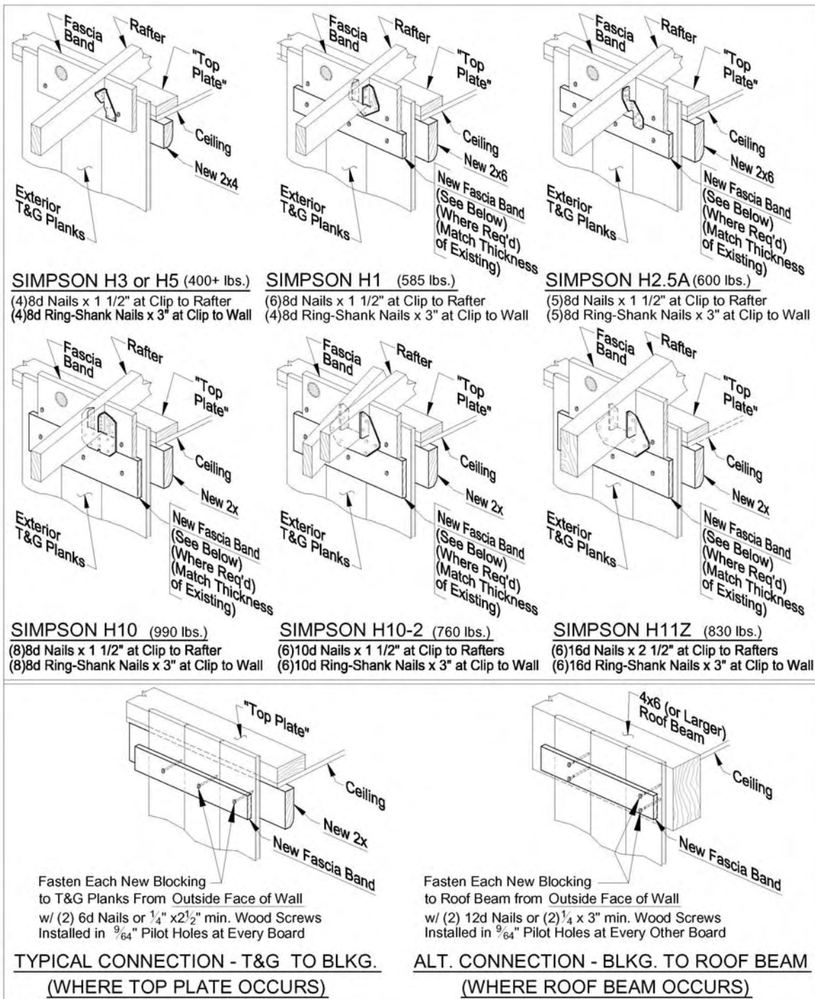
Figure 4B: Roof to Wall Uplift Resistant Ties for "Single Wall" Construction – Existing Fascia Extending Below Rafter
