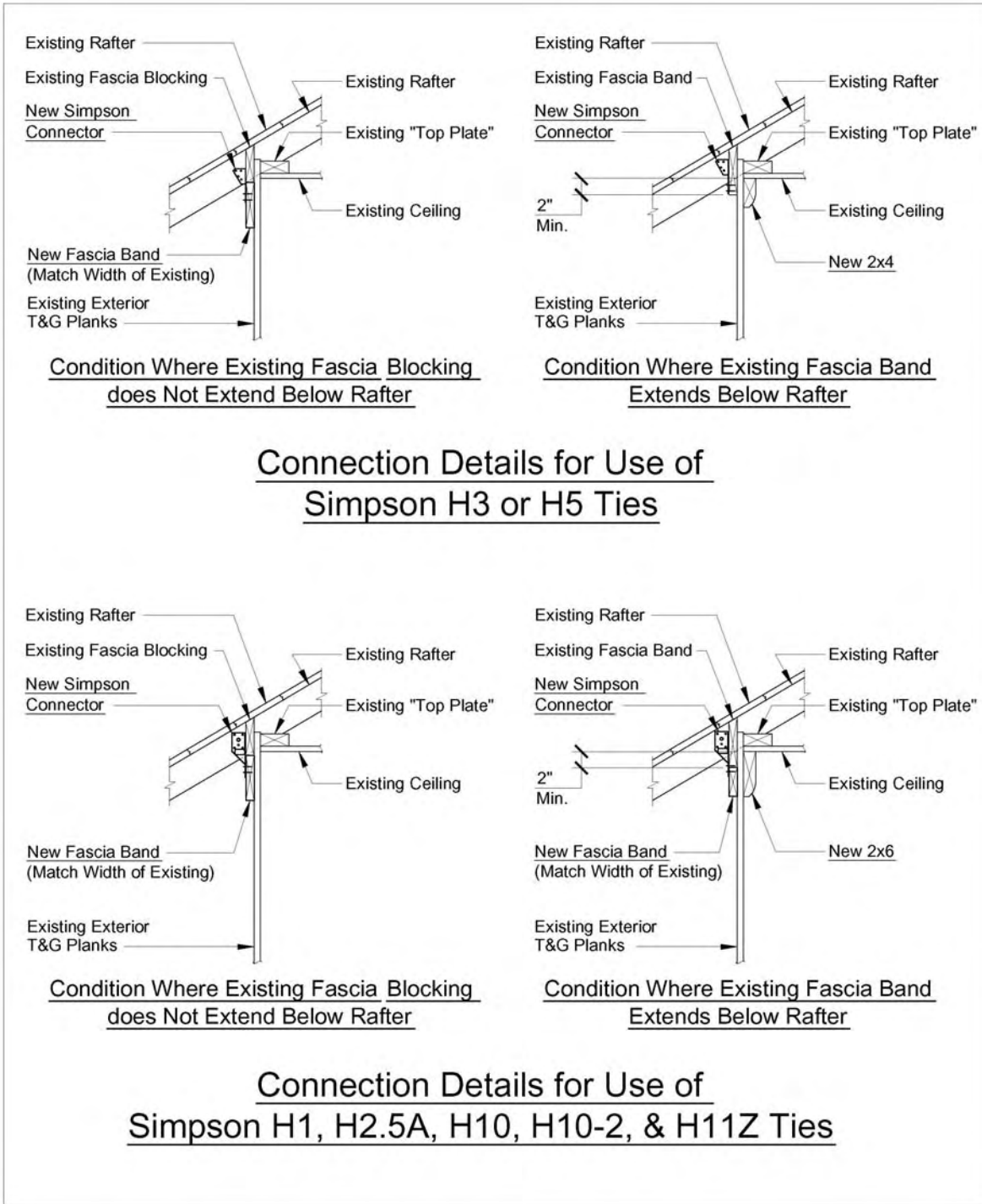
Figure 4: Roof to Wall Uplift Resistant Ties for "Single Wall" Construction
