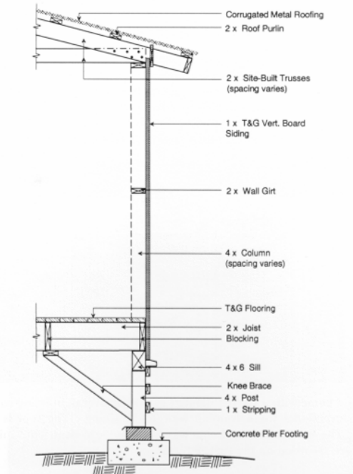
Figure 2: “Single Wall” House with Wood Piers and Concrete “Tofu” Block Foundation (note columns may not exist)
