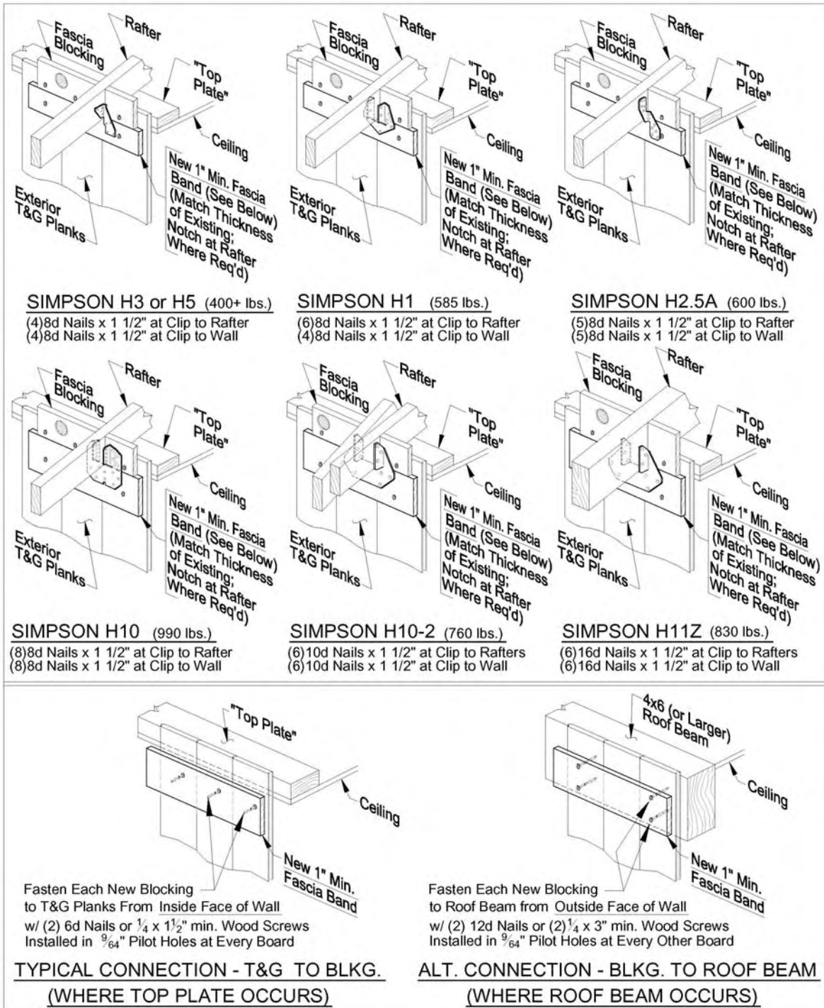
Figure 4A: Roof to Wall Uplift Resistant Ties for "Single Wall" Construction— Existing Fascia Not Extending Below Rafter
