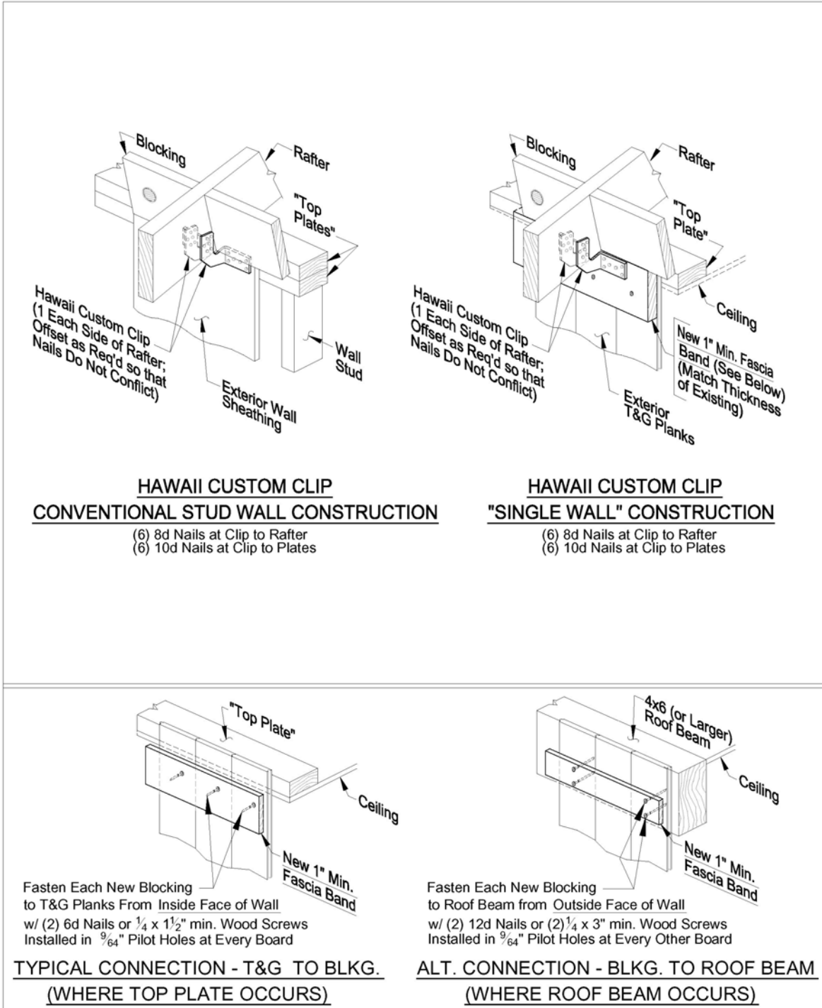
Figure 4C: Roof to Wall Uplift Resistant Ties for Hawaii Custom Clips on Construction Where Rafter Spacing Does Not Exceed 24 Inches and Roof Span Does Not Exceed 24 Feet
