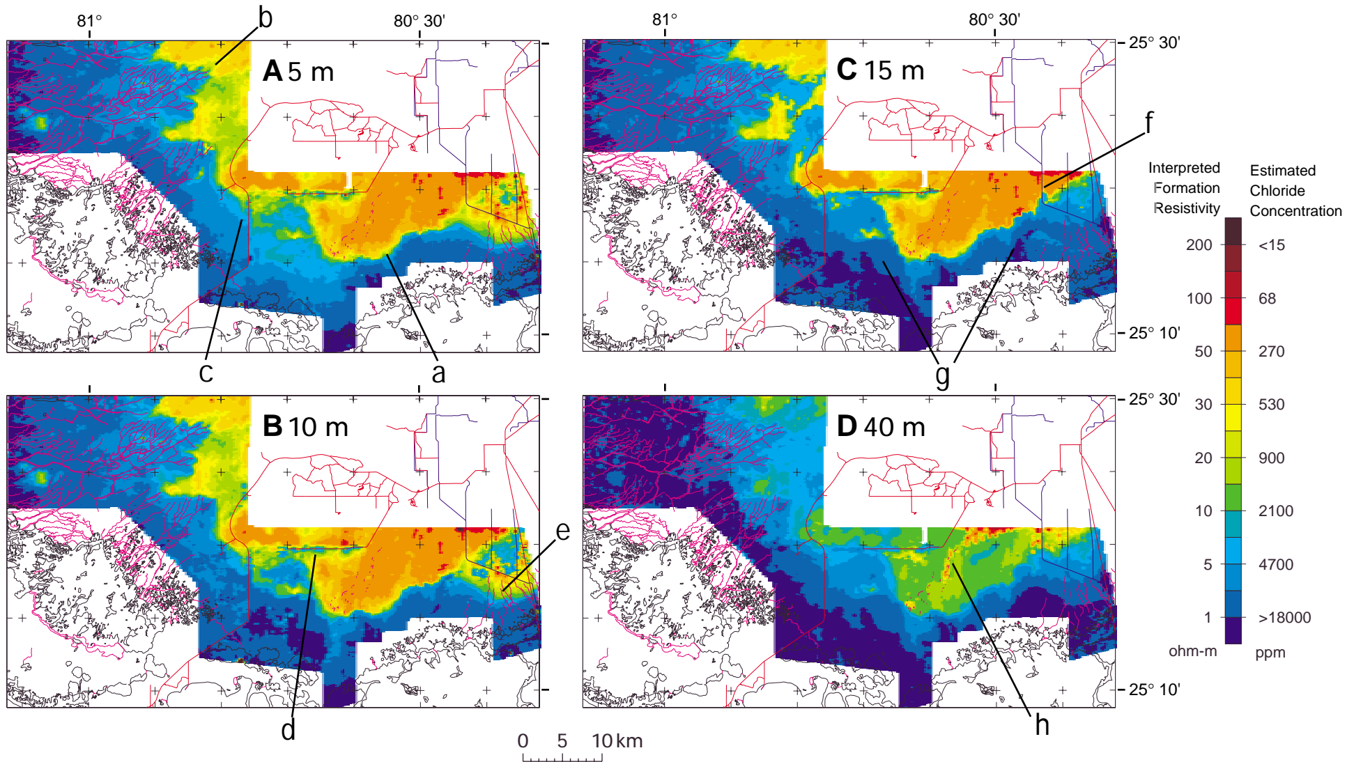
Figure 5 Interpreted HEM resistivity-depth-slice map from Everglades National Park for depths of 5 m (A), 10 m (B), 15 m (C), and 40 m (D). Annotated features are discussed in the text.
