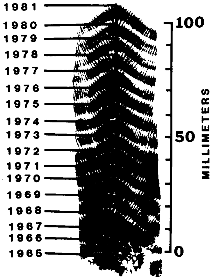
Figure 6. X-radiograph positive print of Porites lutea core slab from Matinloc showing annual growth bands marked along the major axis of growth. Note small amount of low-density banding within each yearly growth couplet. Highsmith (1979) recorded similar skeletal density increase with depth in Enewetak P. lutea .
