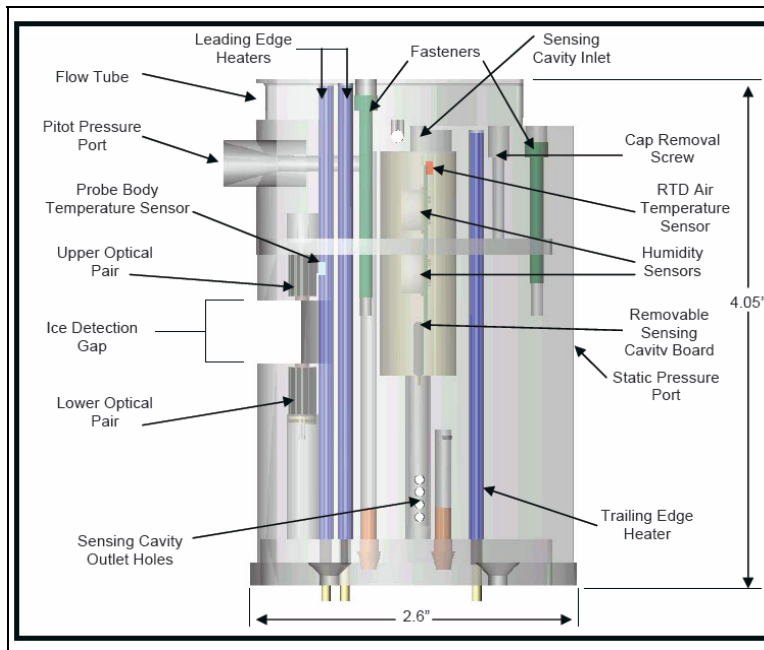
Figure 59. TAMDAR sensor head that senses a variety of atmospheric conditions. Ice sensing is accomplished by light beam interruption in the leading edge notch.
