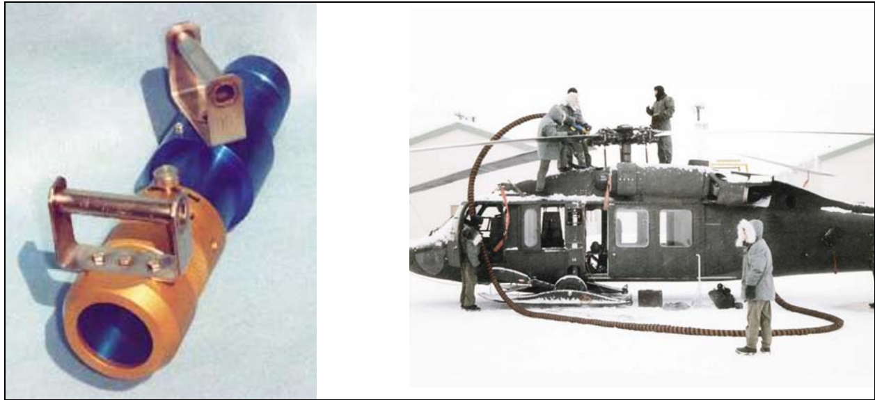
Figure 36. Buddy Start deicing nozzle (left) and system in use on Black Hawk helicopter (right).
