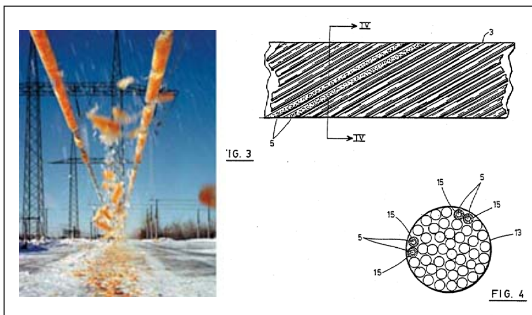
Figure 54. Electro-expulsive deicing technology applied to cables. Image on left shows colored ice falling from cables immediately after system activation.
