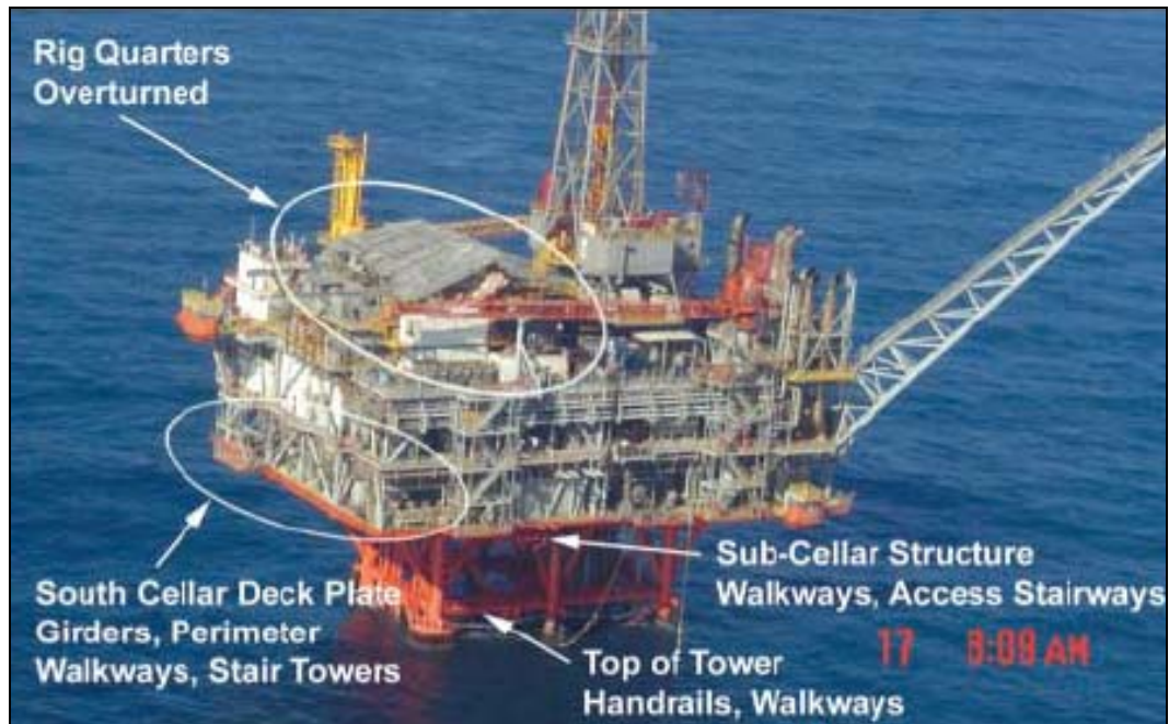
Figure 9. Complex cellar deck on the rig Petronius that would ice readily if located in colder waters.
