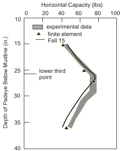
Fig. 9 Comparison of Measured Horizontal Capacity with Theoretical Solutions
