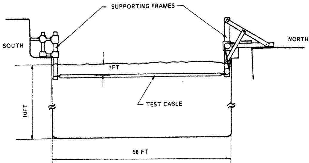
Figure 1 - Cable Deployment
