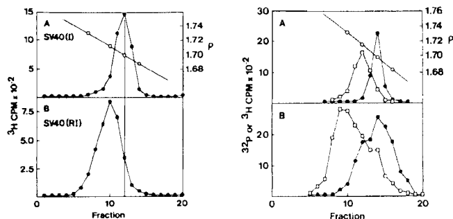
FIG. 11 (left). CsCl density gradient centrifugation of SV40 DNA synthesized in the presence of BrdUTP. Lysates from SV40-infected cells were exposed to ^3\text{H} thymidine for either 1 hour to label SV40(I) DNA (A) or 4 min to label SV40(RI) (B) and then incubated with BrdUTP in the absence of dTTP. \bullet — \bullet , ^3\text{H} ; \circ — \circ , density.
