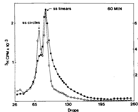
FIG. 9 (top). Isolation of covalently closed viral DNA labeled during in vitro synthesis. Procedure was the same as described in Fig. 8 except sedimentation was in an alkaline sucrose gradient. \circ — \circ , ^3\text{H} ; \bullet — \bullet , ^{32}\text{P} ; I, SV40(I) DNA; II, SV40(II) DNA. Covalently closed dimers appear in Fractions 6 to 7. The gradient was centrifuged for 2 hours as in Fig. 3.
