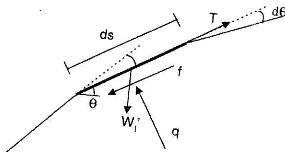
Figure A-1. Soil stresses at an anchor line segment in soil
