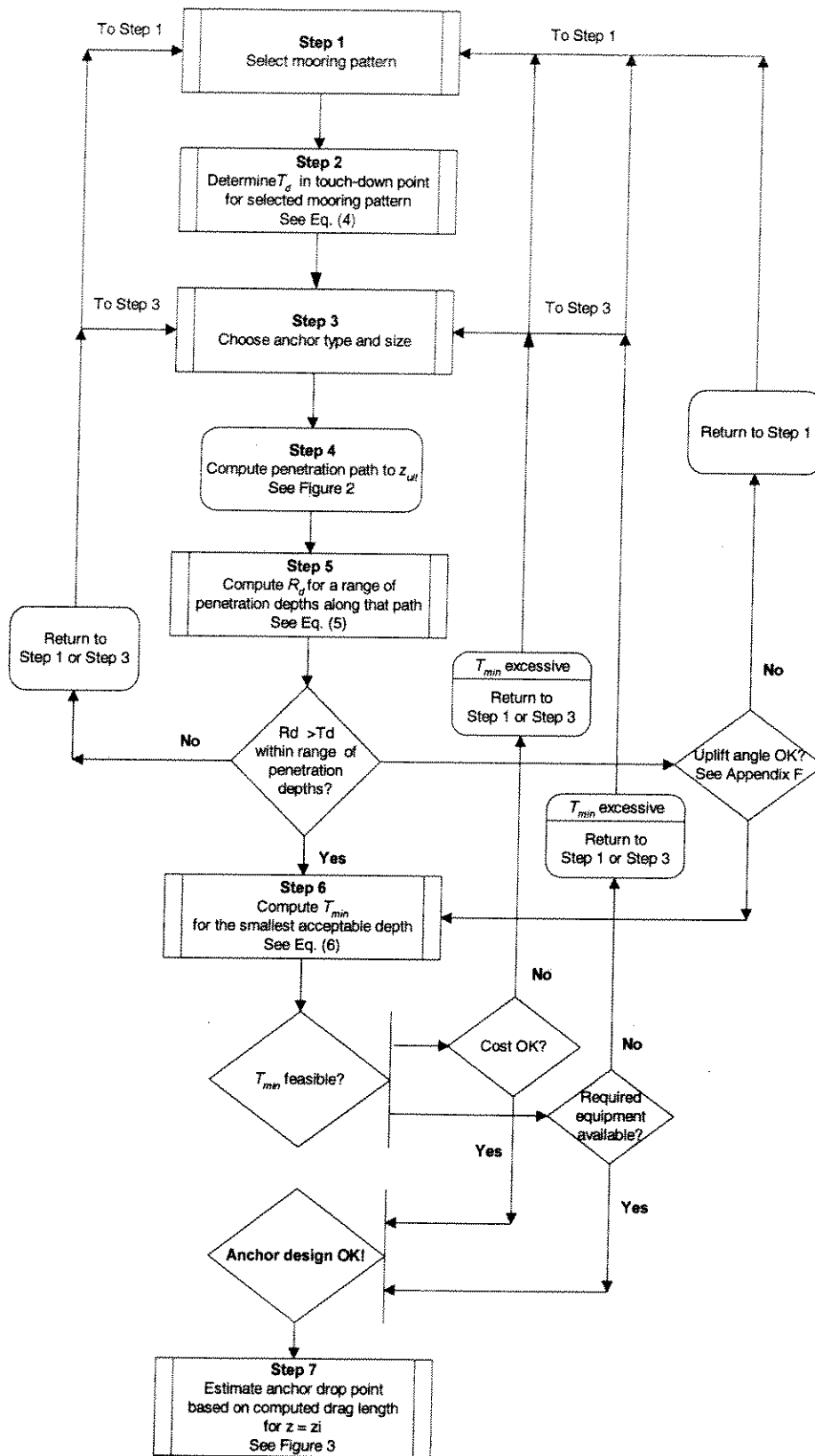
Figure 4 Design procedure - flowchart.
