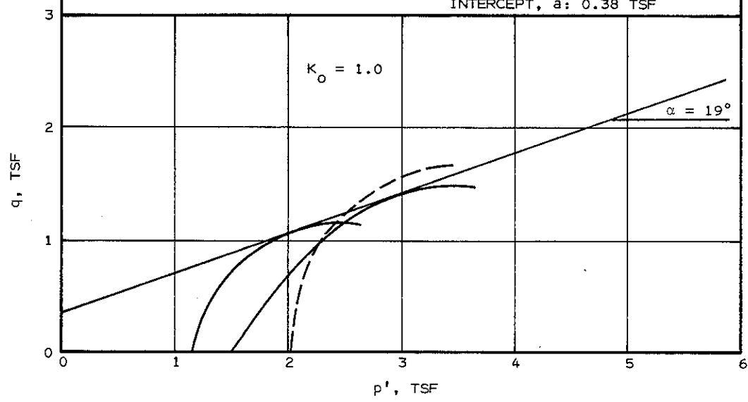
TRIAxIAL TEST RESULTS REMOLDED ANISOTROPIC CONSOLIDATED UNDRAINED
