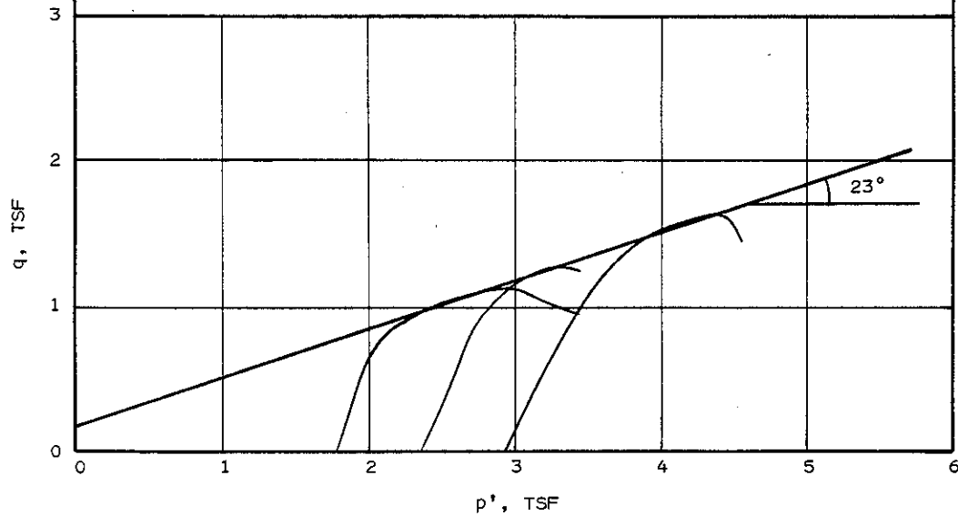
TRIAxIAL TEST RESULTS REMOLDED CONSOLIDATED UNDRAINED
