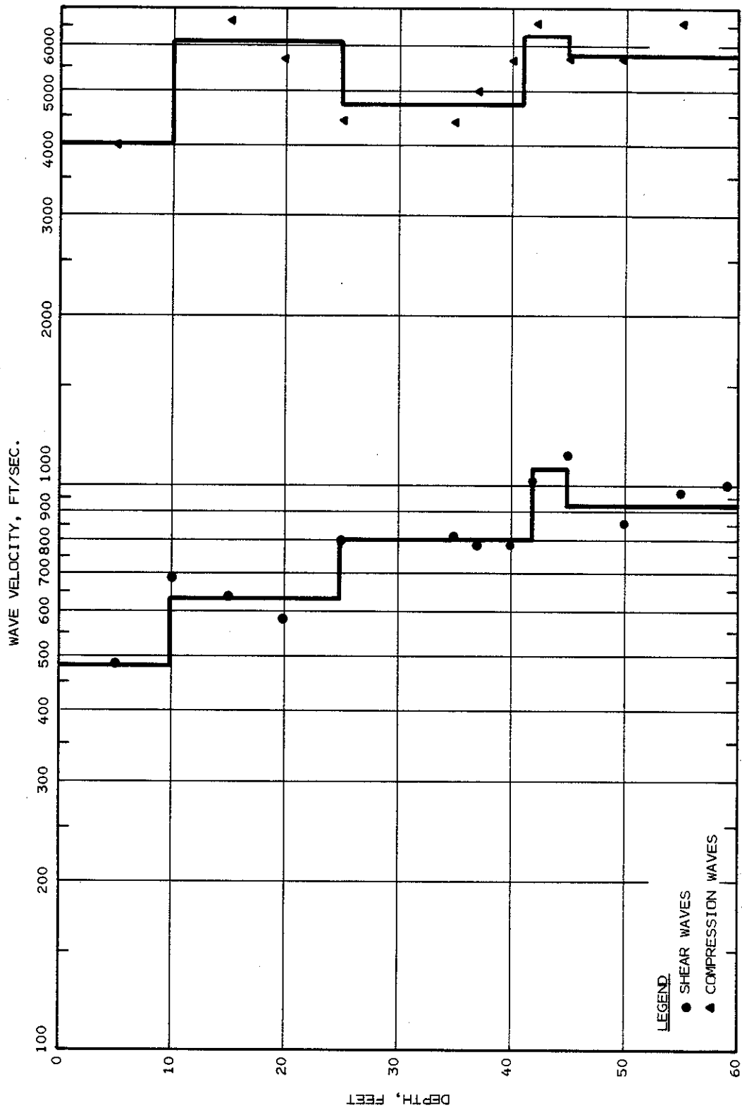
FIGURE C39. SHEAR AND COMPRESSION WAVE VELOCITY PROFILE FROM CROSS-HOLE SEISMIC TESTS
