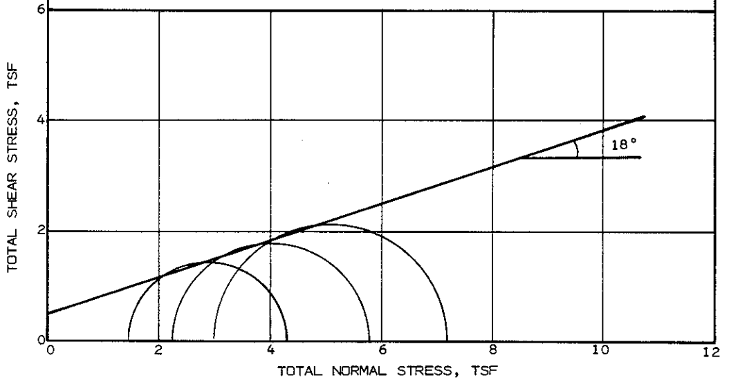
CIU TRIAXIAL TEST RESULTS REMOLDED
