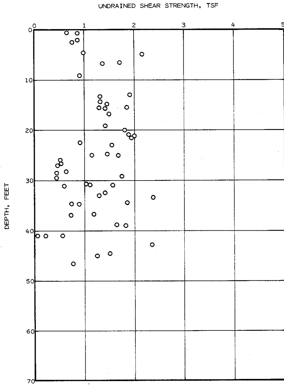
FIGURE C19. UNDRAINED SHEAR STRENGTH TORVANE VALUES
