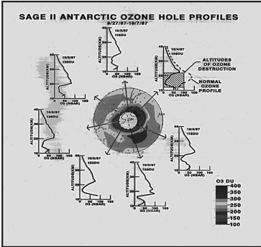
Fig. 2. The small plots around the center figure represent the vertical distribution of ozone, from SAGE II data, at various locations in the Antarctic region. The vertical profiles show at which levels the greatest depletion of ozone is occurring. The central figure is from another satellite (TOMS) which measures how much ozone is in the whole atmosphere directly below the satellite. By using SAGE II data, scientists were able to pinpoint where the greatest ozone depletion was occurring and better determine the causes of the Antarctic ozone hole.
