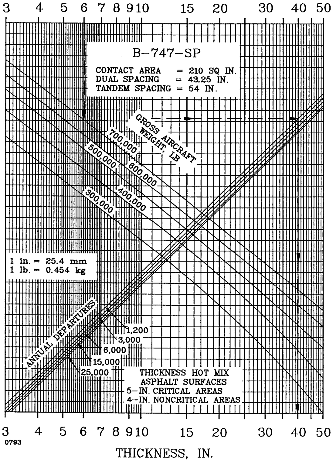
FIGURE 3-8 FLEXIBLE PAVEMENT DESIGN CURVES, B-747-SP
