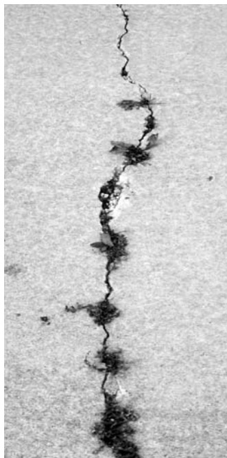
◀◀ Slab crack with spalling and debris.
