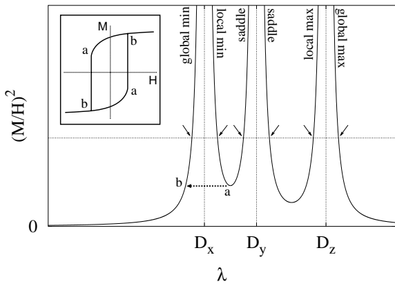
Fig. 1. Plot of g(\lambda) . D_x < D_y < D_z . h_\nu \neq 0, \nu = x, y, z
