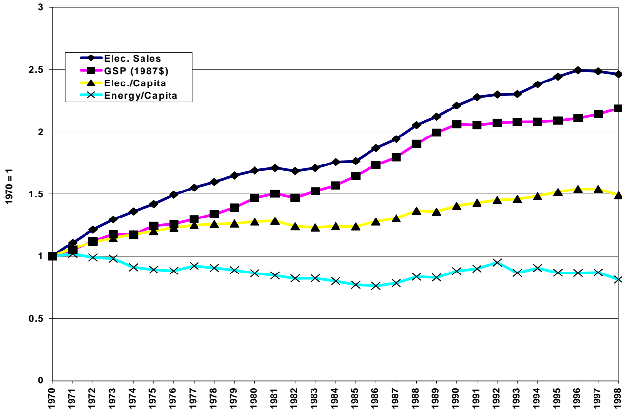
Figure 2. Key Energy and Economic Indicators in Hawai'i, 1970 to 1998
