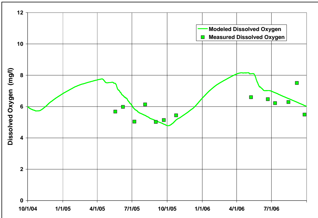
Figure B-6: Simulated versus Measured Hypolimnetic Oxygen - Grand Lake
