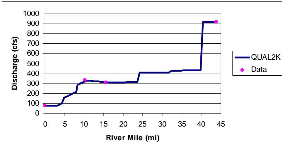
Figure 4. Comparison of model output with measured data for discharge.
