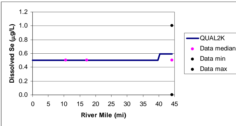
Figure 13. Comparison of model output with measured data for dissolved selenium.
