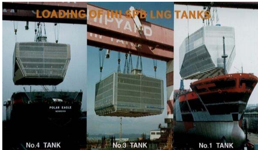
Figure 2. Prismatic Tanker Ship
