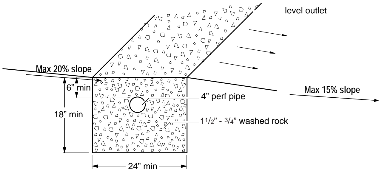
FIGURE 3.2.3.2.C 10-FOOT DISPERSION TRENCH CROSS-SECTION AND ROOF APPLICATION
