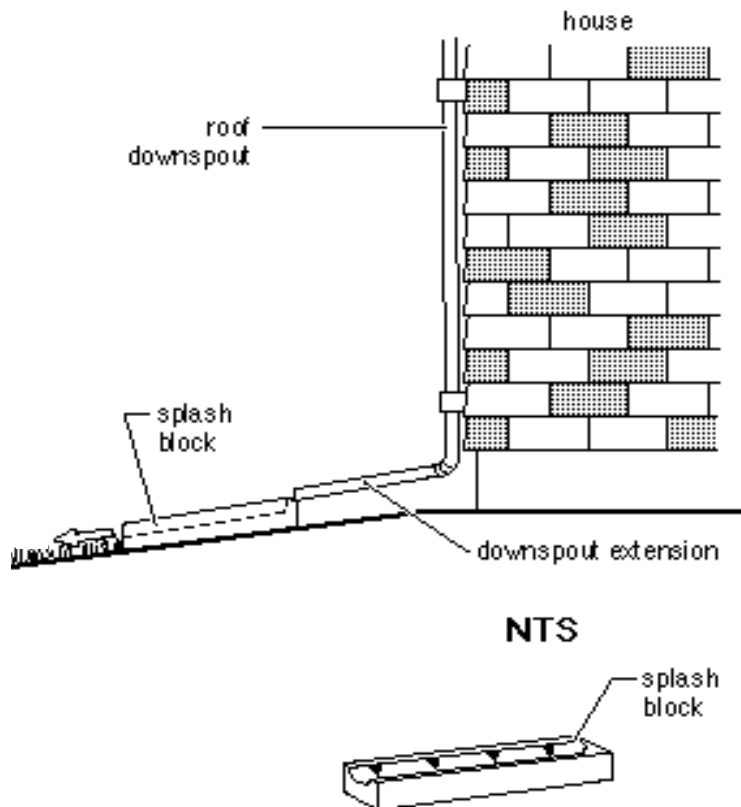
FIGURE 3.2.3.2.A TYPICAL SPLASH BLOCK
