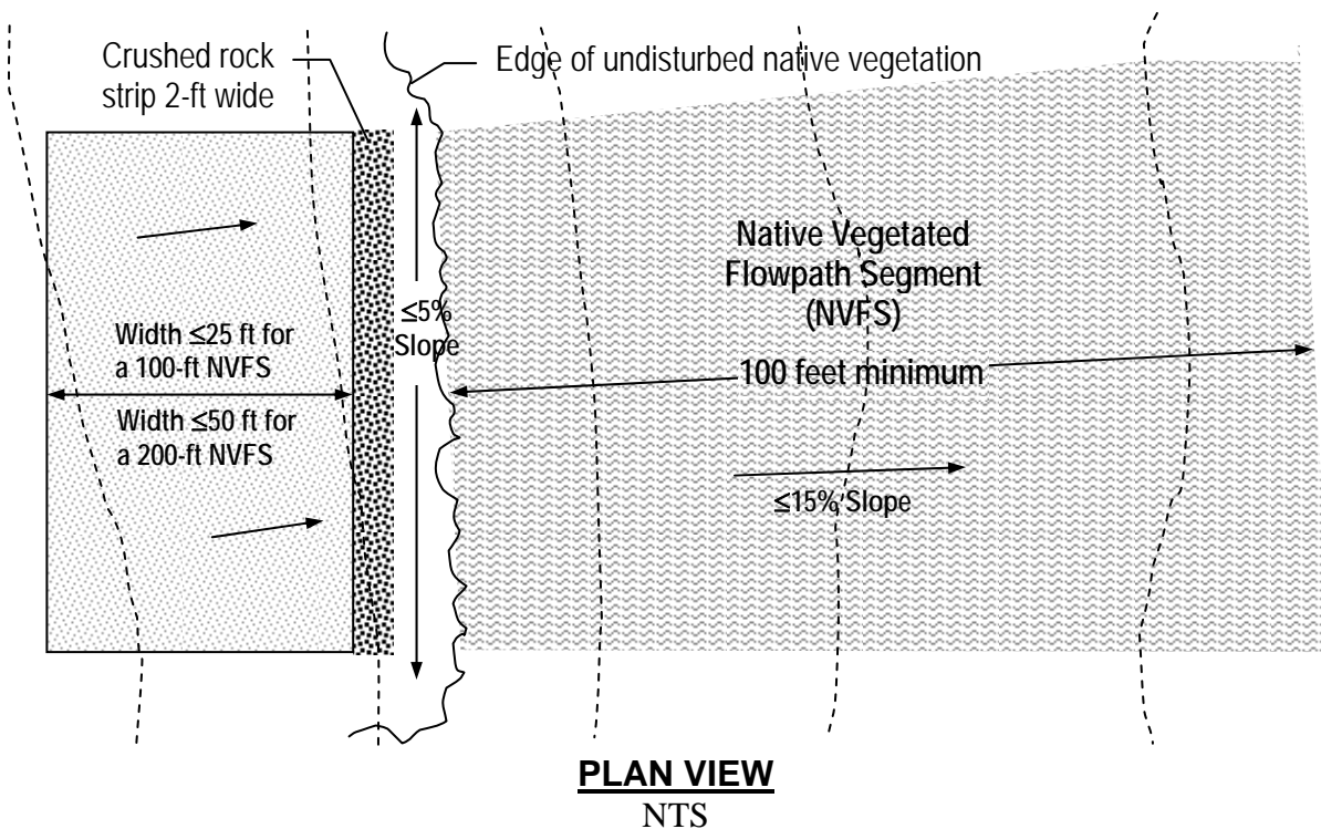
FIGURE 3.2.3.2.E APPLICATION OF SHEET FLOW DISPERSION
