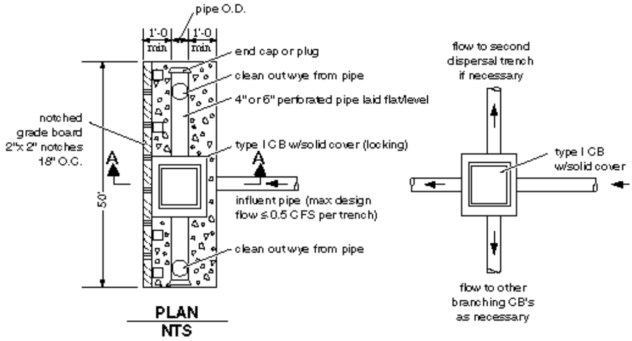
FIGURE 3.2.3.2.D 50-FOOT DISPERSION TRENCH WITH NOTCHED BOARD
