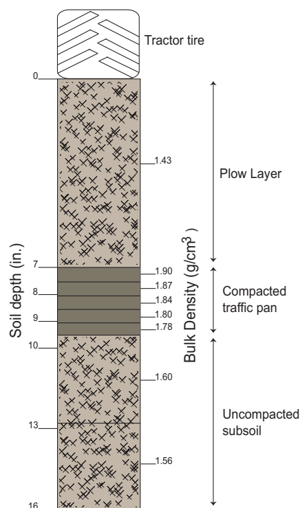
Figure 1. Tillage and heavy equipment traffic compacted soil below the plow layer of an Udult soil (Norfolk), inhibiting root penetration and water movement through the soil profile.
