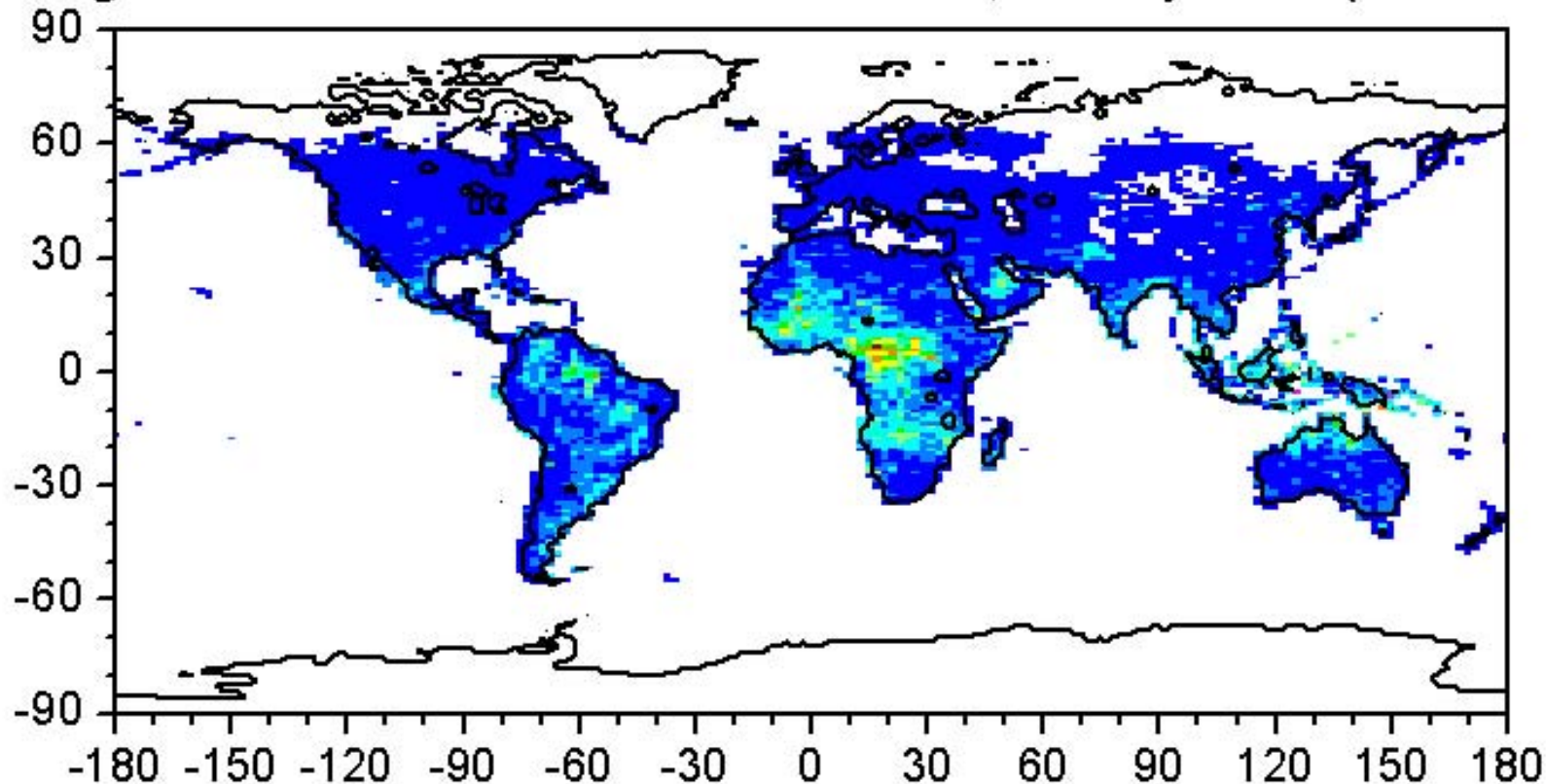
Orig-Corrected SW TOA Flux Difference; All-Sky Land (Dec 2001)
