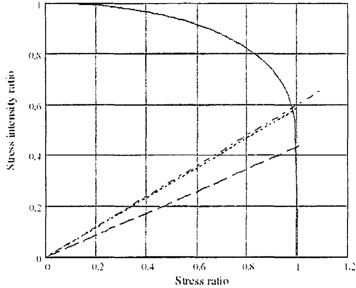
Figure 1. Failure assessment diagram for Ti-7 (compact specimen)
