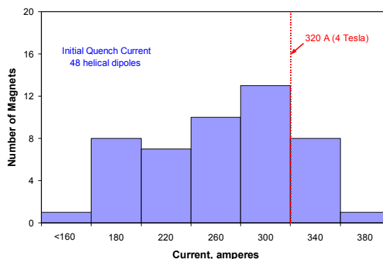
Figure 2: Distribution of initial quench currents.
