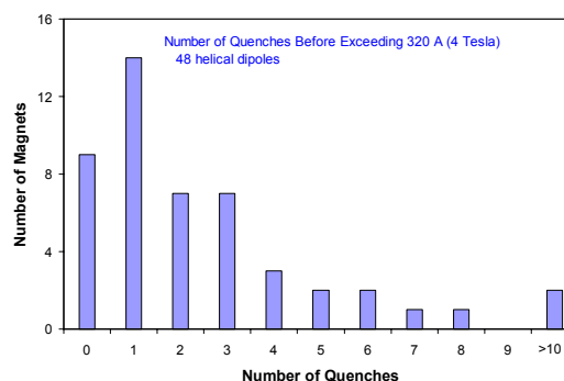
Figure 3: Number of required quenches.
