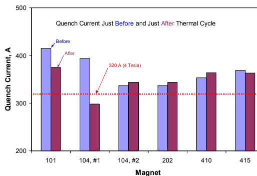
Figure 4: Retraining after thermal cycle.
