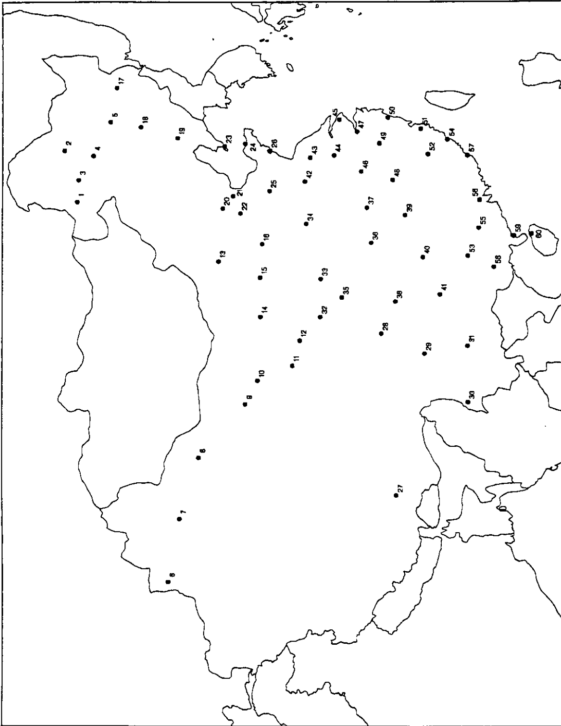
Fig. 7. Distribution of stations from the PRC 60-station climate data set over the period 1951–1988. Station numbers correspond to the order of stations in Table 3.
