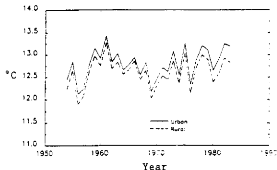
Fig. 2: The annual mean temperatures averaged over the urban and rural stations shown in Figure 1. The mean temperatures for rural and urban stations averaged over 1954-1983 are 12.61^{\circ}\text{C} and 12.80^{\circ}\text{C} , respectively.
