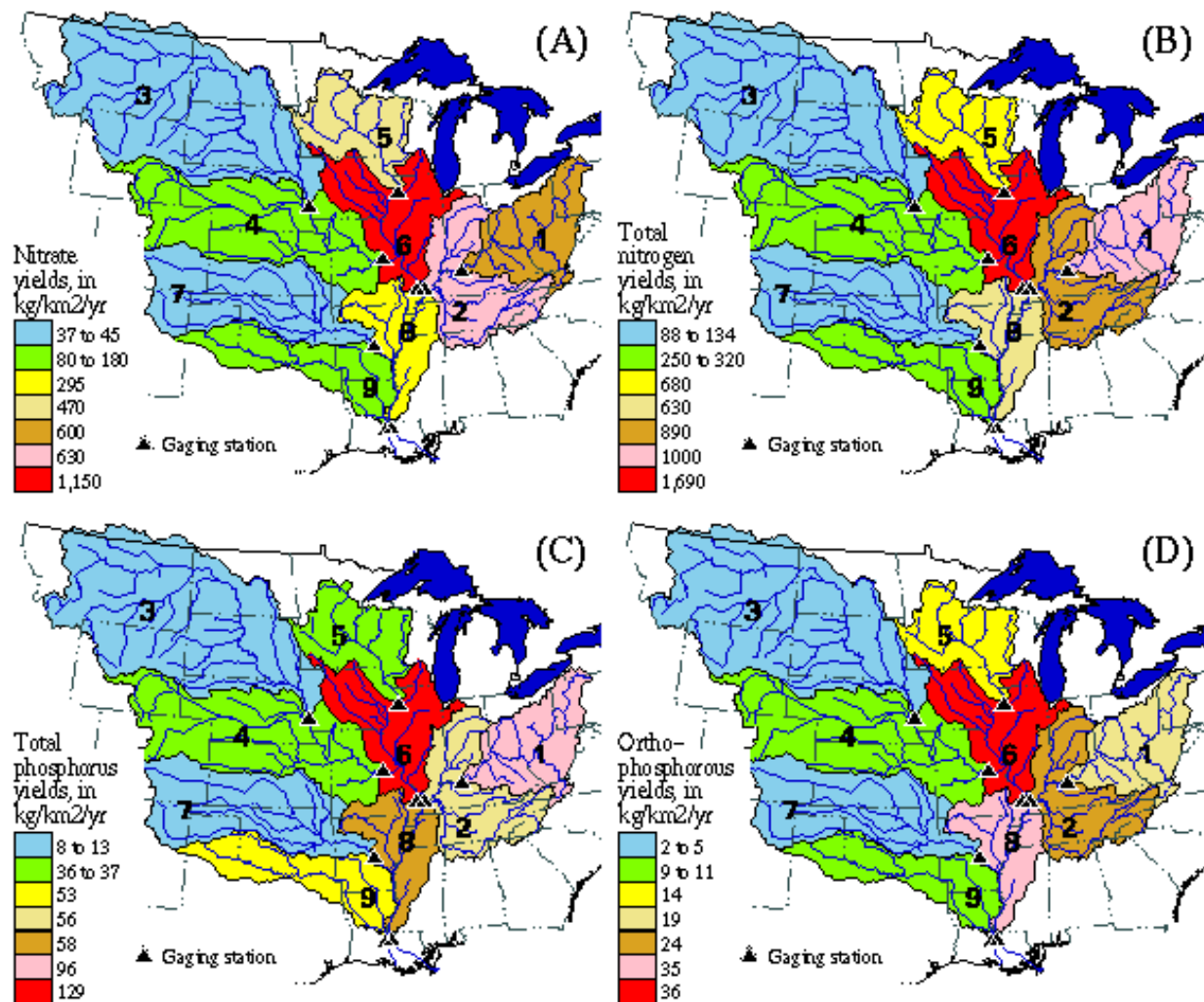
Figure 5. Yields of nitrogen and phosphorus contributing to Hypoxia in the Gulf of Mexico (Goolsby et al., 1999)
