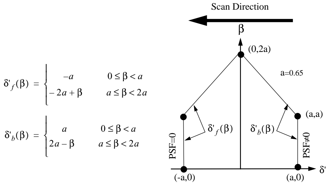
Figure 8-3. Optical FOV
