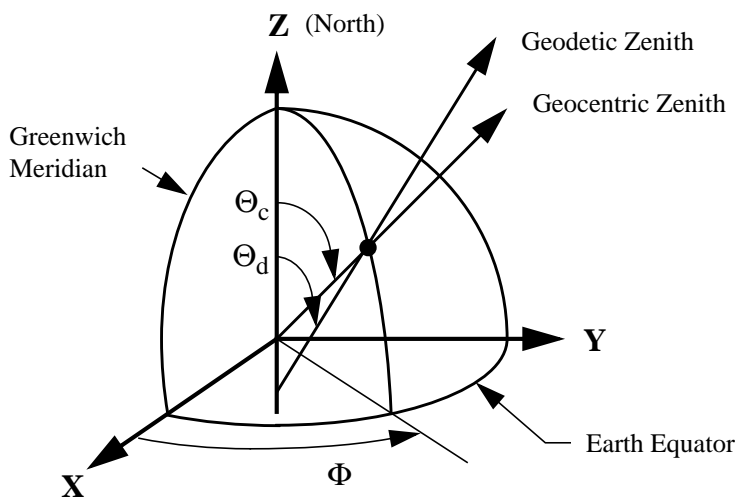
Figure 4-1. Geocentric and Geodetic Colatitude/Longitude
