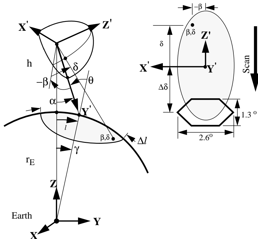
Figure 8-2. Scanner Footprint
