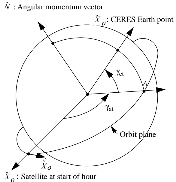
Figure 4-4. Along-track Angle
