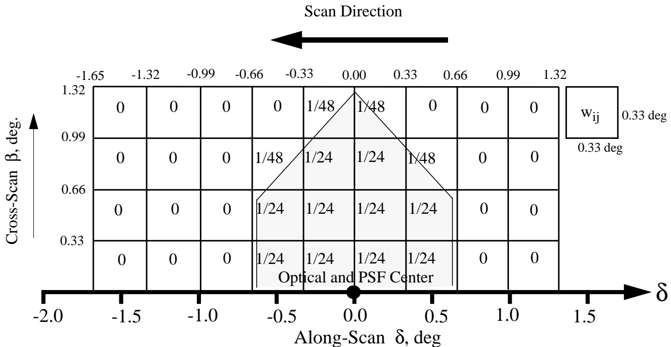
Figure 8-5. Static PSF and Field-of-View
