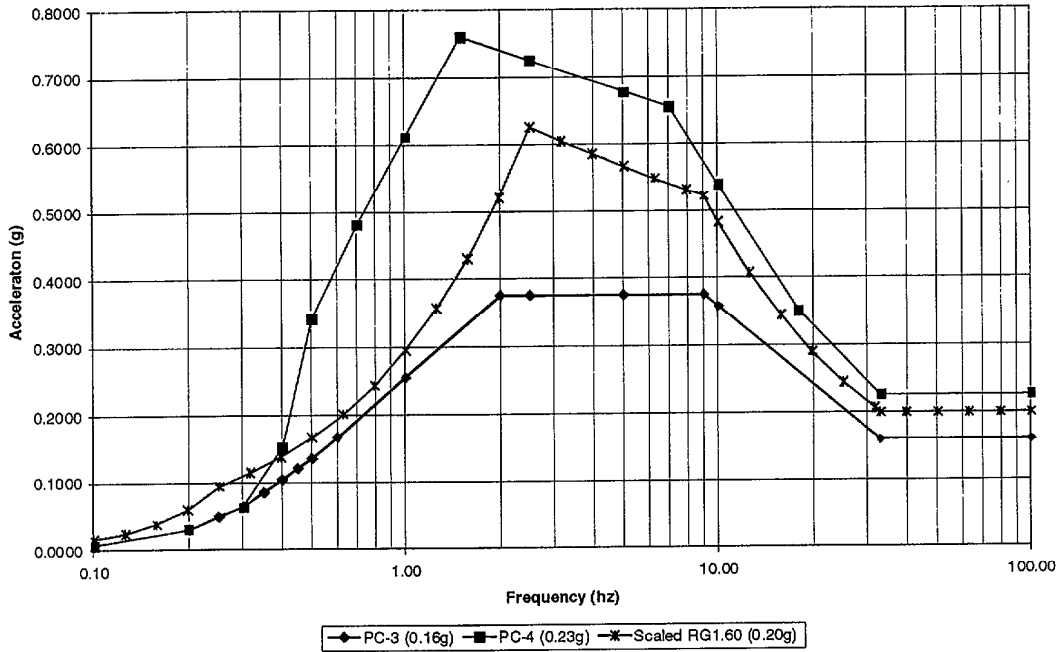
SRS Response Spectra (Horizontal 5% Damping)
