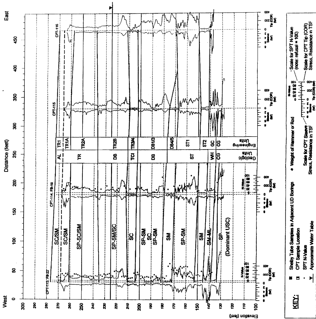
Figure 5-11. Geologic Cross Section 4 (WSRC 1999a) Page 112 of 198
