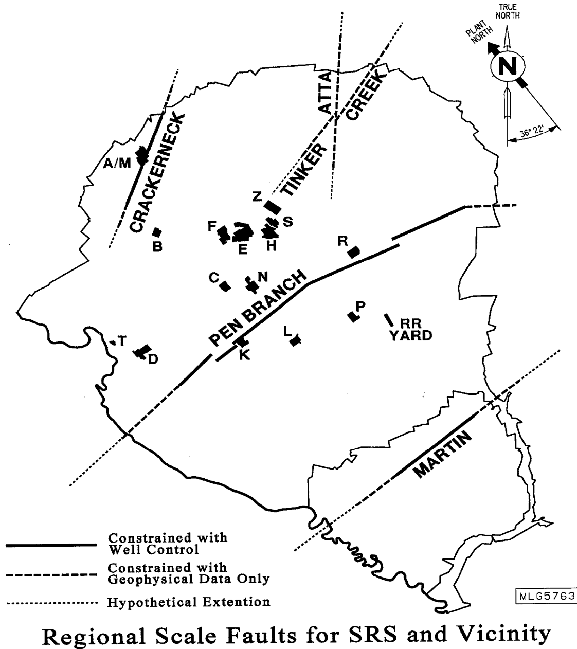
Figure 3-4. Regional Scale Faults for SRS and Vicinity (WSRS 2000a).
