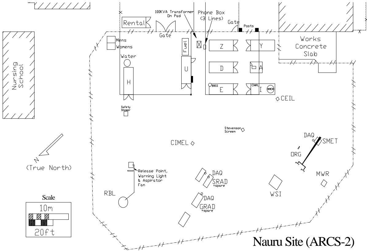
Figure 9. The Nauru site layout.
