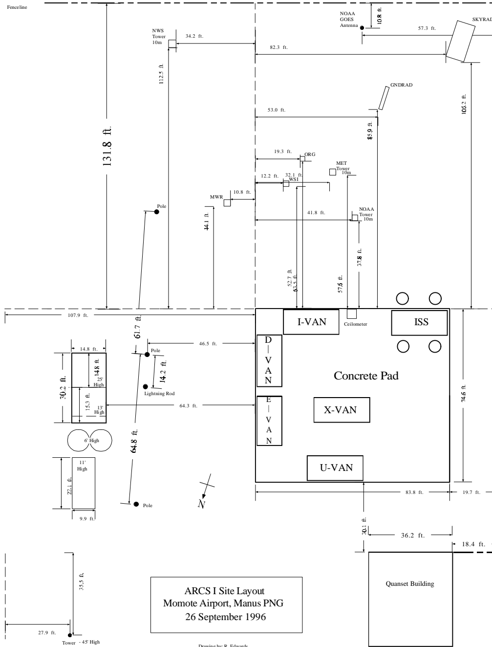
Figure 5. Manus site layout.
